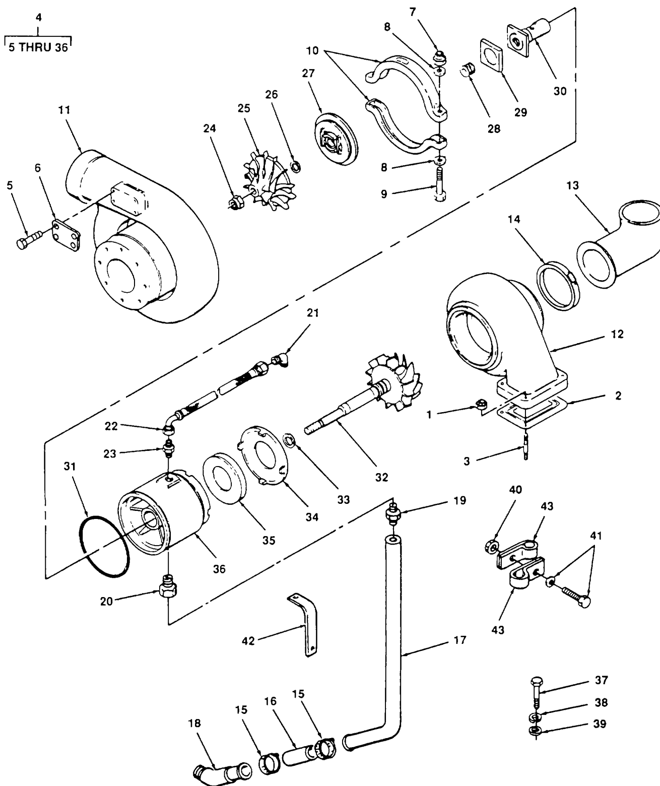
Figure 104. Turbocharger Assembly.
