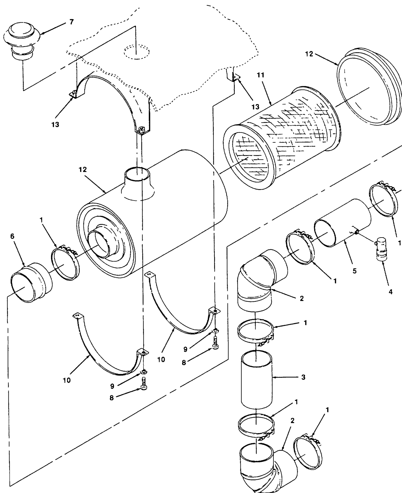
Figure 103. Air Cleaner
