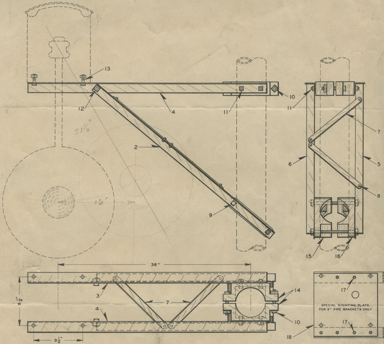
PARTS FOR No. 1731-5 IRON OFFSET BRACKET TO FIT 5" STANDARD PIPE 5-9/16" O.D.
