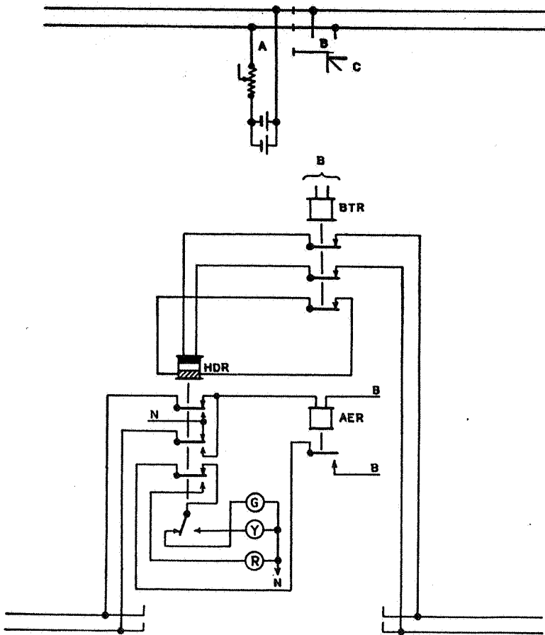
Fig. 24. Typical Local Wiring—Color Light Signal.
