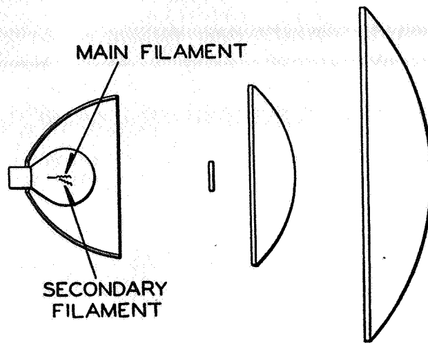
Fig. 33. Diagram Showing Positioning of Filaments in a Searchlight Signal Unit.
