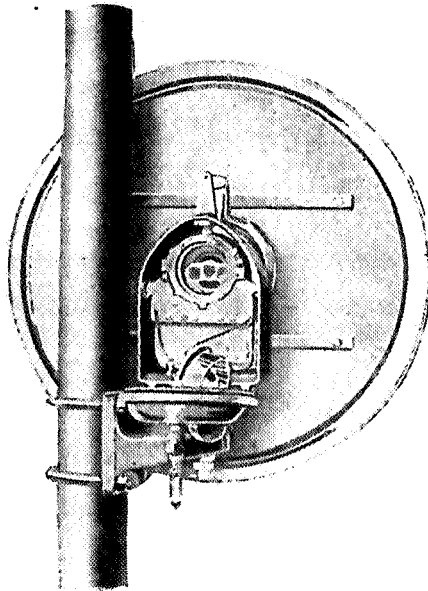
Fig. 12. Color Light Signal, Searchlight Type.
