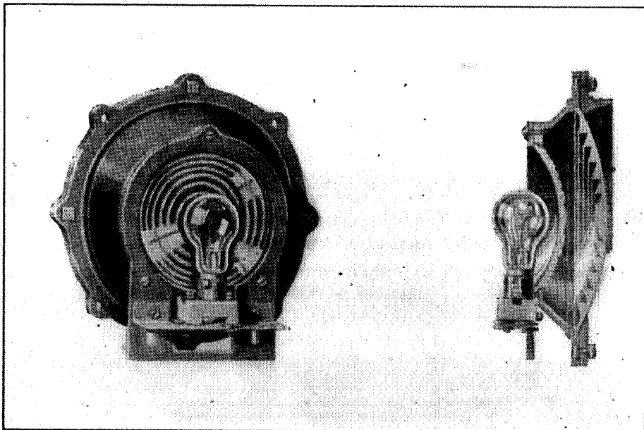
Fig. 3. Doublet Lens Unit.
