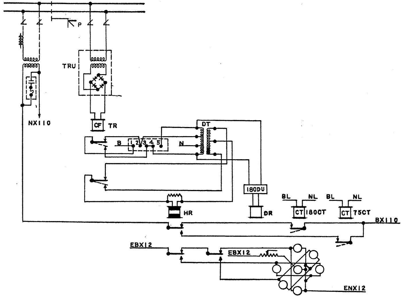
Fig. 26. Typical Local Wiring—Position Light Signal.
