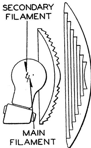
Fig. 32. Diagram Showing Positioning of Filaments in a Lensing Unit Having No Reflector.
