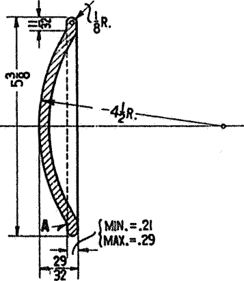
5 3 / 8 CONVEX ROUNDEL HIGH TRANSMISSION GLASS
