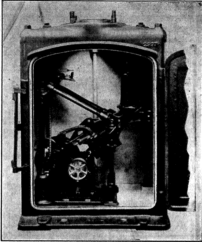
Fig. 3. Electric Motor Signal, Base-of-Mast Mechanism.
