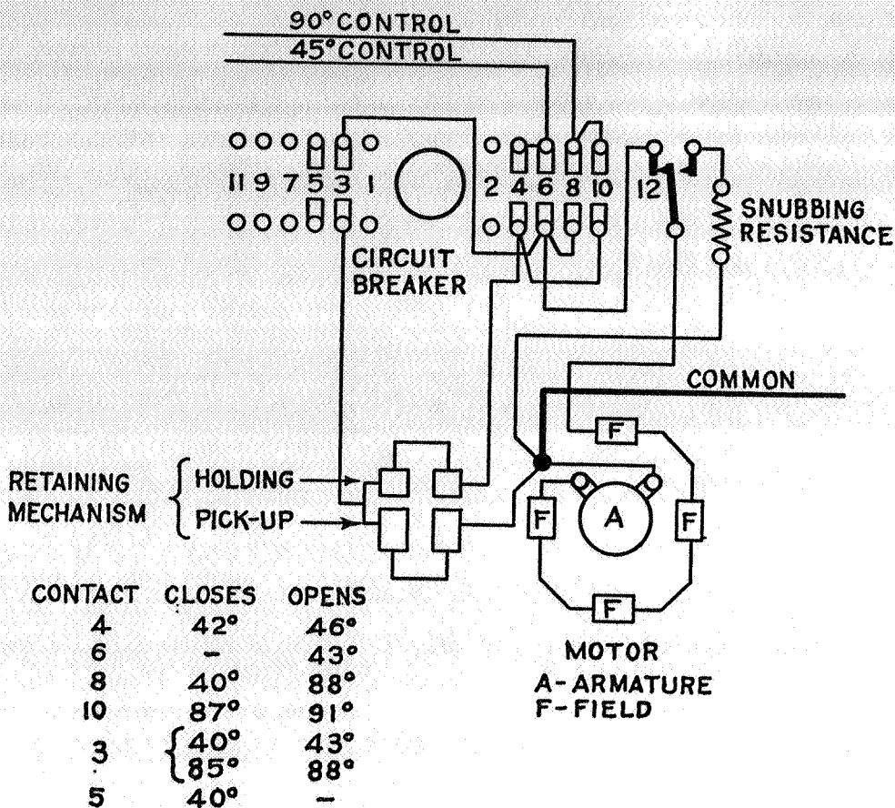
Fig. 21. Mechanism Wiring, Model 2-A Signal.
