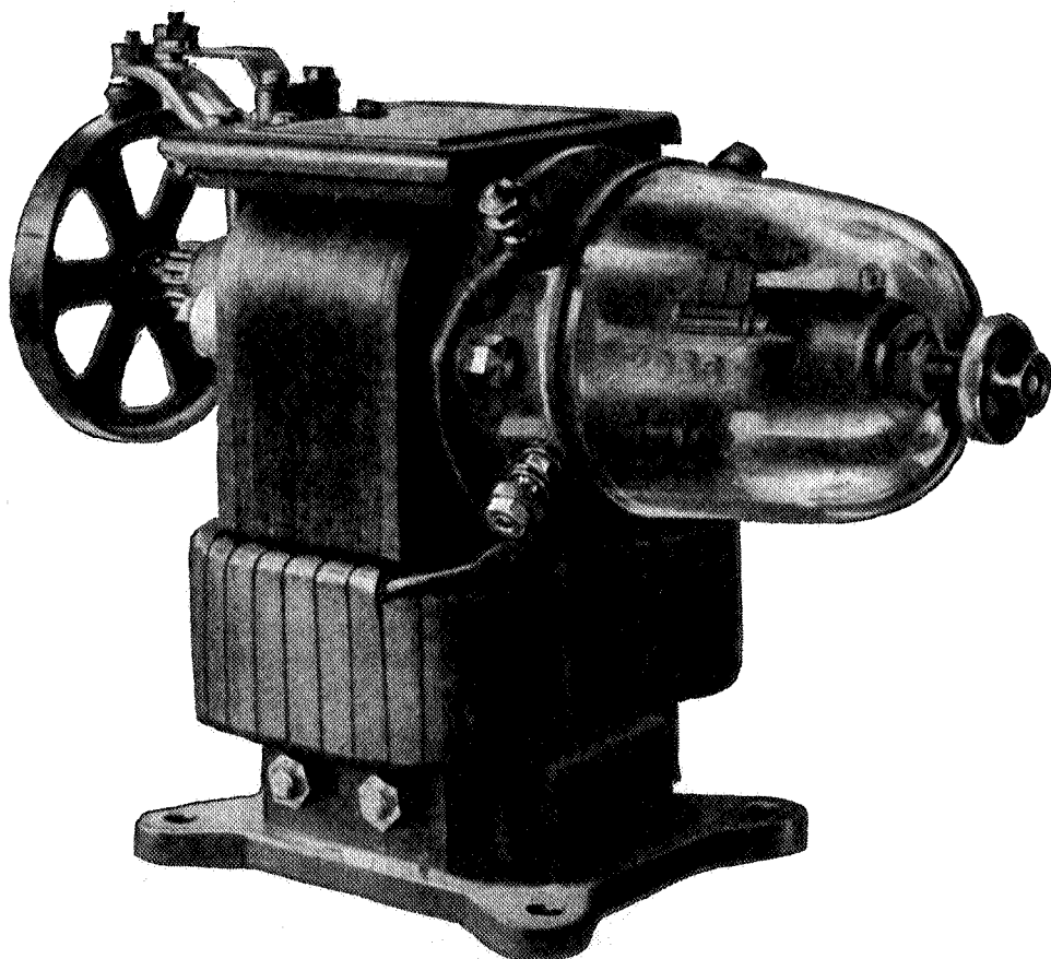
Fig. 8. Direct Current Motor for Style B Mechanism.
