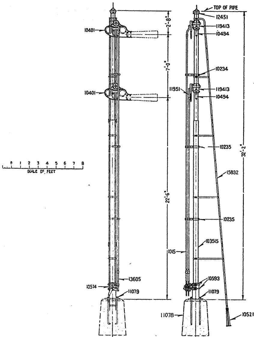
TWO-ARM MECHANICAL GROUND SIGNAL
