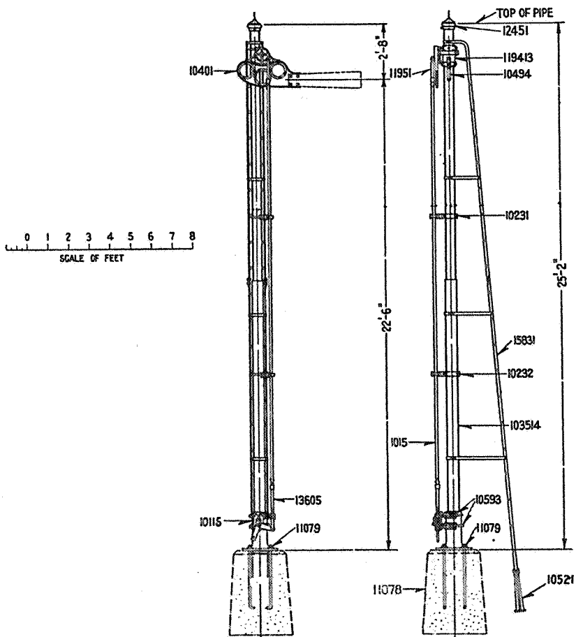
ONE-ARM MECHANICAL GROUND SIGNAL
