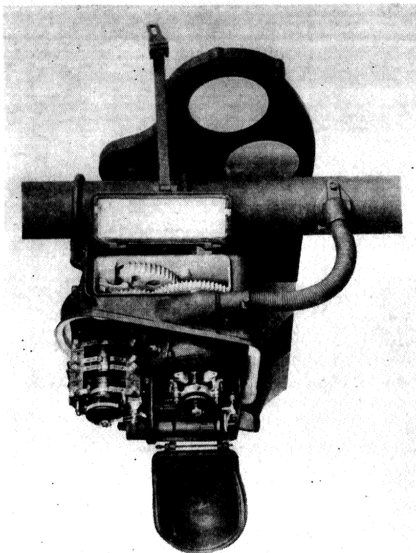
Fig. 4. Electric Motor Signal, Top-of-Mast Mechanism.
