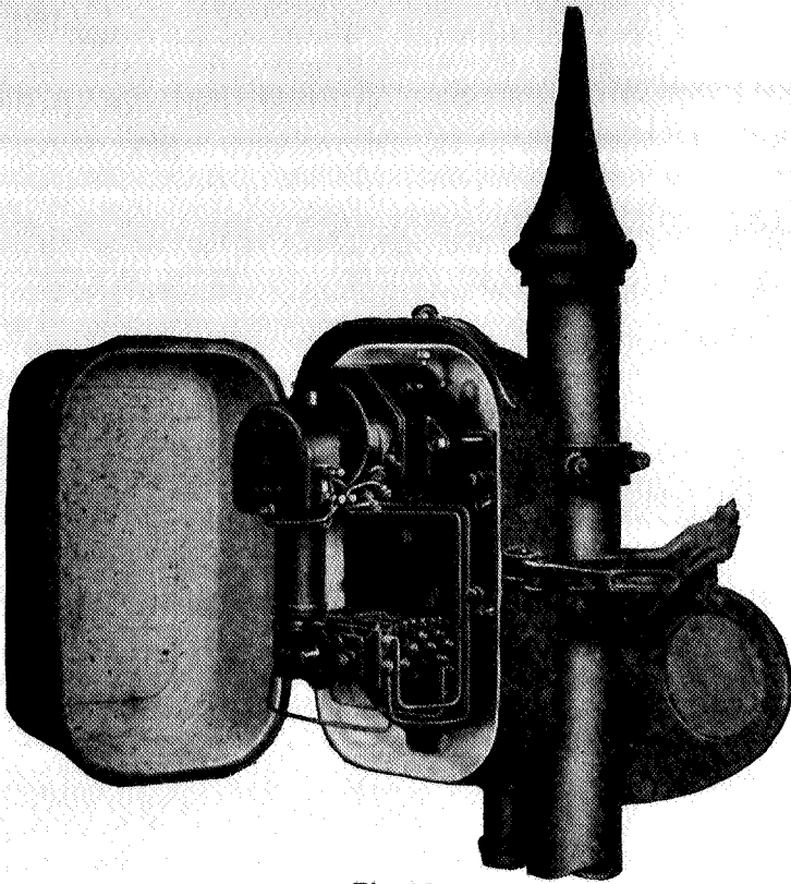
Fig. 16. Style T-2 Direct Current Signal Mechanism.
