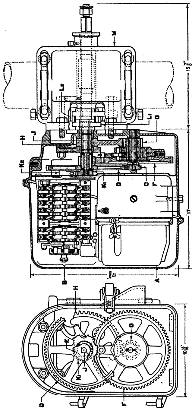
Fig. 12. Model 2-A Direct Current Signal Mechanism.
