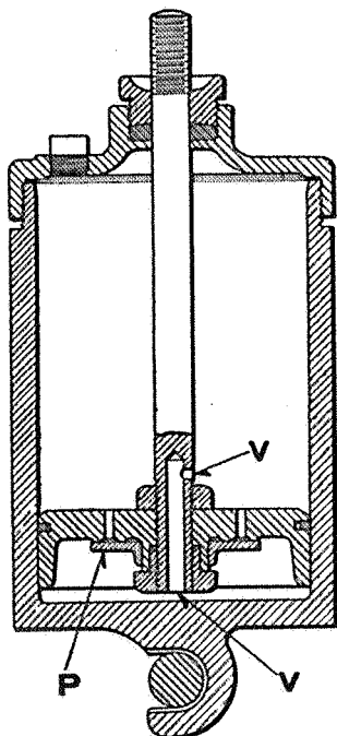
Fig. 9. Oil Buffer, Style S Mechanism.
