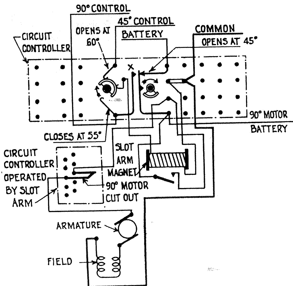
Fig. 20. Mechanism Wiring, Style S Signal.
