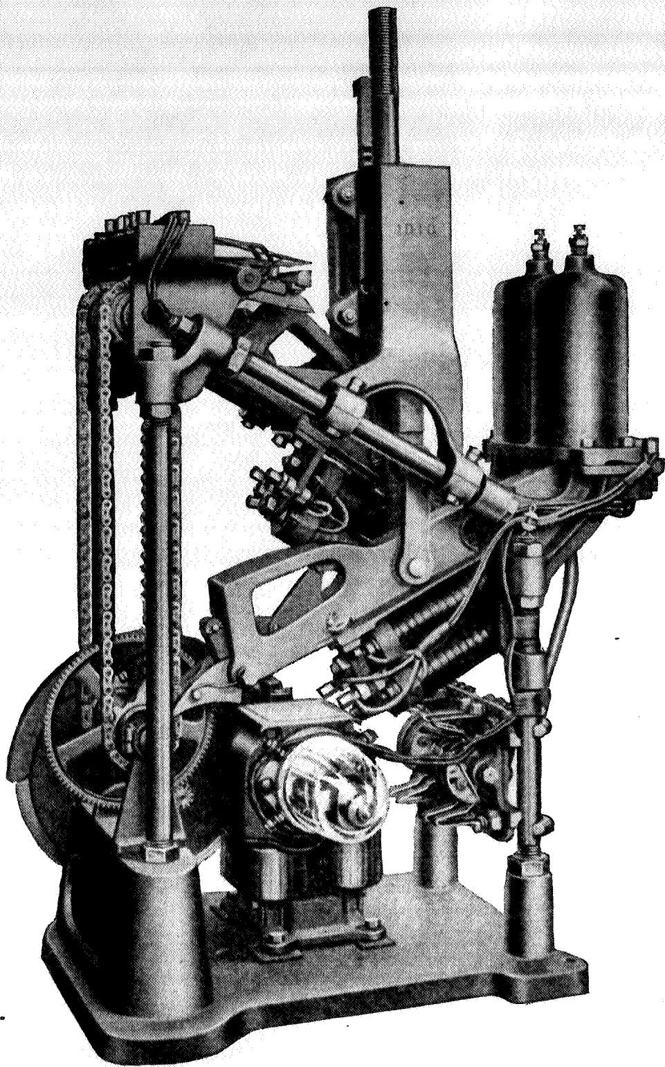
Fig. 7. One-Arm Three-Position Style B Signal Mechanism.
