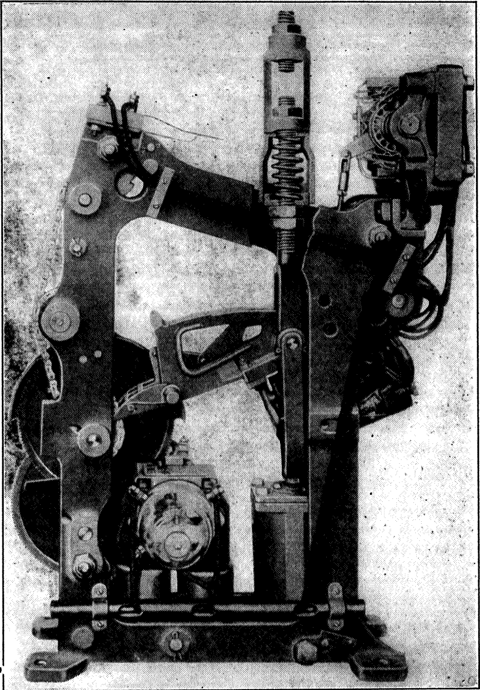
Fig. 11. Style S Base-of-Mast Mechanism.
