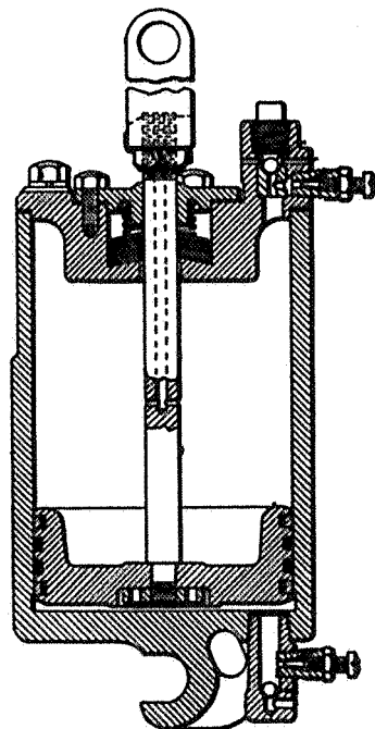
Fig. 10. Air Buffer, Style S Mechanism.
