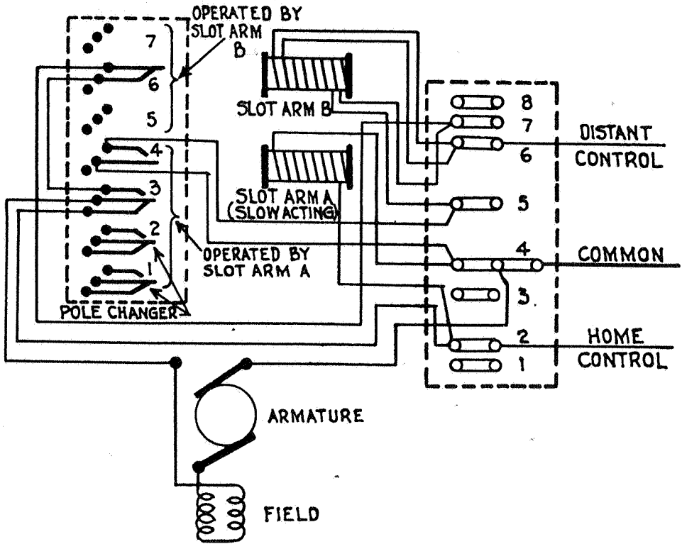
Fig. 19. Mechanism Wiring, Style B Signal.
