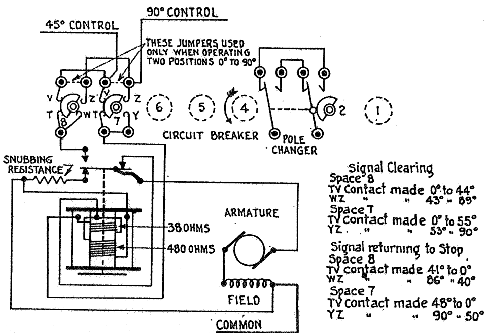
Fig. 22. Mechanism Wiring, Style T-2 Signal.
