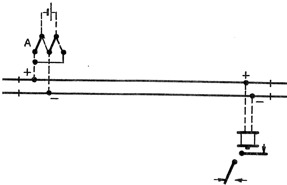
Fig. 10. Polarized Track Circuit.
