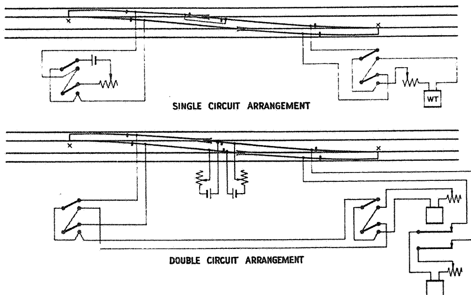
Fig. 6. Crossovers with Independent Track Circuits.
