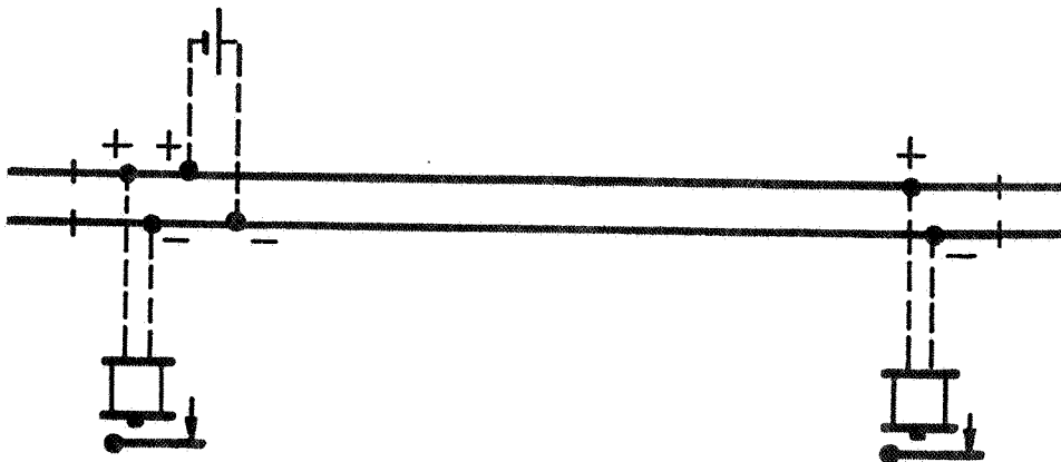
Fig. 9. End Fed Track Circuit and Two Relays.
