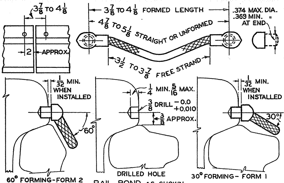
60° FORMING-FORM 2
