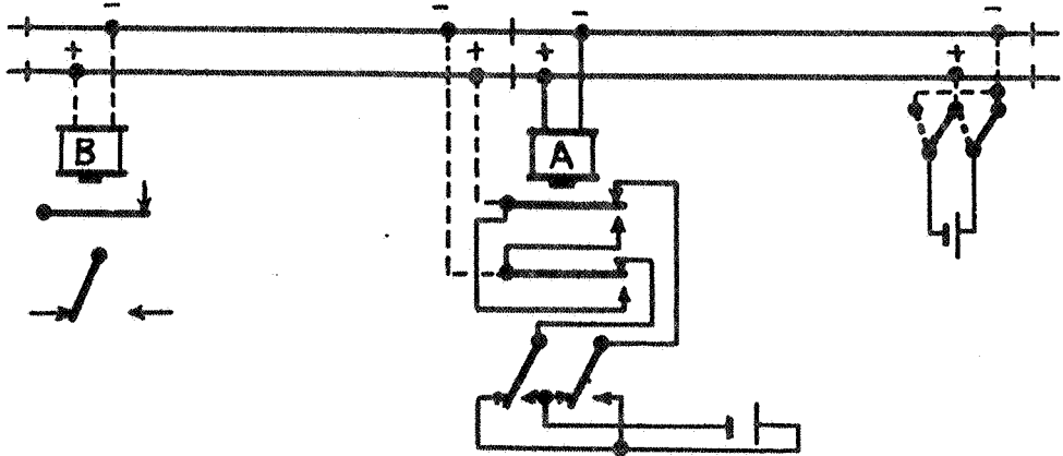
Fig. 13. Polarized Cut-Sections.
