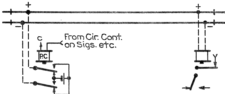
Fig. 11. Polarized Track Circuit, Using Pole Changing Relay.
