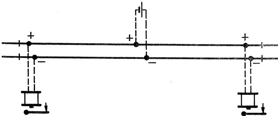
Fig. 8. Center Fed Track Circuit.
