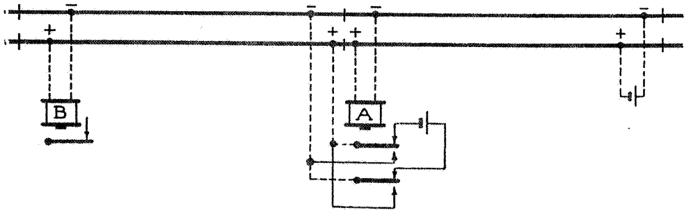
Fig. 12. Neutral Cut-Sections.
