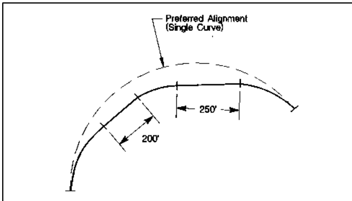
Figure 3-1. Combining Curves
