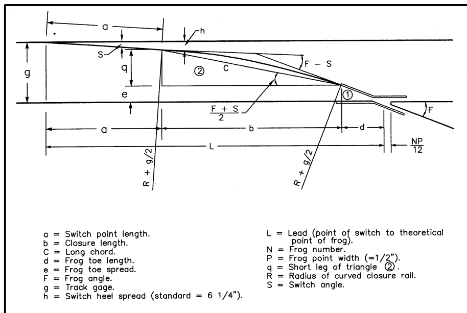
Figure 6-28. Turnout Design
