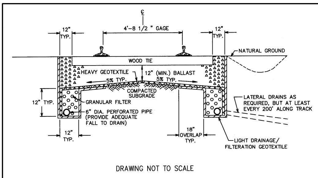
Figure 6-17. Required Subdrainage where Open Side Ditches cannot be Installed
