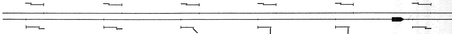
Fig. 7. Aspects Displayed in a Two-Block Indication System, Double Track, with One Block Overlap.
