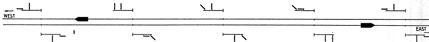
Fig. 5. Aspects Displayed in Three-Block Indication System, Double Track.
