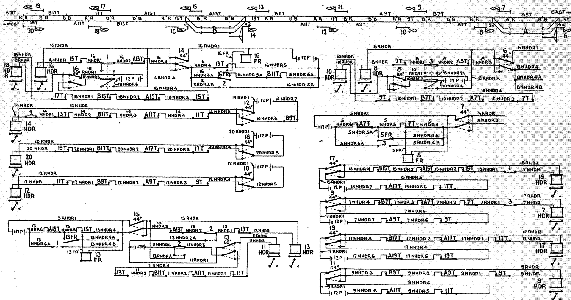
Fig. 10. Circuits for Single-Track Overlap Two-Block Indication Three-Position Semaphore Signals, Normal Clear, with Direct Current Neutral Track and Polarized Line Control Circuits.
