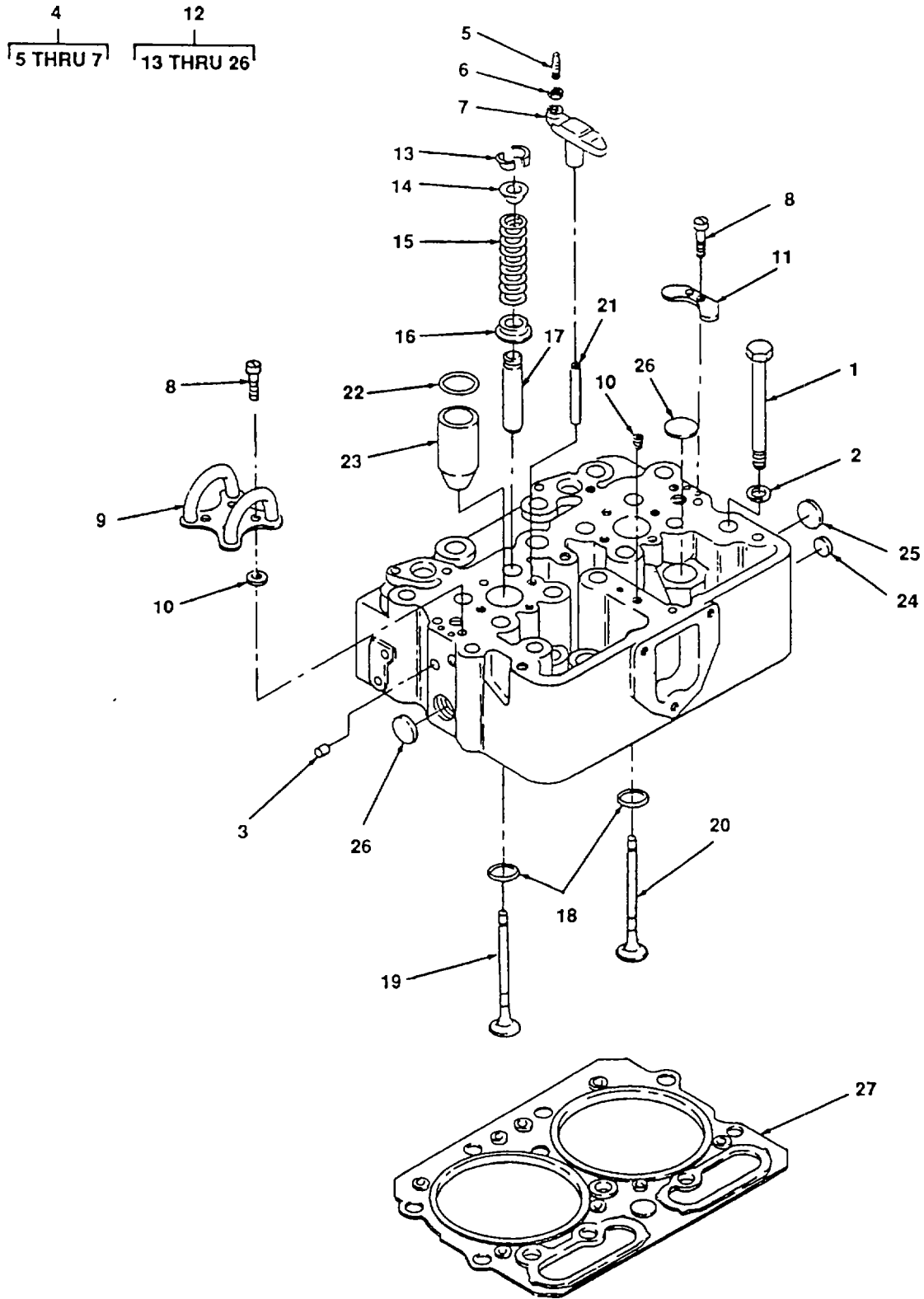
Figure 124. Cylinder Head Assembly
