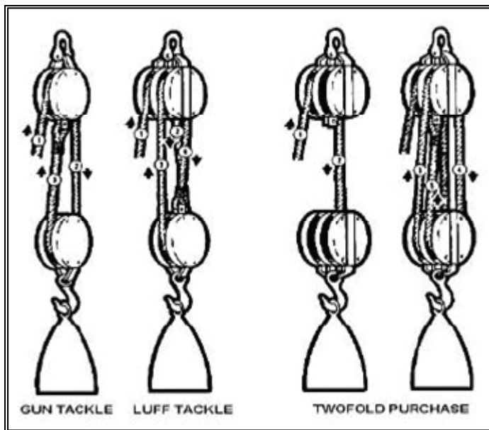
Figure 6-6. Reeving Tackles
