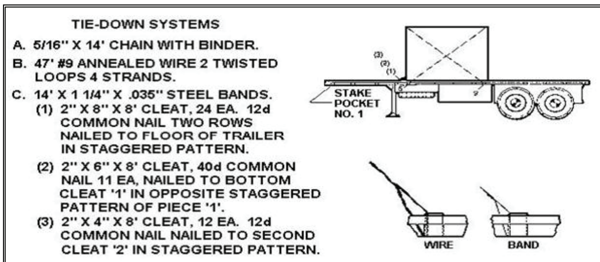
Figure 19-3. Recommended Tie-Down for CONEX on M127 Semitrailer
