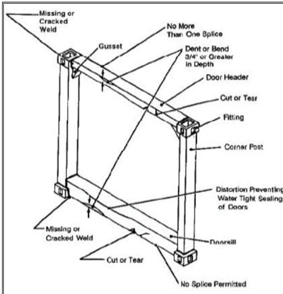
Figure 15-3. Defects of Rear End Frame Causing Container Rejection
