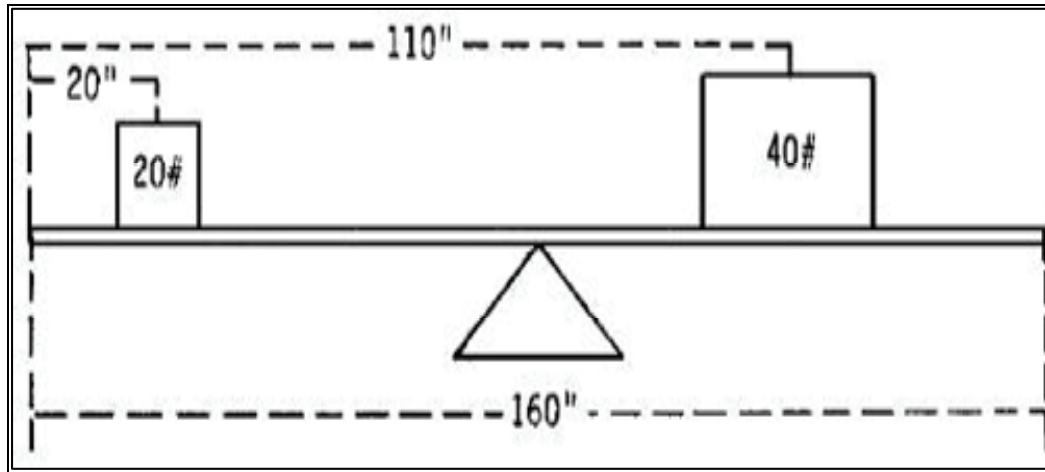
Figure 17-5. Computing Aircraft and Load CG
