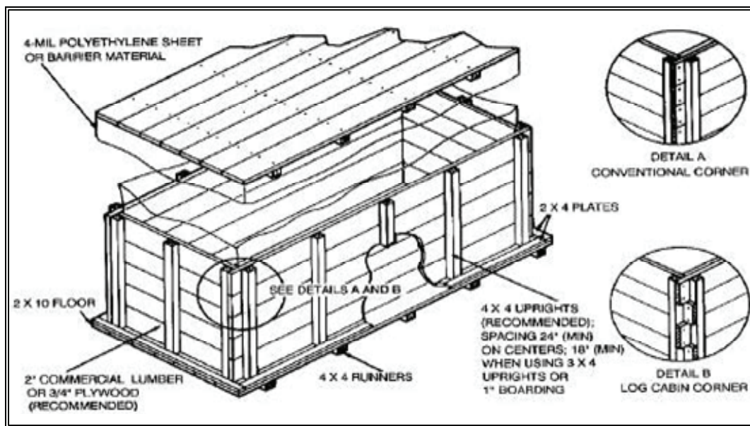
Figure 9-38. Portable Class A Magazines
