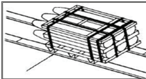
Figure 9-14. Strip Decking
