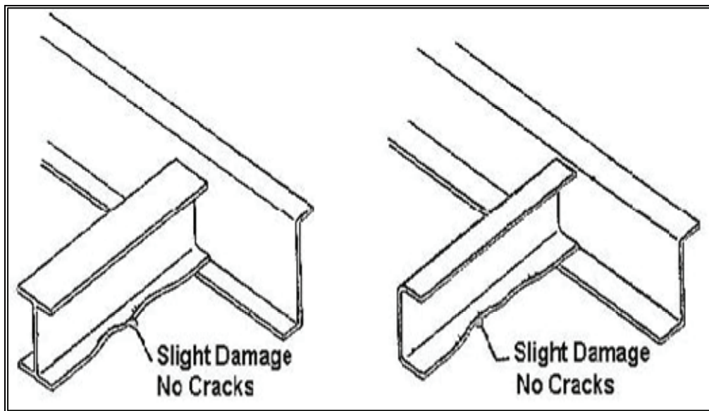
Figure 15-11. Cross Member Damage Not Requiring Replacement
