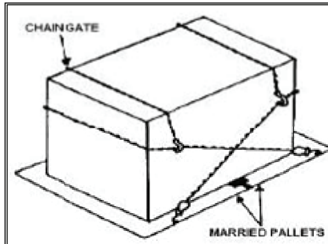
Figure 18-12. Chain Gate
