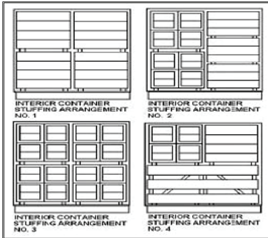
Figure 12-6. Methods for Stuffing Various Sizes of Wooden Boxes and Crates (Rear View)
