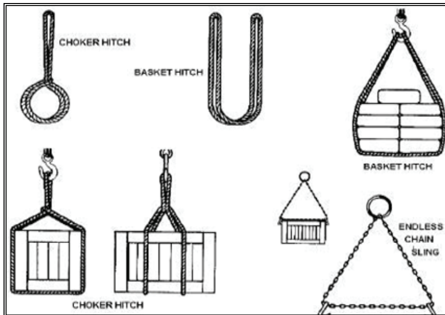
Figure 4-2. Types of Endless Slings
