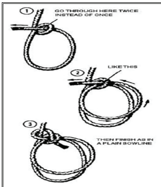
Figure 6-18. Tying a French Bowline
