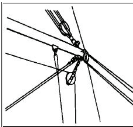
Figure 3-28. Doubling-Up Cargo Runner Using Doubling-Up Pad Eye
