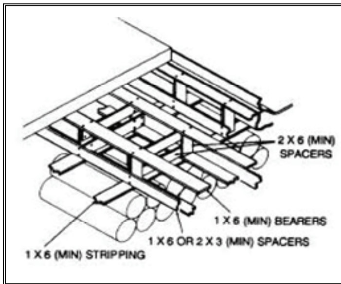
Figure 9-41. Tomming in Square of Hatch
