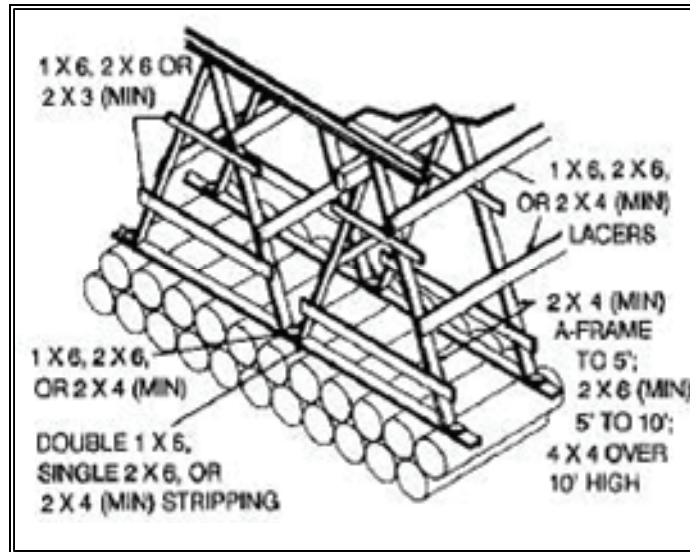
Figure 9-39. Overhead A-Frame Tomming
