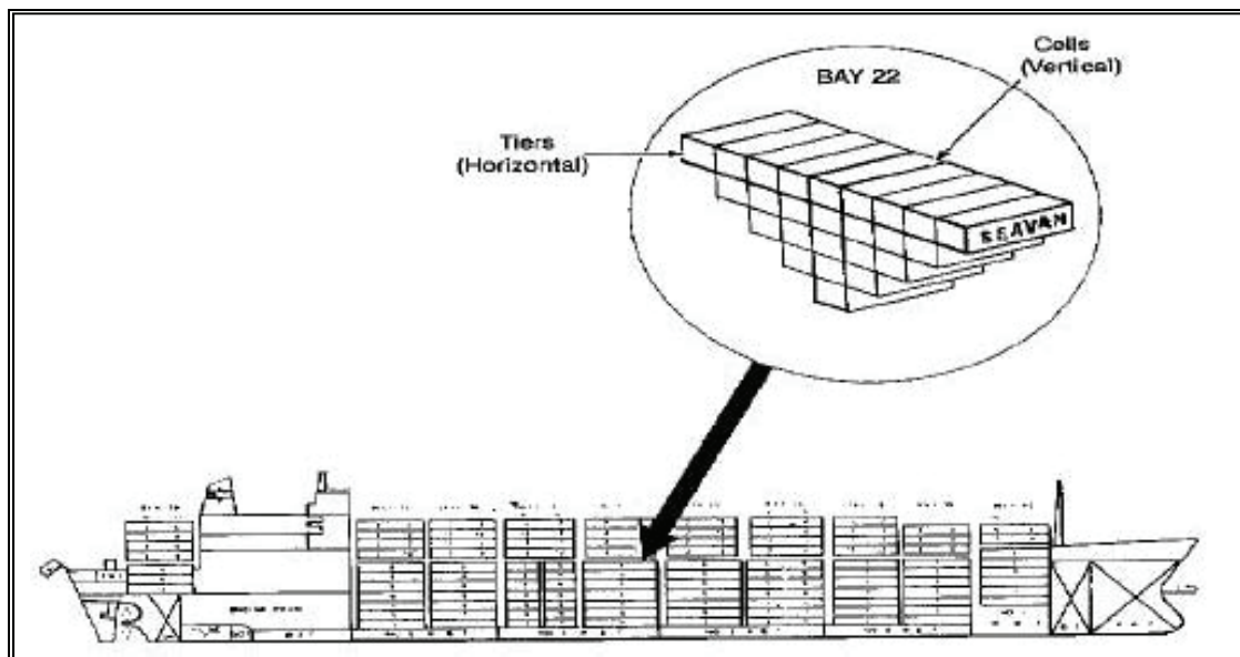
Figure 7-7. Example of Cells, Bays, and Tiers
