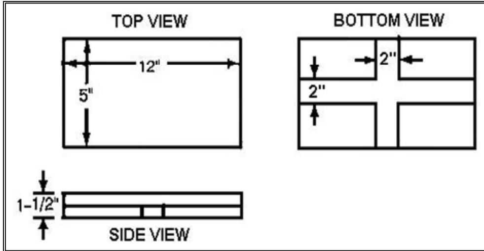
Figure 18-9. Sampler Spacer
