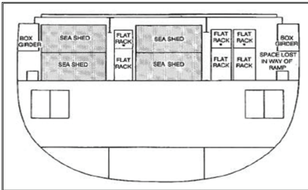
Figure 2-7. Sea Sheds Stacked and Loaded in Container Ship Hold
