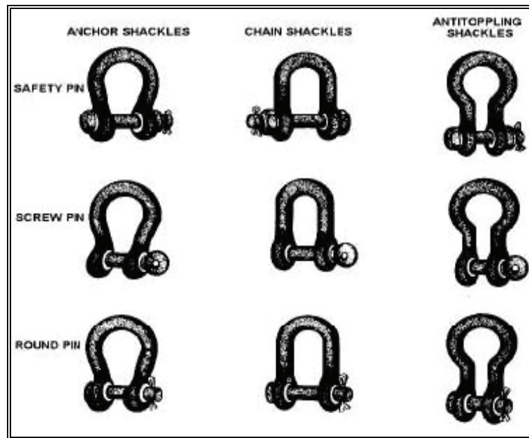
Figure 3-3. Shackles and Safety Pins
