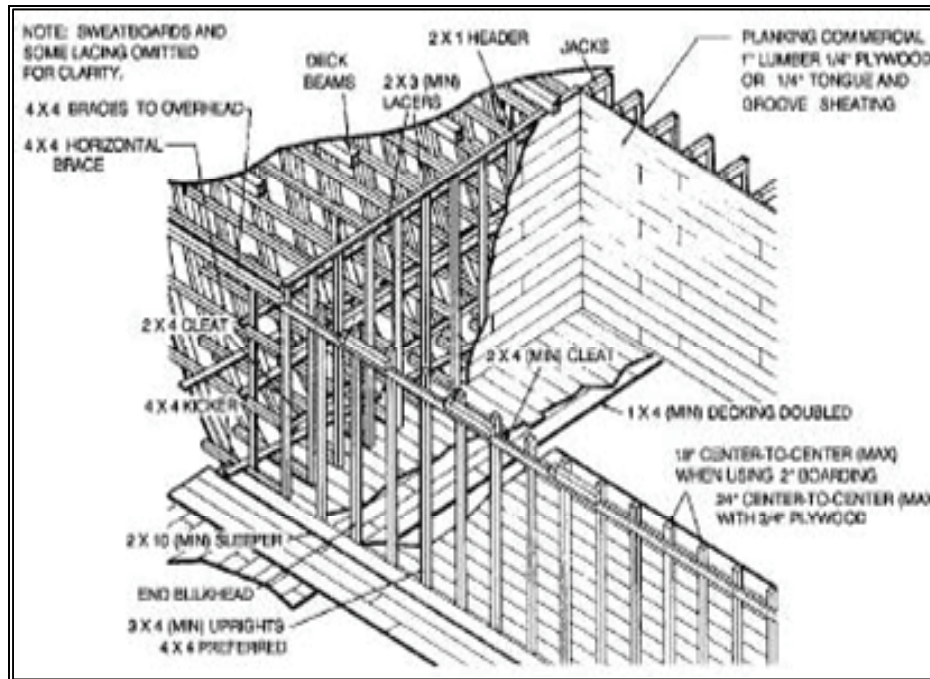
Figure 9-37. Construction Details - Class A Magazine
