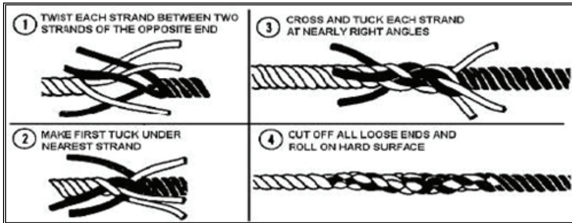
Figure 6-22. Short Splice
