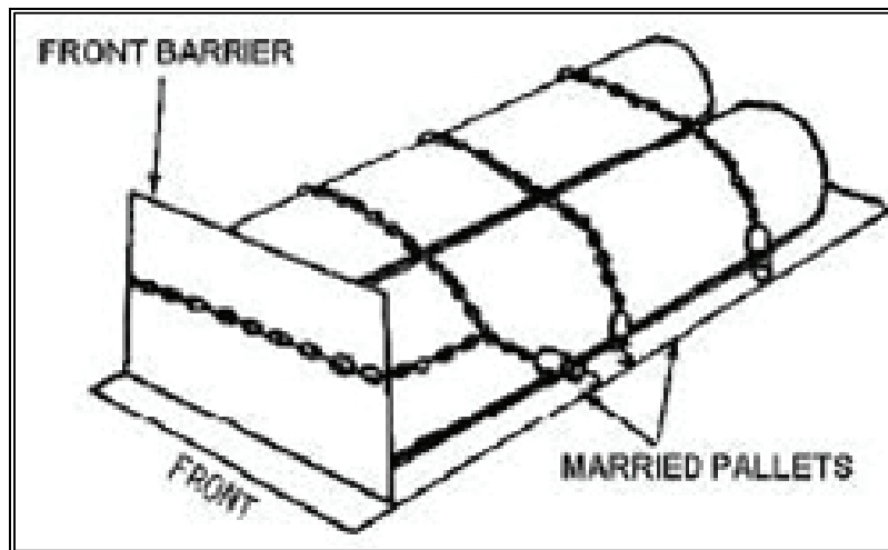
Figure 18-11. Pallet Barrier
