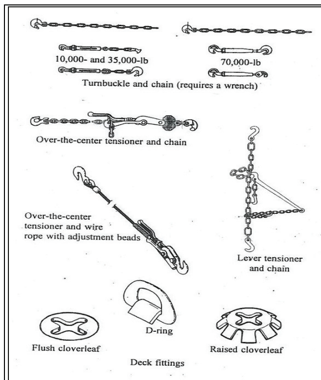
Figure 8-9. Lashing Material for RO/RO Ships
