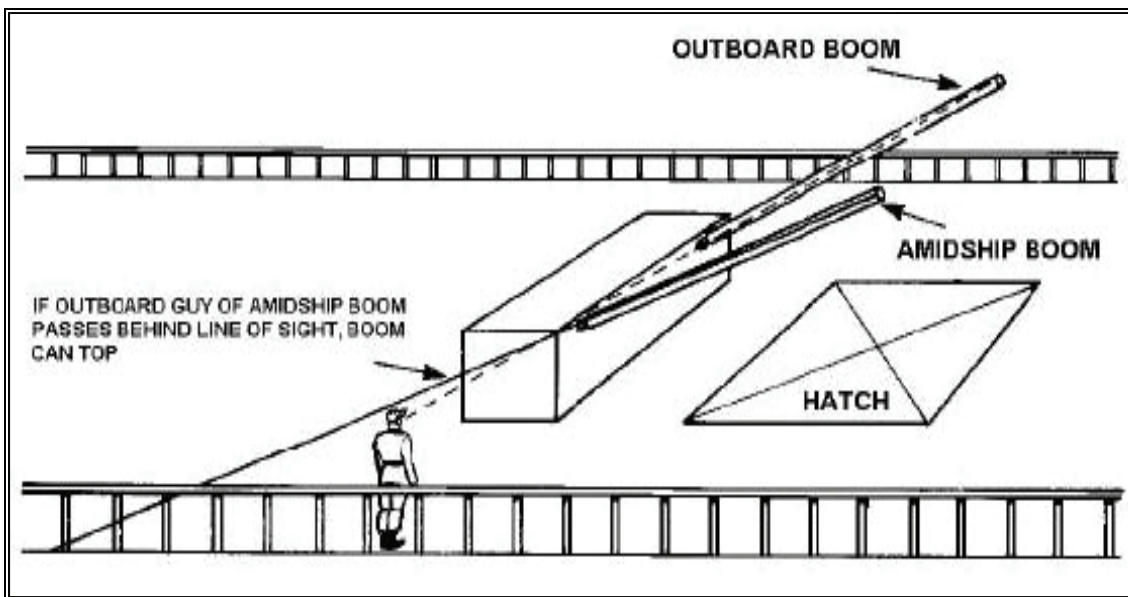
Figure 3-18. Determining if Amidship (Stay) Boom Can Top
