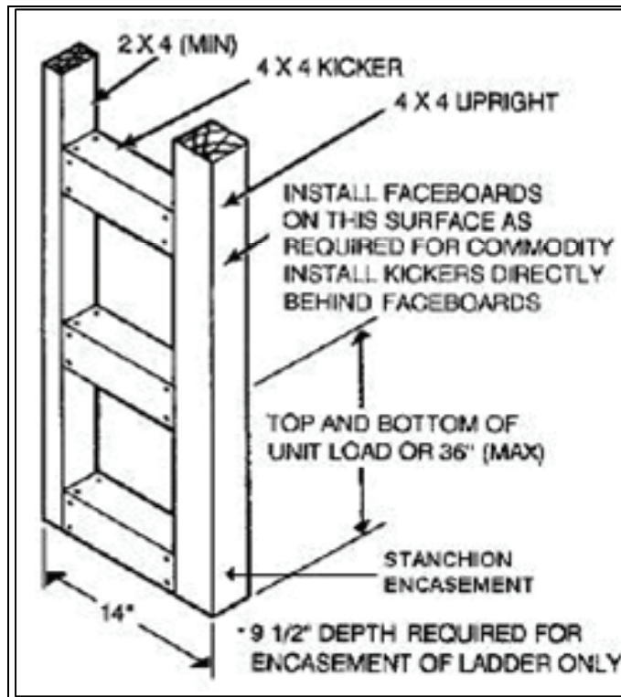
Figure 10-7. Ladder and Stanchion Encasement
