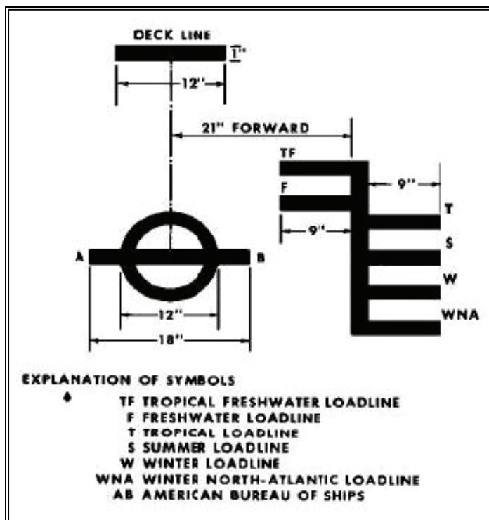
Figure 7-2. Loadline Marks
