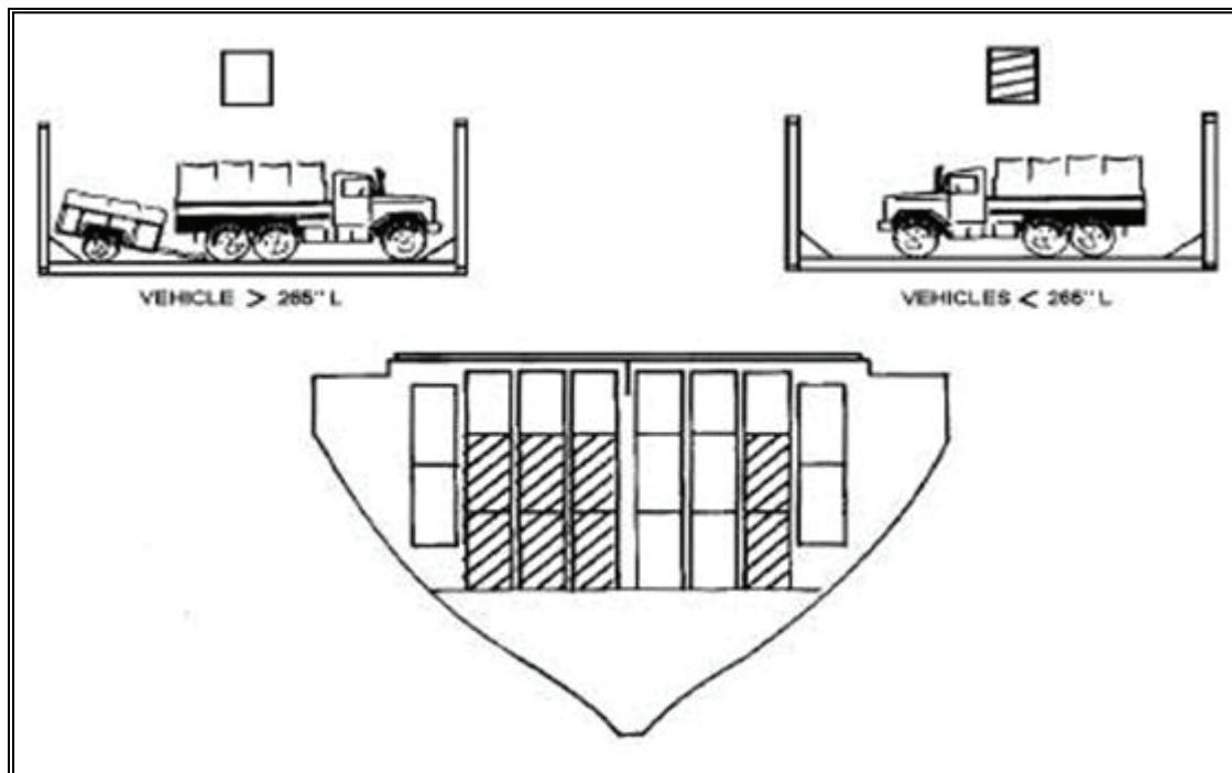
Figure 8-28. Required Cargo Mix for Holds 7A and 8F – Hatch Square Method
