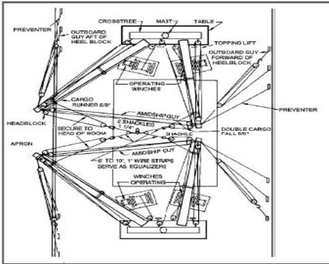
Figure 3-33. Rigging Four Booms with a Double Purchase
