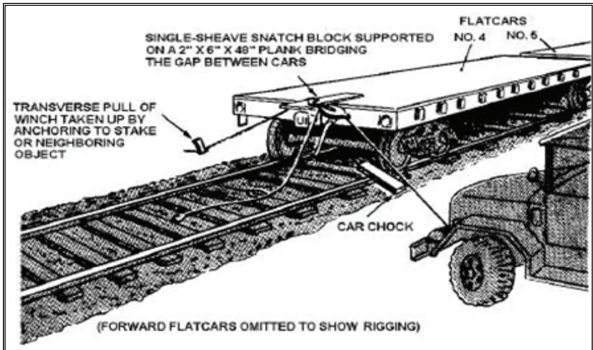
Figure 20-3. Vehicle Winch Used to Power Towing Cable
