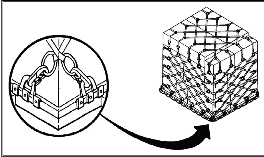
Figure 18-6. Typical Net Attachment
