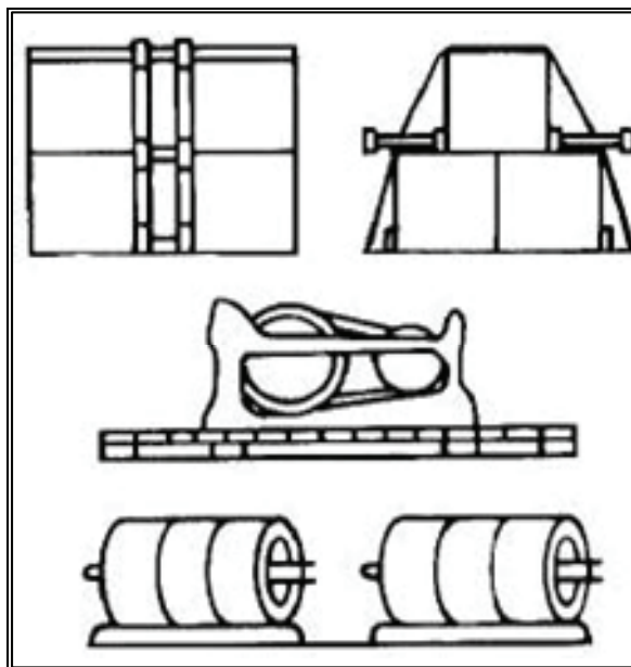
Figure 12-7. Distribution of Heavy Loads in Containers
