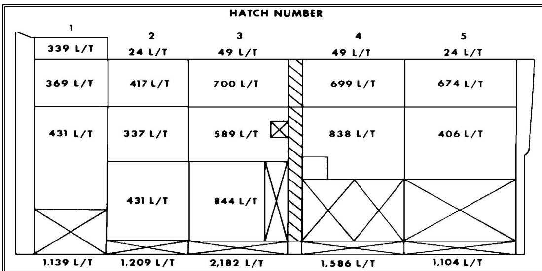
Figure 7-4. Weight Distribution Plan
