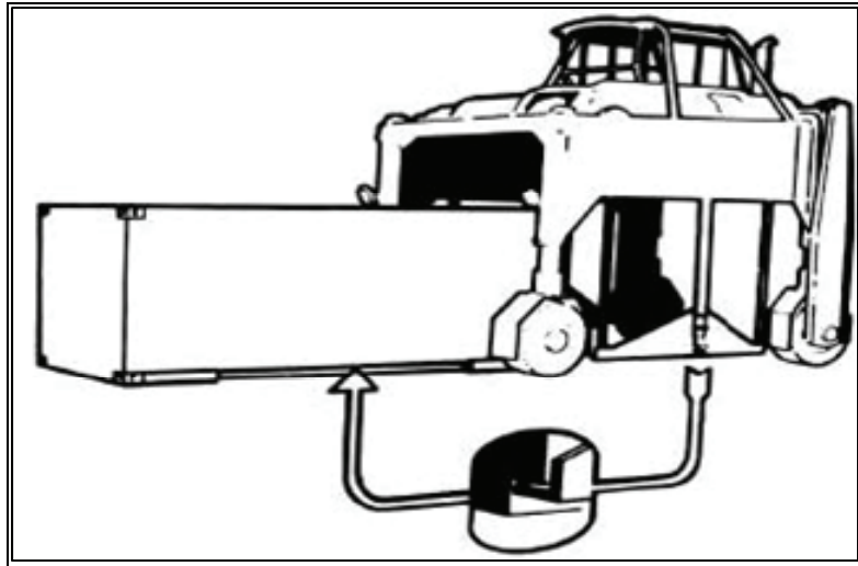
Figure 13-16. Straddle Carrier
