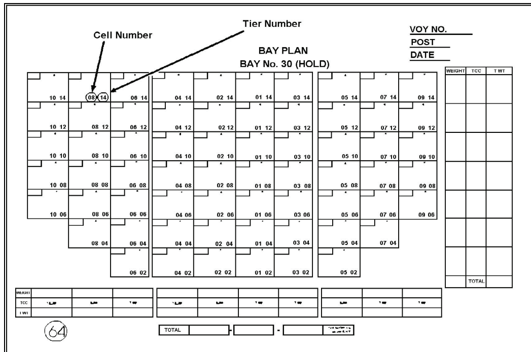
Figure 7-9. Bay Plan
