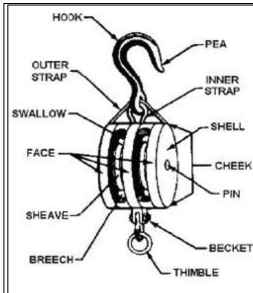
Figure 6-1. Components of Wooden Blocks
