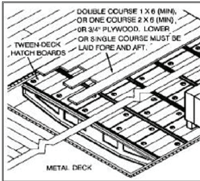
Figure 9-21. Tween-Deck Hatch Boards
