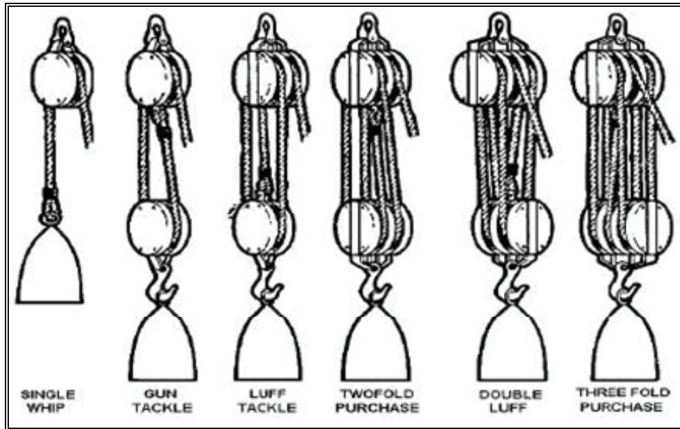
Figure 6-5. Types of Tackles
