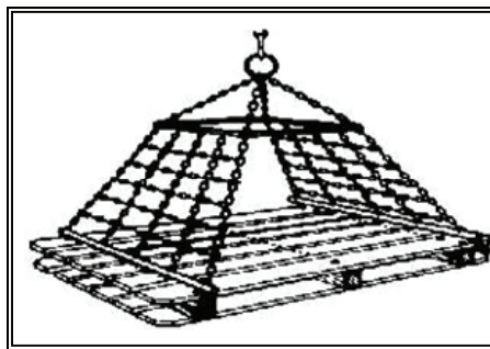
Figure 4-17. Pallet Bridle
