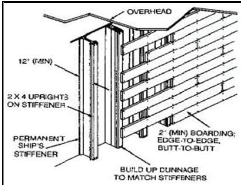
Figure 9-25. Heat Bulkhead, Stiffener Side
