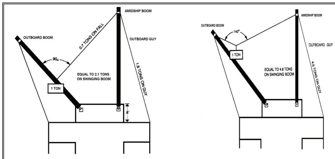
Figure 3-14. Load Suspended at 90-Degree and 140-Degree Fall Angle
