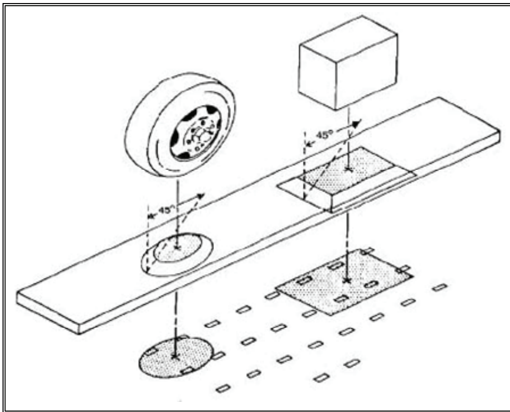
Figure 18-15. Increasing an Area by Shoring
