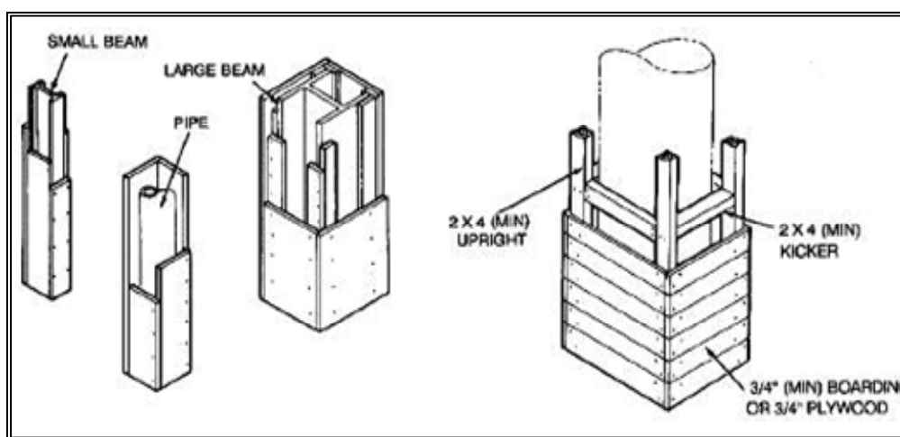
Figure 9-35. Typical Complete Encasements
