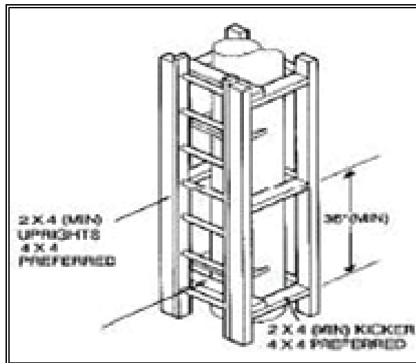
Figure 9-5. Typical Partial Encasement
