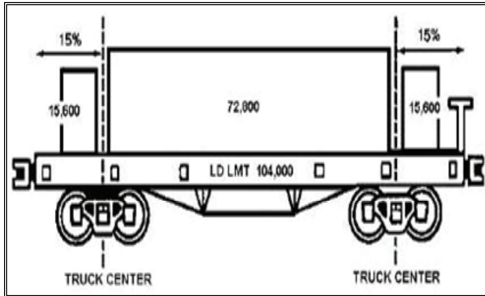
Figure 20-4. Maximum Load Weight Guidance
