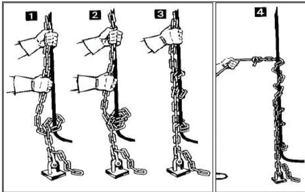
Figure 3-11. Steps in Applying Stopper Chain
