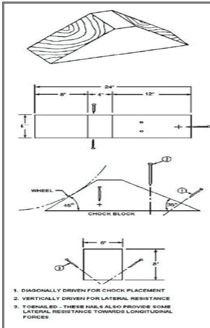
Figure 20-7. Standard Pattern 16 Block
