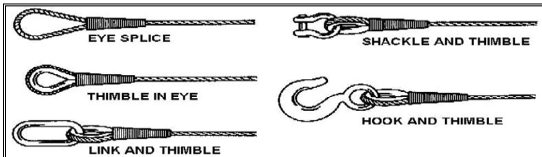
Figure 4-1. Sling Eyes
