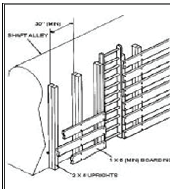
Figure 9-32. Nonheat Bulkhead against Shaft Alley
