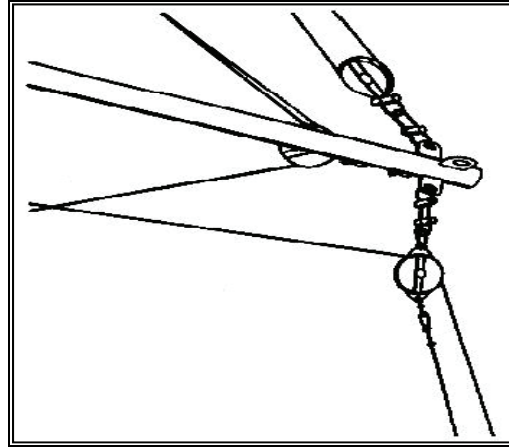
Figure 3-29. Doubling-Up Cargo Runner Using Bottom of the Block
