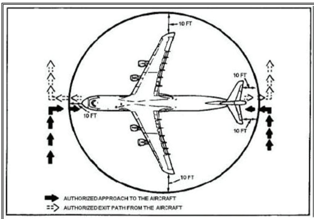
Figure 16-6. Circle of Safety
