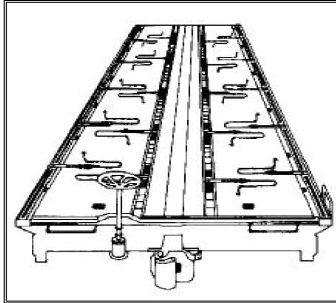
Figure 20-18. Flatcar, 60-Foot HTTX
