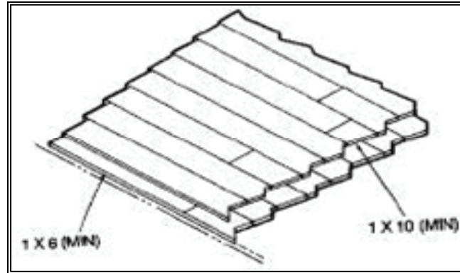
Figure 9-15. Full Decking
