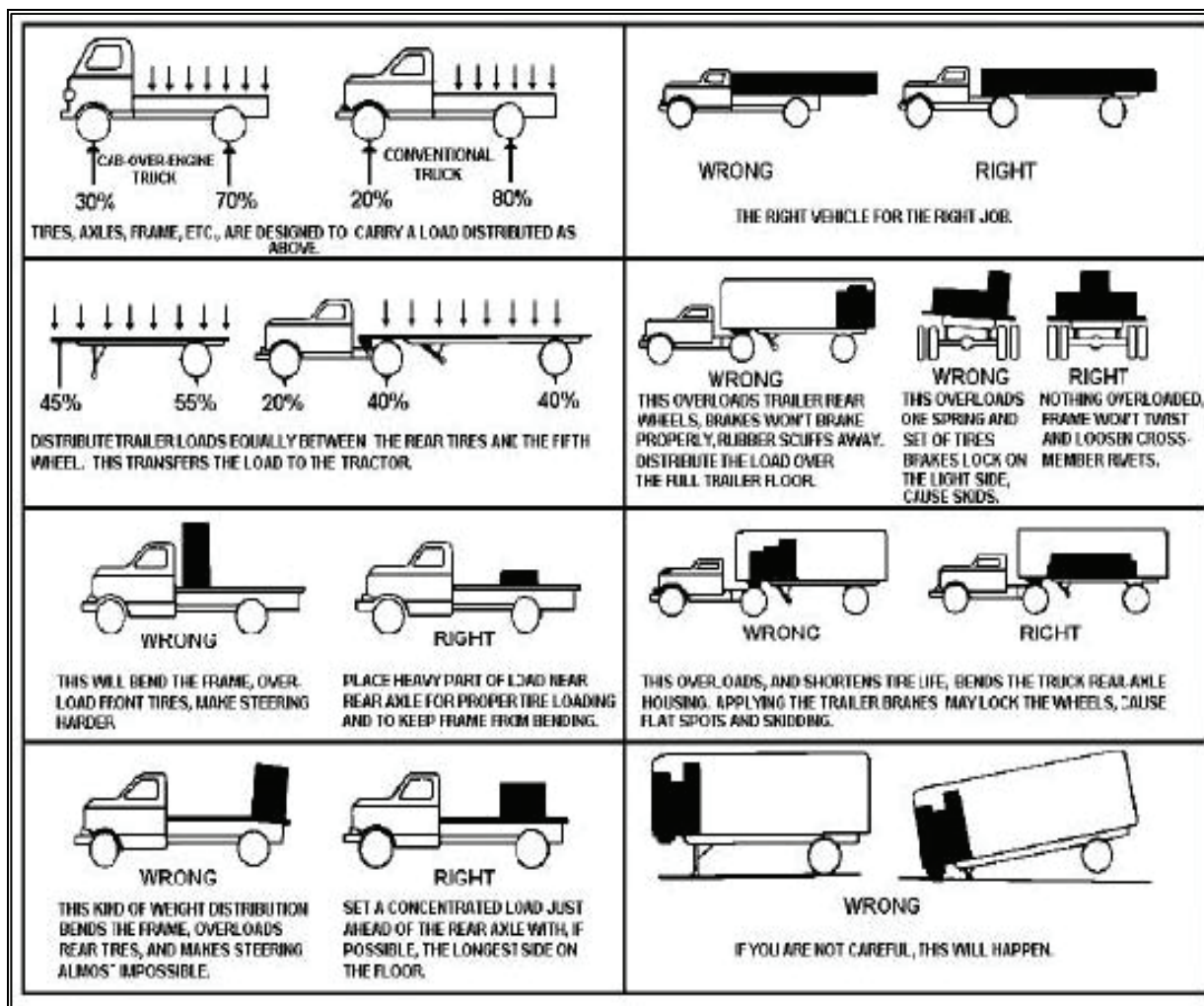
Figure 19-1. Right and Wrong Ways to Distribute Truck Loads
