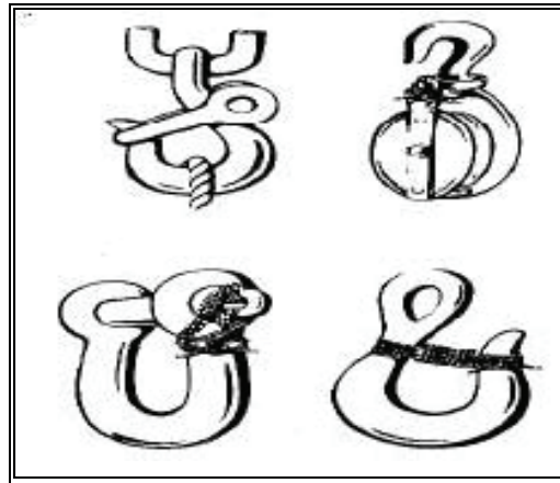
Figure 3-4. Mousing Hooks
