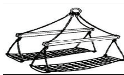
Figure 4-13. Vehicle Spreader with Wheel Nets
