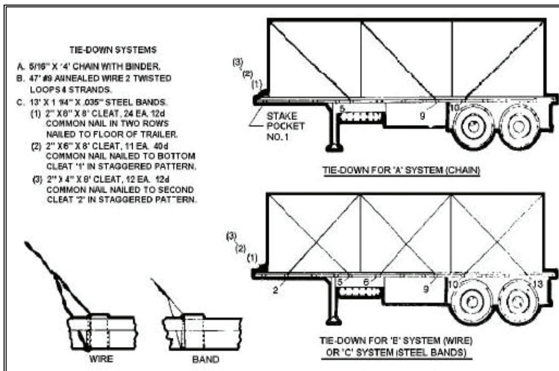
Figure 19-5. Recommended Tie-Down for Three CONEXs on M127 Semitrailer
