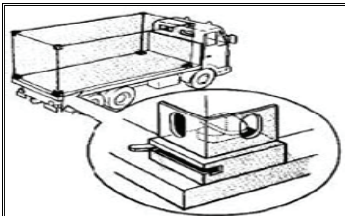
Figure 13-12. Container Secured with Locking Device on Truck
