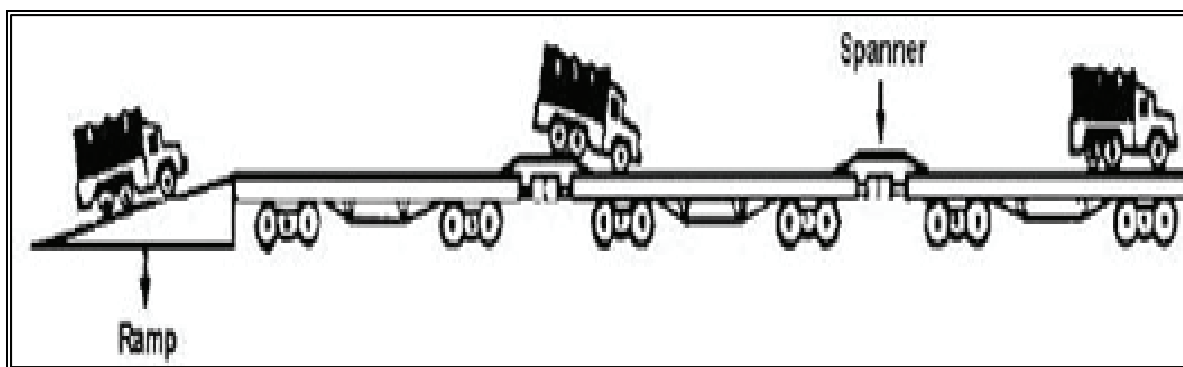
Figure 20-1. Circus Method of Loading Vehicles
