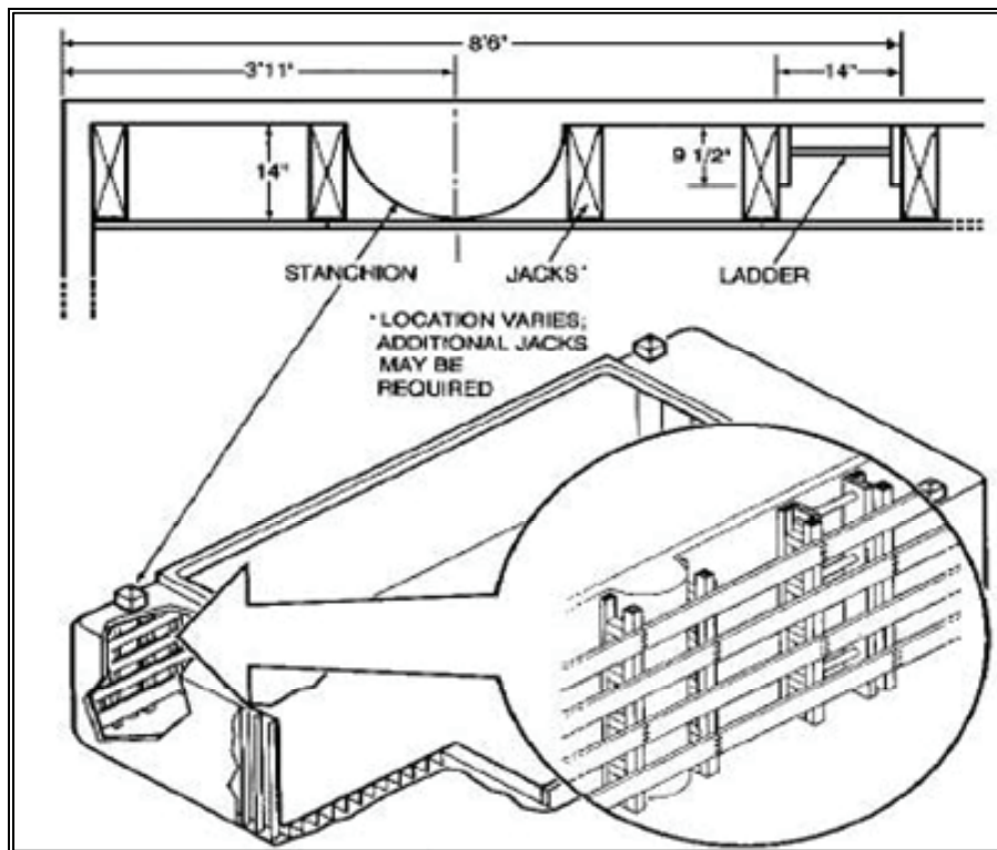
Figure 10-9. Diagonally Braced Bulkhead
