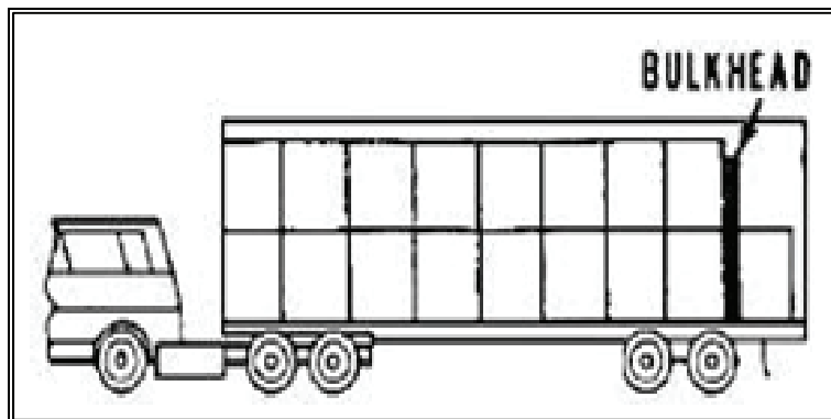
Figure 12-5. Bulkhead Constructed to Support Load
