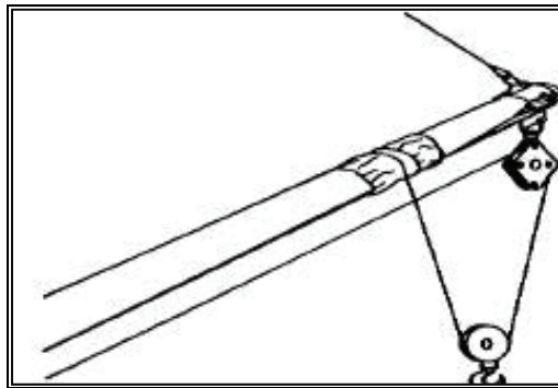
Figure 3-30. Doubling-Up Cargo Runner by Taking Turns on the Boom
