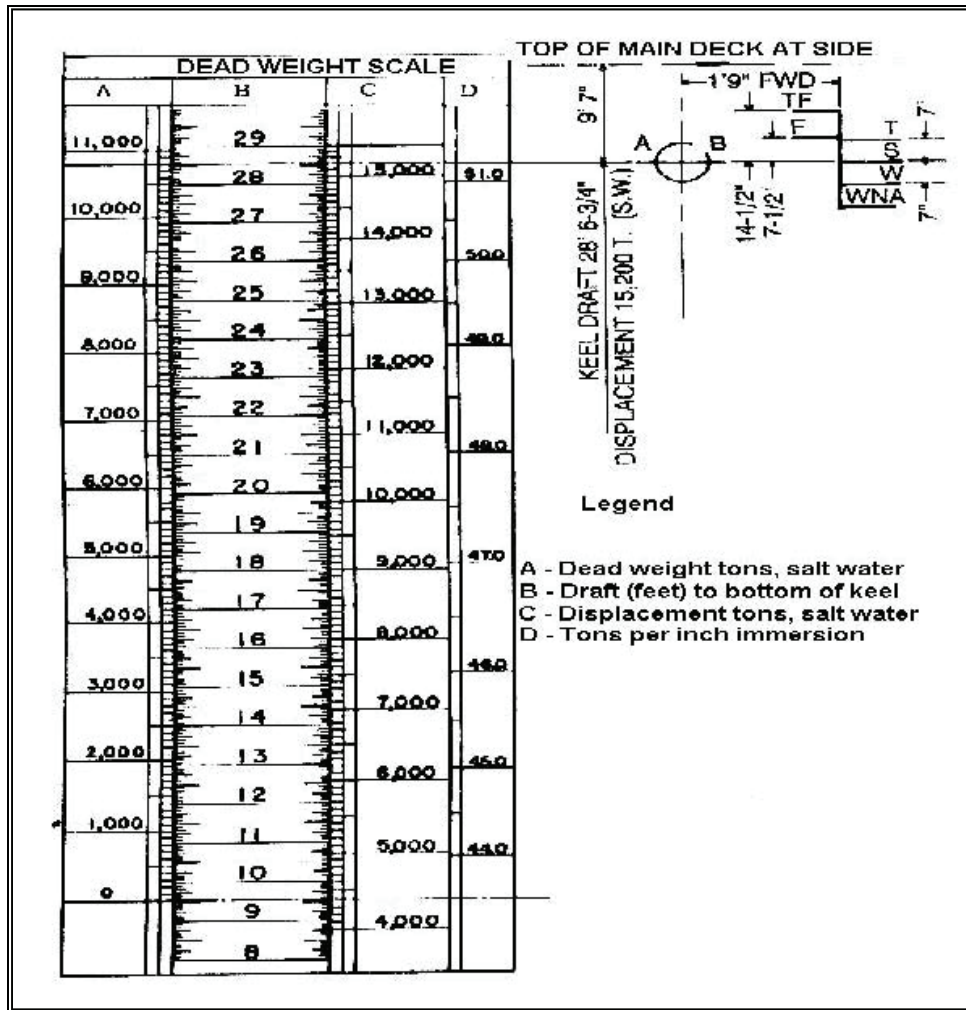
Figure 7-3. Vessel Dead Weight Scale
