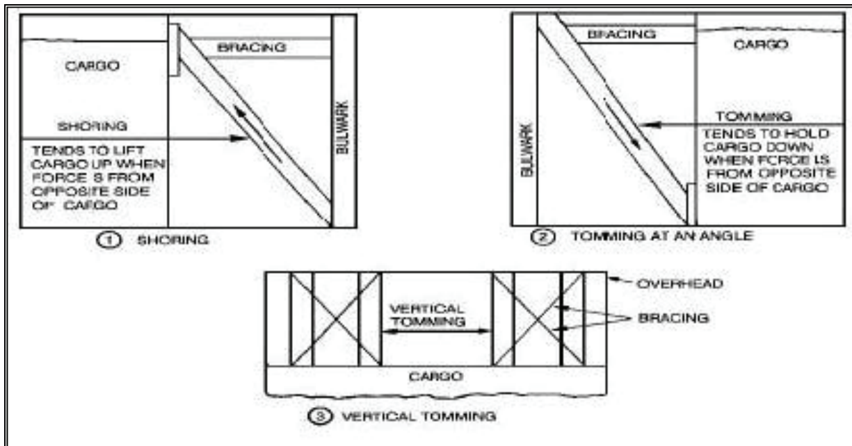
Figure 8-14. Shoring and Tomming Methods
