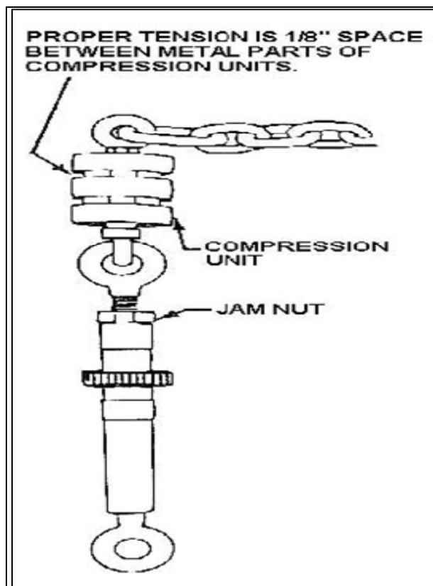
Figure 20-29. Turnbuckle with Jam Nut and Compression Unit
