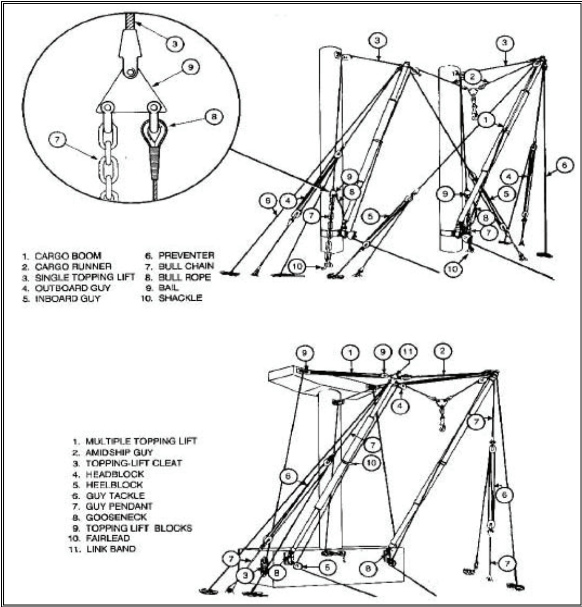
Figure 3-6. Running Rigging
