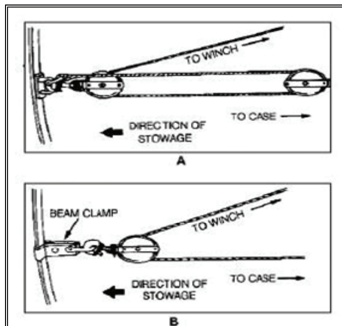
Figure 8-3. Use of Tackle and Beam Clamps
