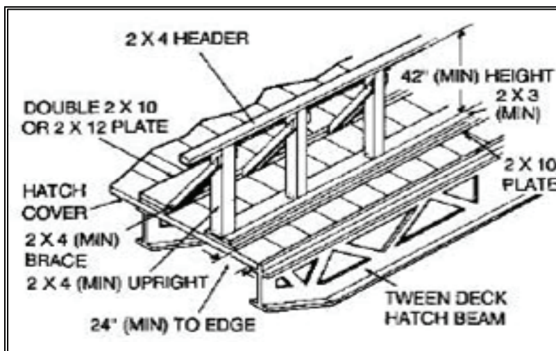
Figure 9-42. Open-Hold Guardrail
