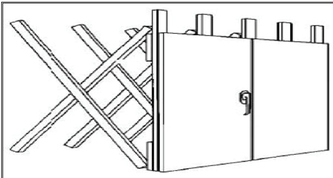
Figure 20-6. Correctly Constructed Bulkheads for Doorway Protection
