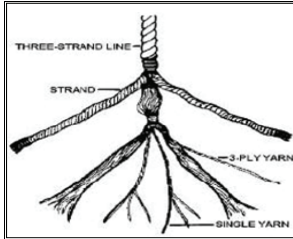
Figure 6-11. Fabrication of Fiber Line
