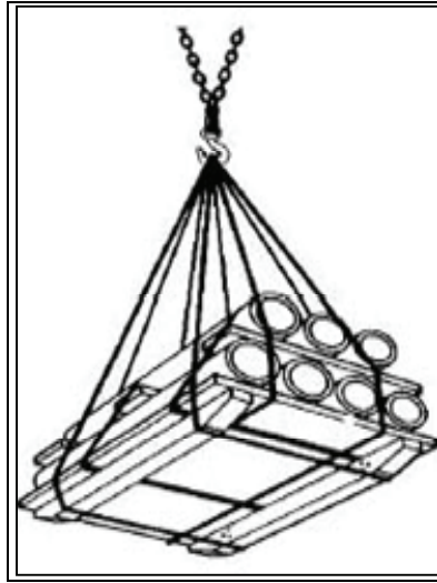
Figure 4-12. Sled Pallet
