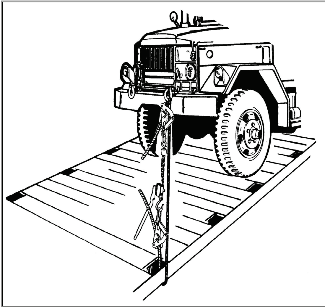
Figure 20-13. Chain Hoist with Grippers in Use
