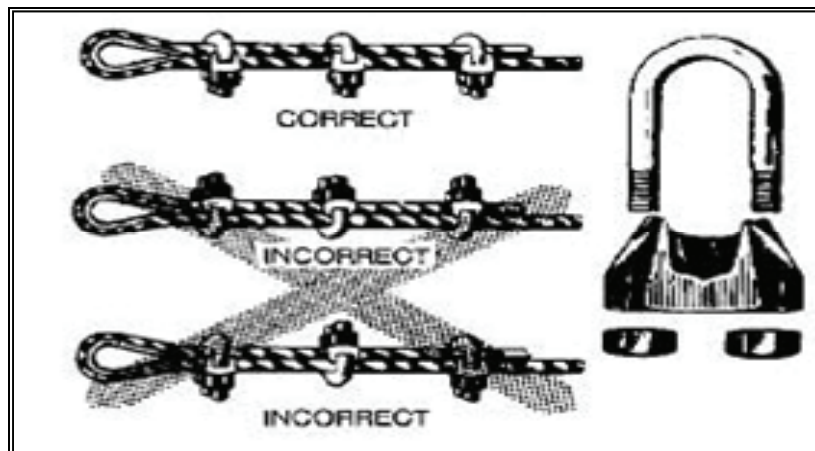
Figure 6-25. Correct Use of Wire Clips
