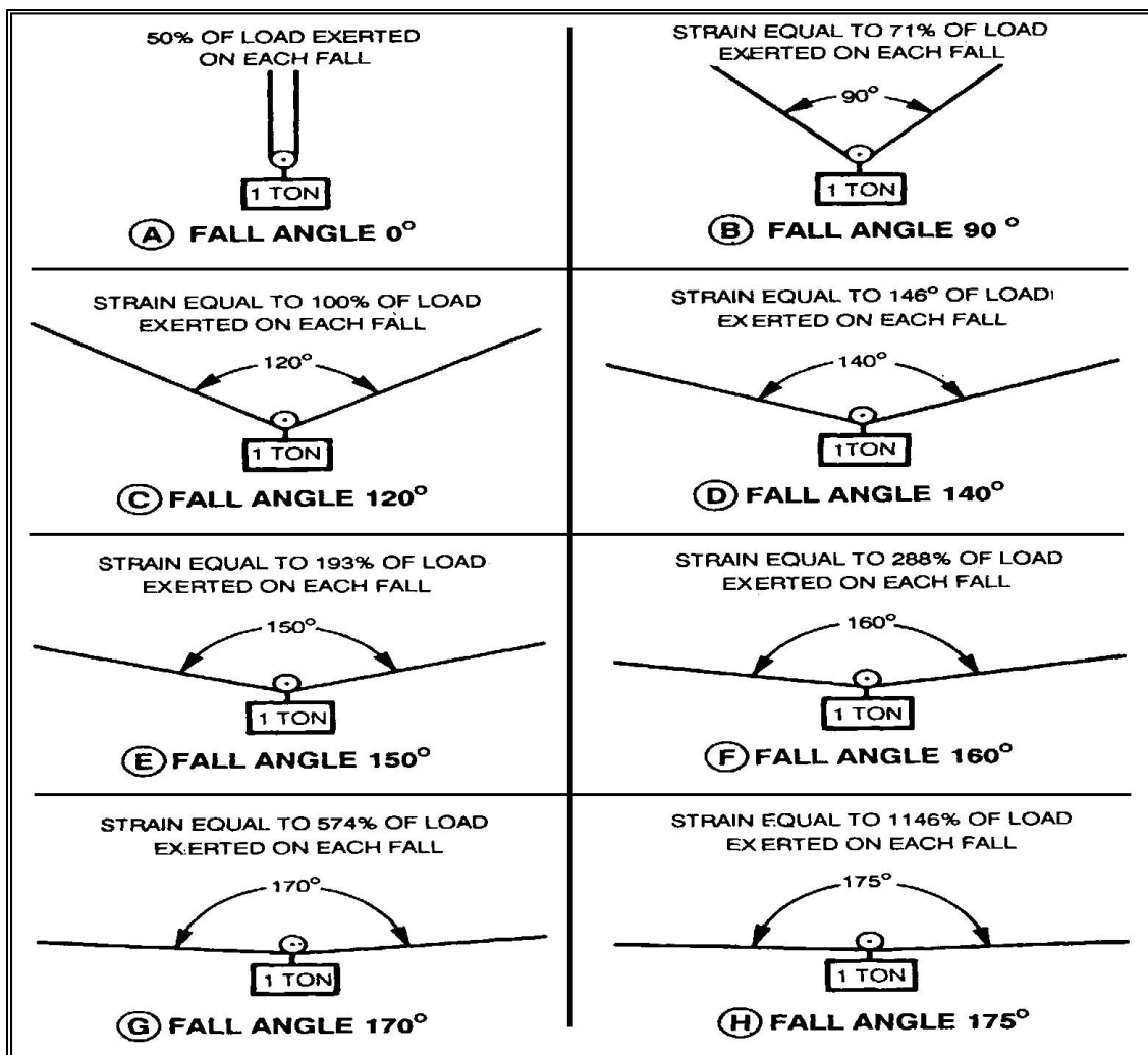
Figure 3-16. Strain on Fall Angles
