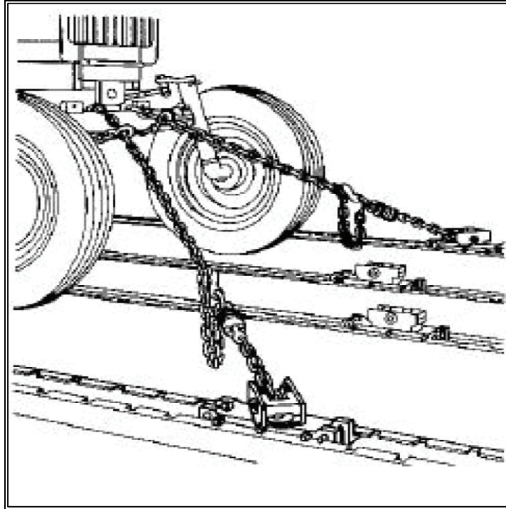
Figure 20-20. Saddleback Winch, 360-Degree
