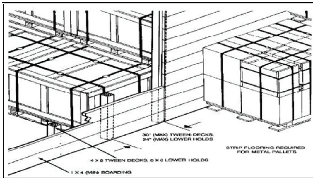
Figure 9-34. Division Bulkhead
