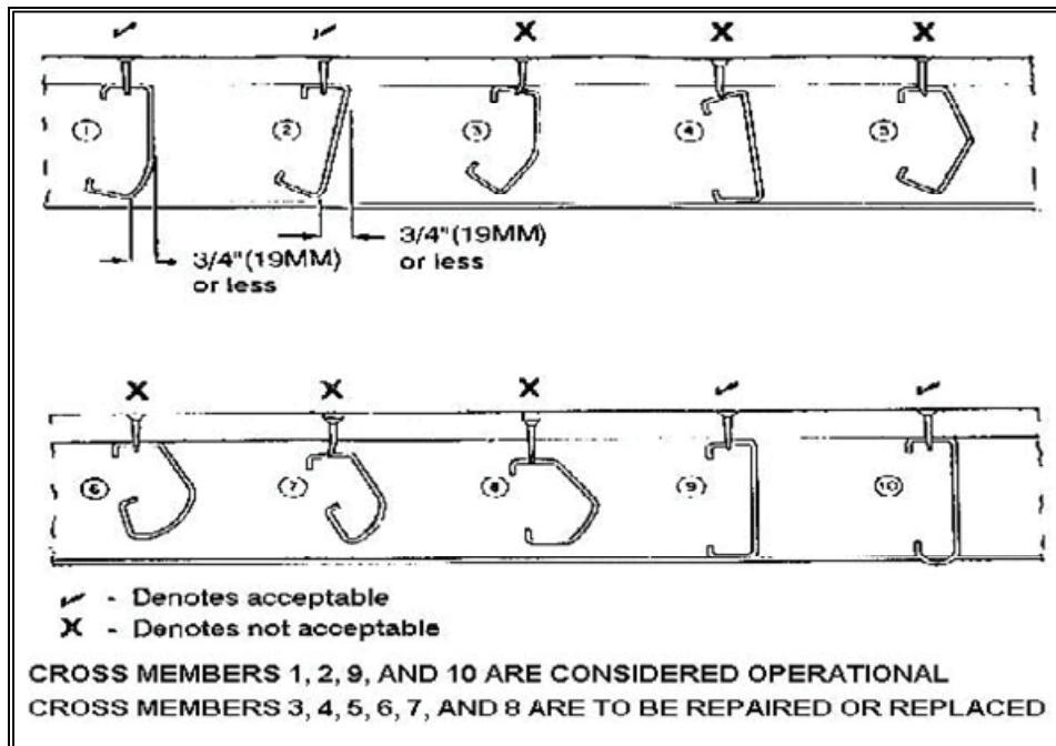
Figure 15-9. Examples of Cross Member Damage
