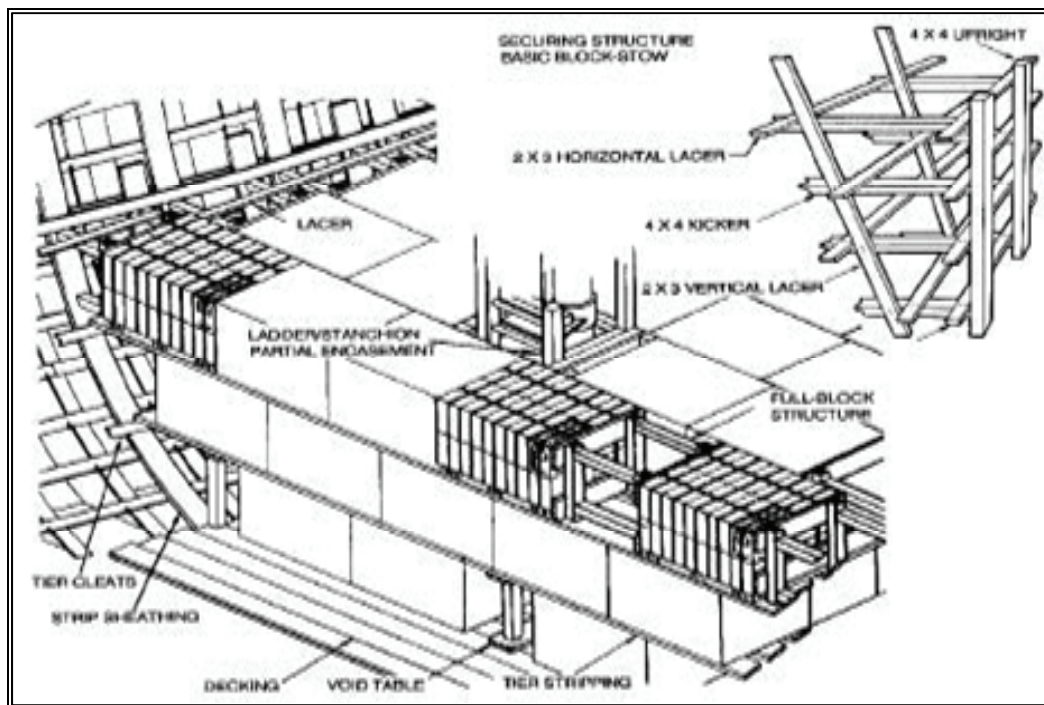
Figure 9-9. Typical Block Stowage, Lower Hold Number 1
