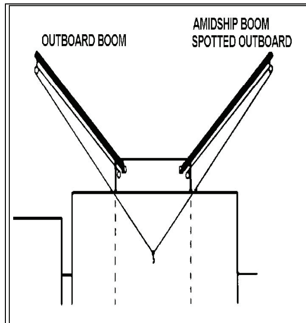
Figure 3-24. Spotting Booms with a Wing-and-Wing Rig
