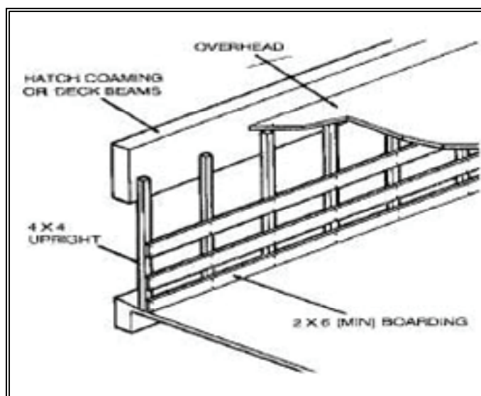
Figure 9-31. Fence at Hatch Edge
