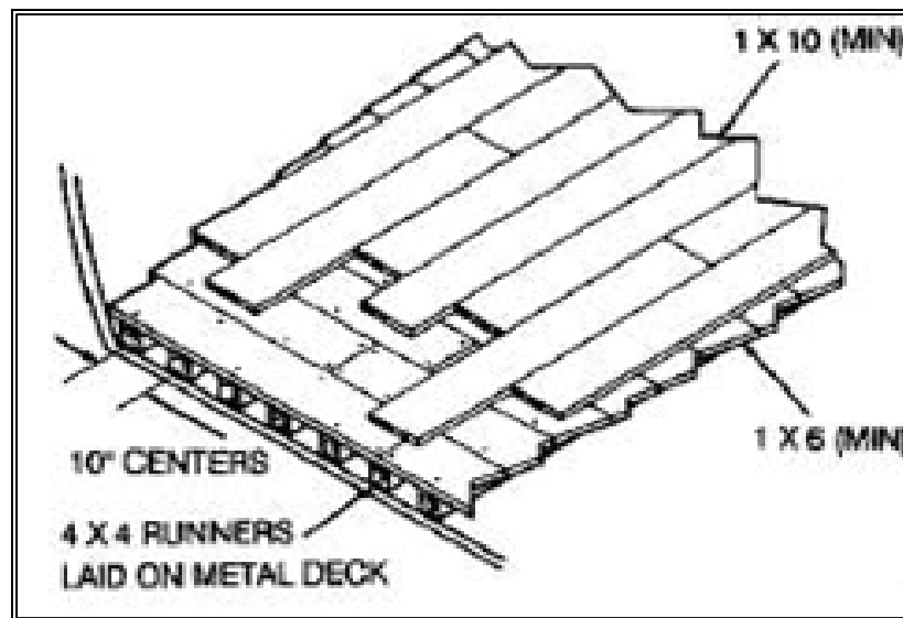
Figure 9-16. 1-Inch Wood Decking on 4 x 4 Runners
