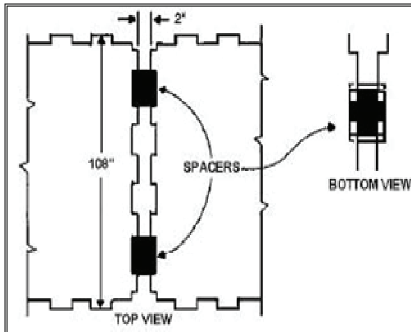
Figure 18-8. Use of Spacers
