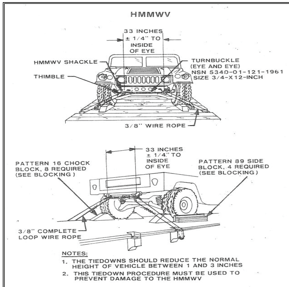
Figure 20-31. Front and Rear Securement of a HMMWV
