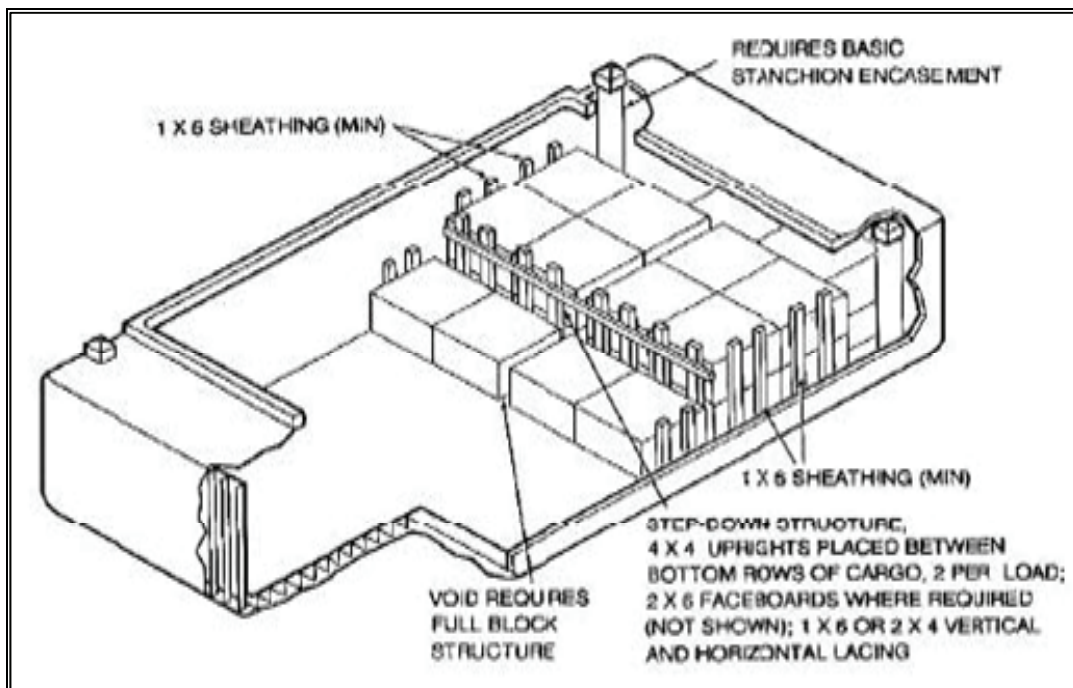
Figure 10-10. Partition Bulkhead
