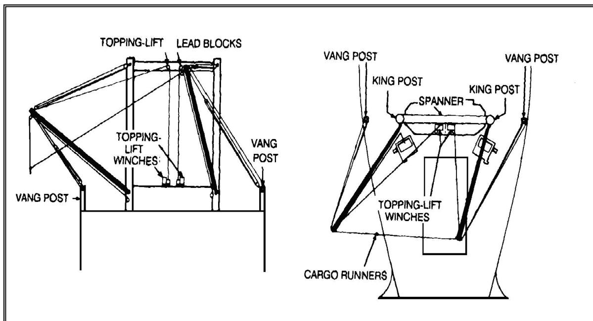
Figure 3-20. Farrel Rig
