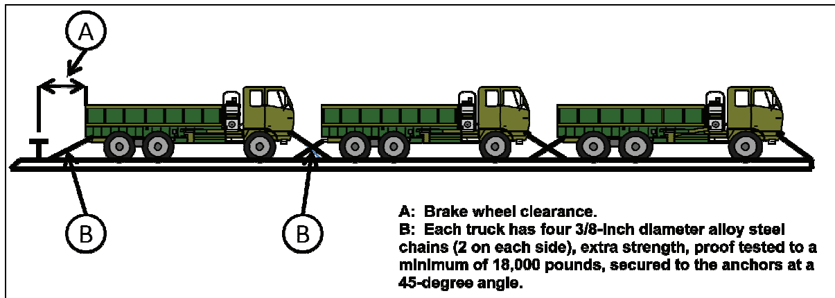
Figure 20-30. Chain Securement of a 2 1/2-Ton Truck/LMTV
