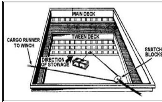
Figure 8-2. Dragline Rigging
