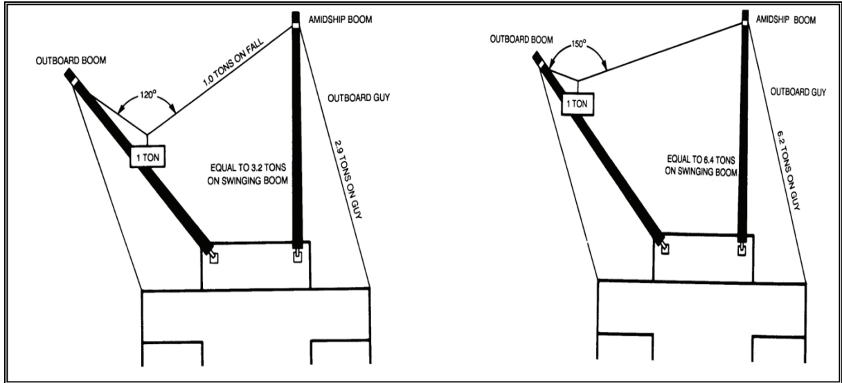
Figure 3-15. Load Suspended at 120-Degree and 150-Degree Fall Angle
