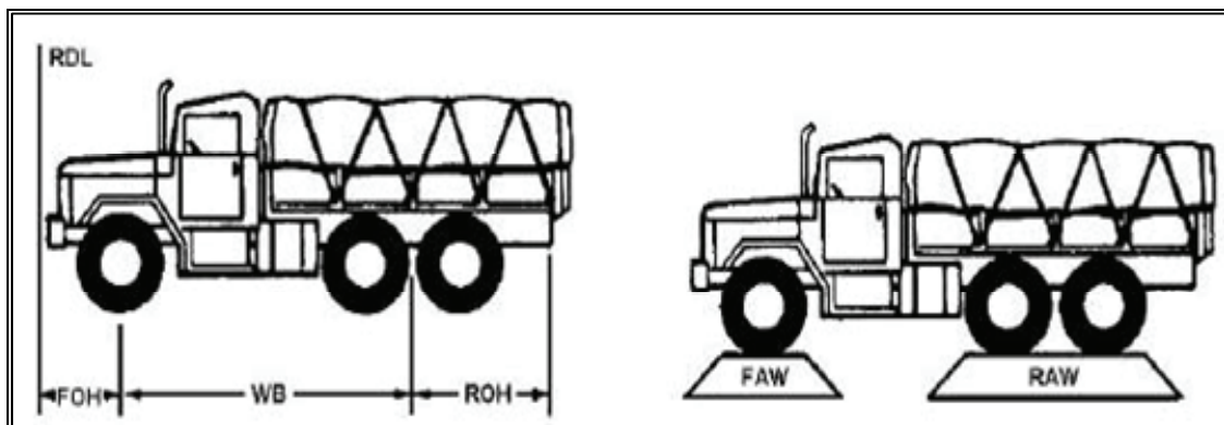
Figure 17-1. Vehicle Measurement Points
