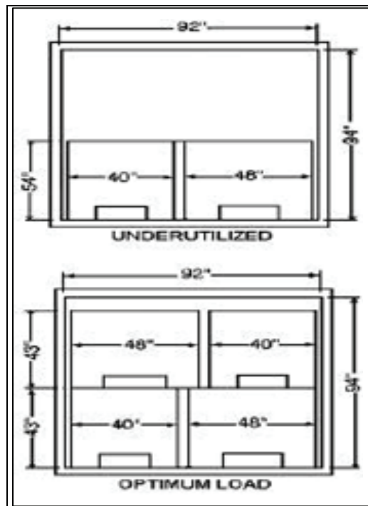
Figure 12-2. Cube Utilization
