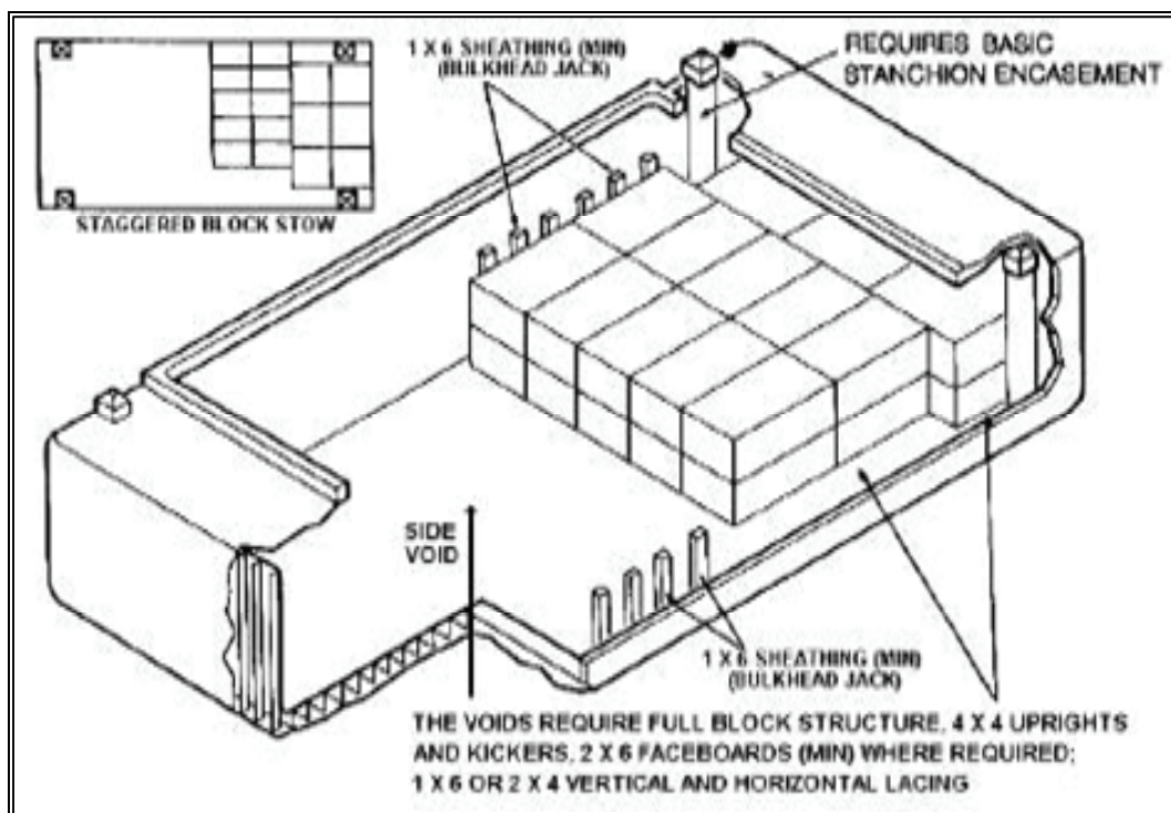
Figure 10-5. Staggered Block Stow and Bulkhead Jack
