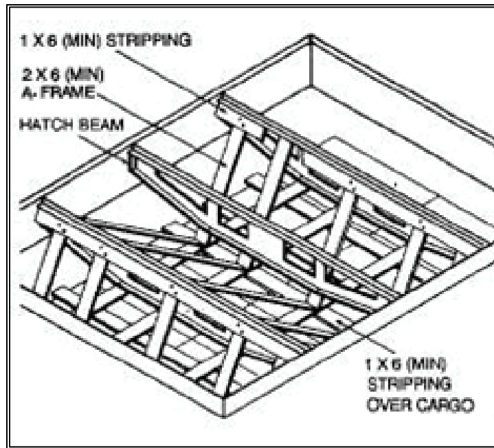
Figure 9-40. Tomming under Tween-Deck Hatch Beams
