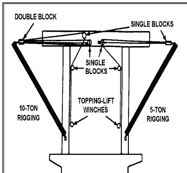
Figure 3-22. Ebel Rig with 5- or 10-Ton Boom Rigging
