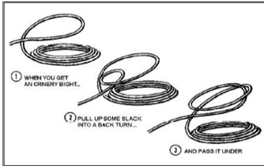
Figure 6-10. Putting a Back Turn in Wire Rope
