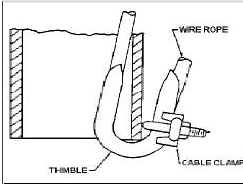
Figure 20-11. Use of Thimble and Cable Clamp
