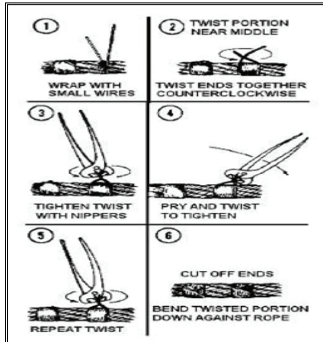
Figure 6-9. Seizing Wire Rope
