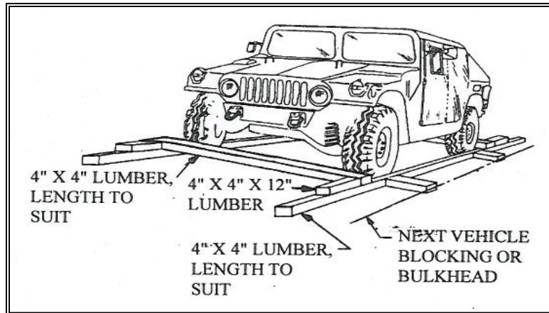
Figure 8-12. Vehicle Secured on Deck with Dunnage
