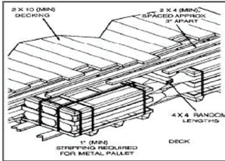
Figure 9-22. Use of Dunnage to Support Decking
