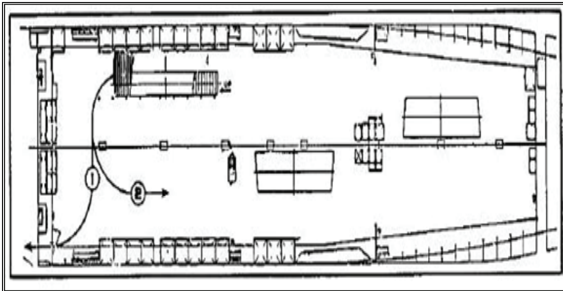
Figure 8-34. RO/RO Flow - "A" Deck
