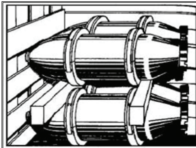
Figure 9-12. Band-to-Band Method of Stowing Bombs
