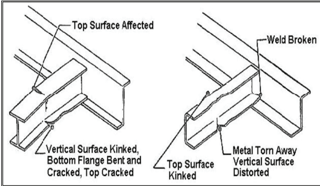
Figure 15-10. Cross Member Damage Requiring Replacement
