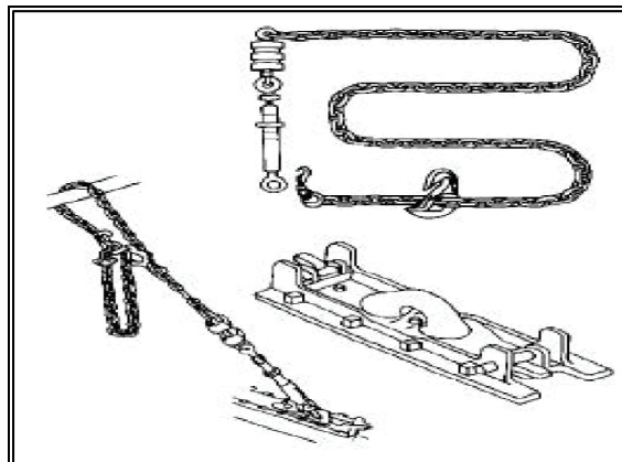
Figure 20-17. Heavy-Duty Chains and Anchors
