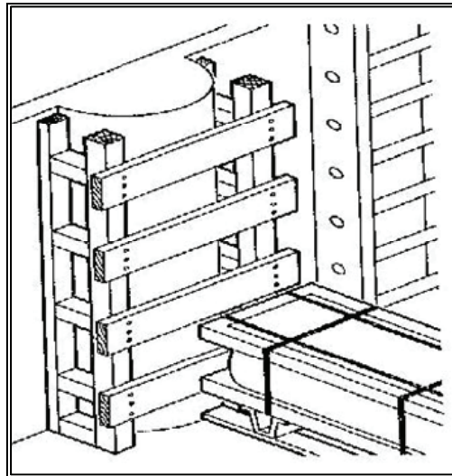
Figure 10-8. Step-Down Structure
