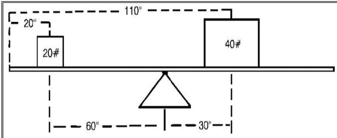
Figure 17-4. Achieving Moment of Balance
