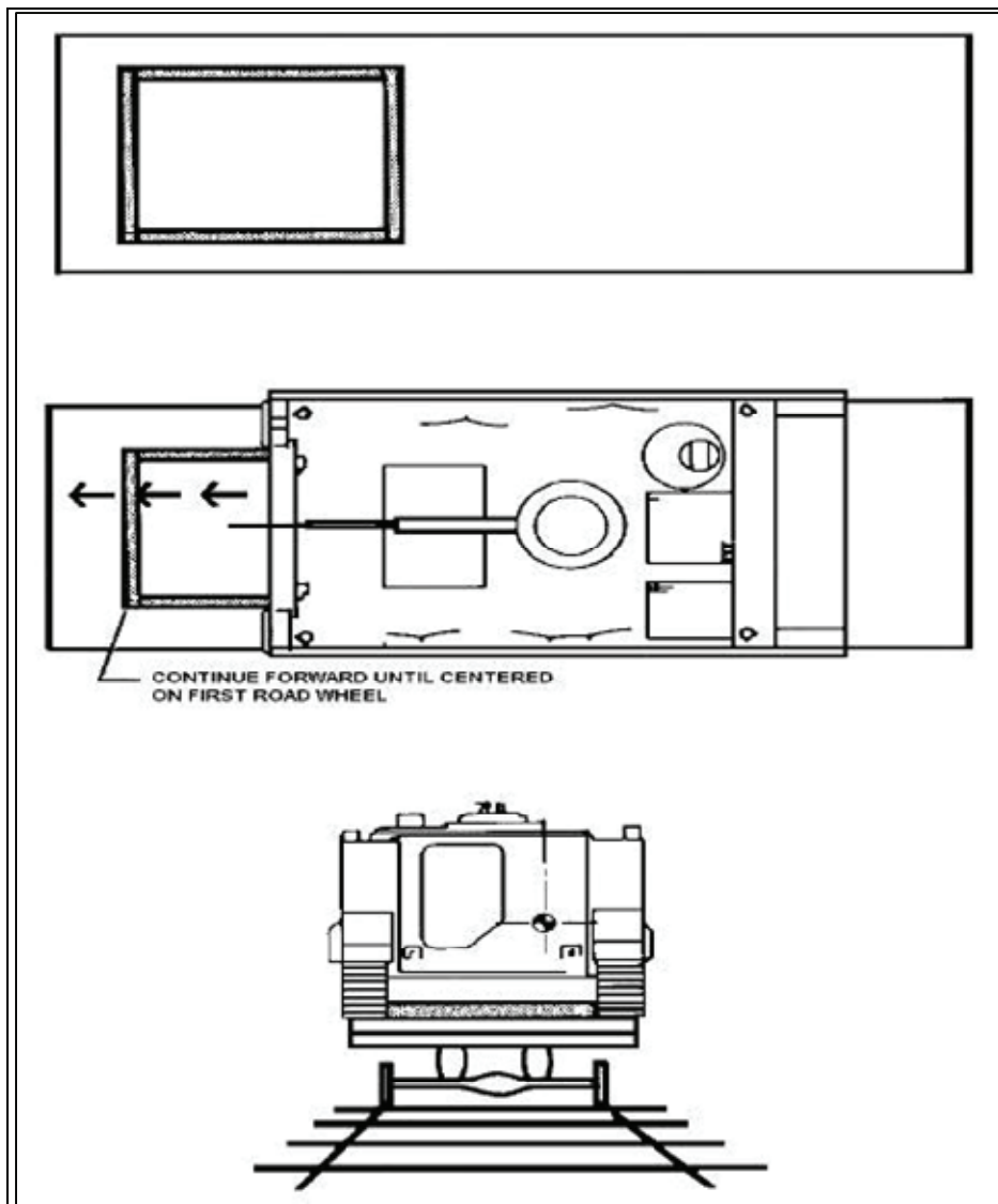
Figure 20-9. Side Blocking Frames
