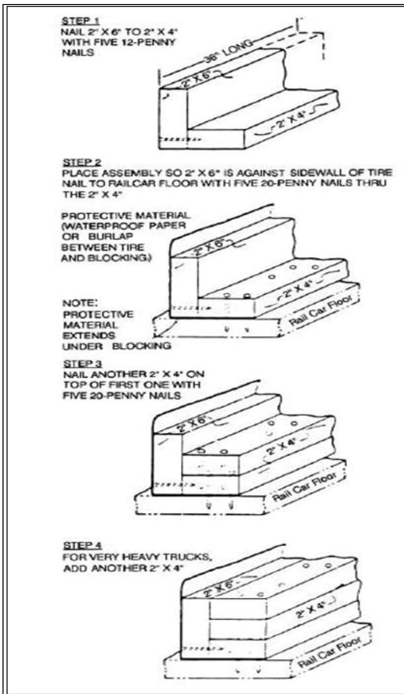
Figure 20-8. How to Make Side Blocking for Wheels
