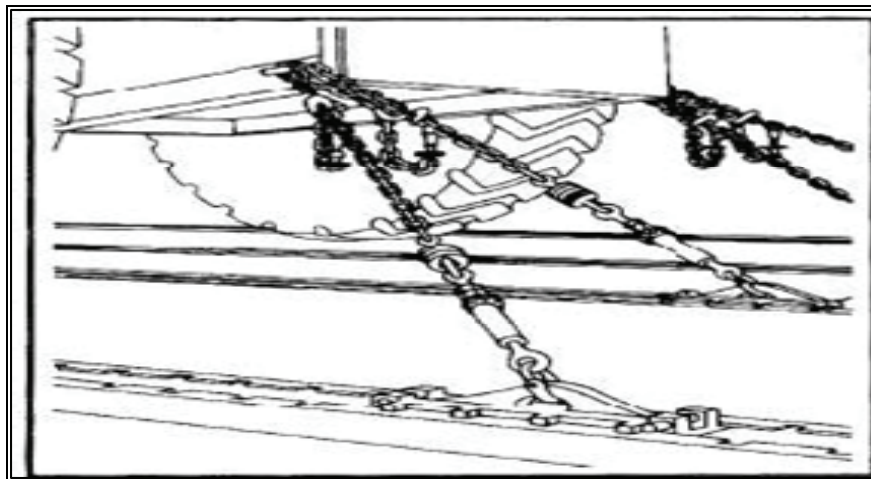
Figure 20-15. DODX Tie-Down Device
