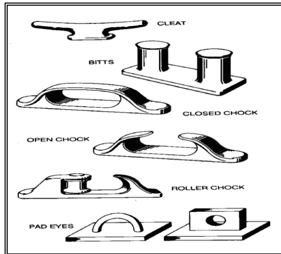
Figure 3-7. Deck Fittings
