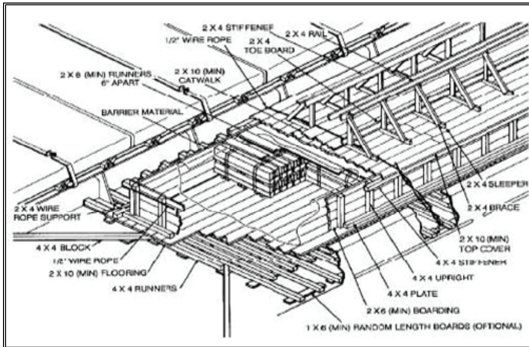
Figure 9-43. Closed Deck-Stow Structure
