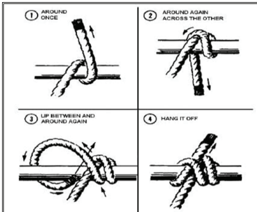
Figure 6-21. Stopper Hitch
