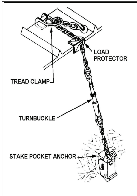
Figure 20-19. Stake Pocket Anchor
