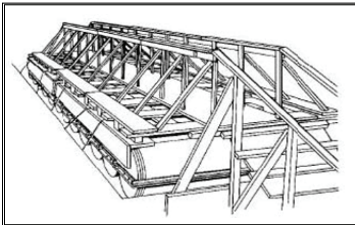
Figure 8-10. Catwalk over Deck Cargo
