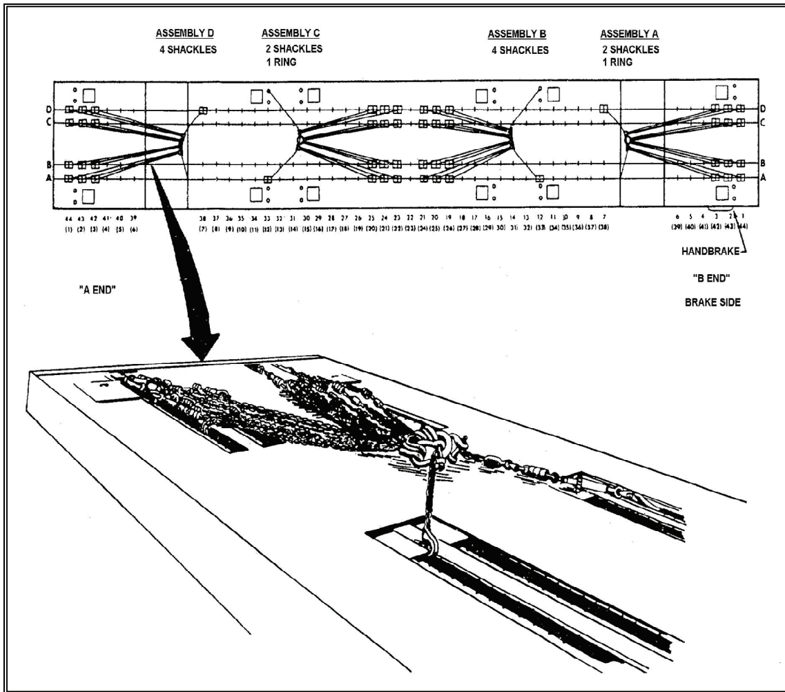
Figure 20-16. Securing Tie-Down Chains and Hardware on the 140-Ton DODX Flatcar
