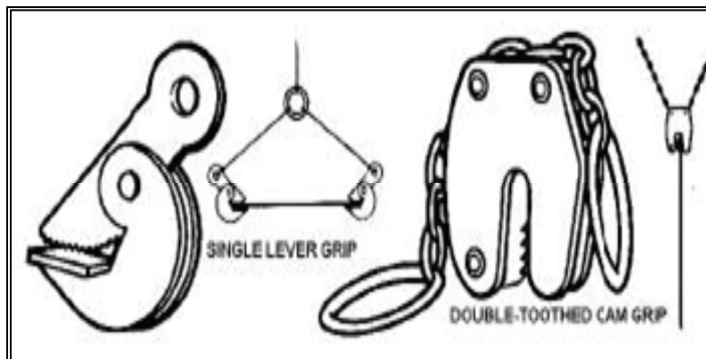
Figure 4-19. Plate-Handling Clamp Grips
