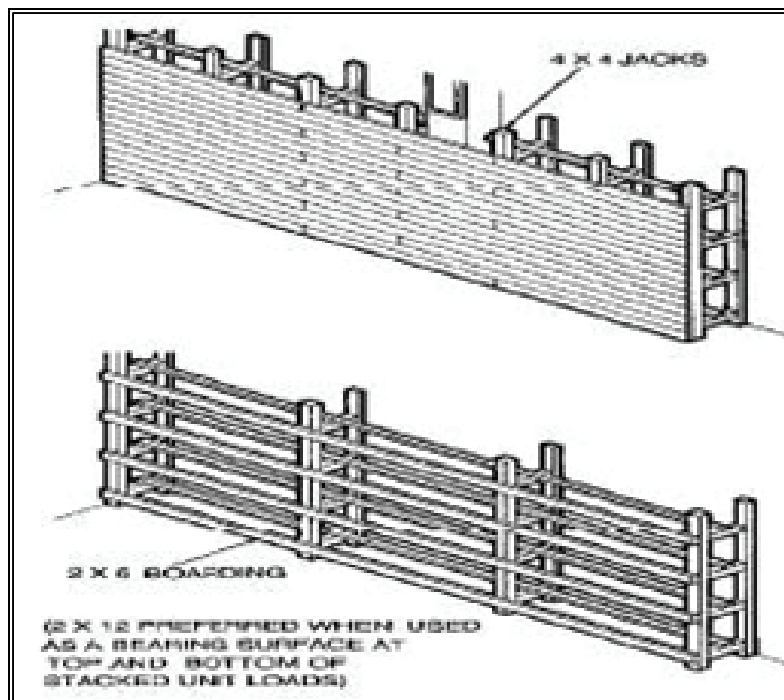
Figure 9-4. Heat and Nonheat Bulkheads
