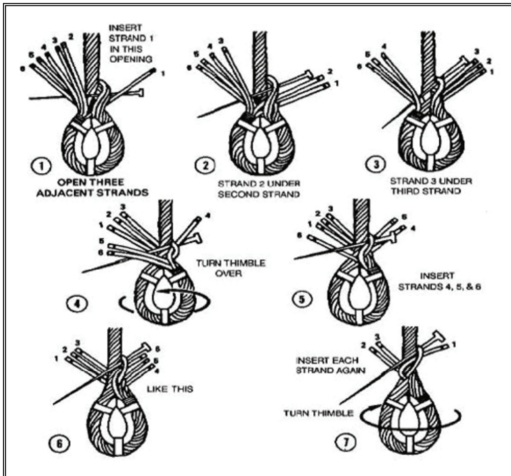
Figure 6-27. Tucking Strands of a Liverpool Splice
