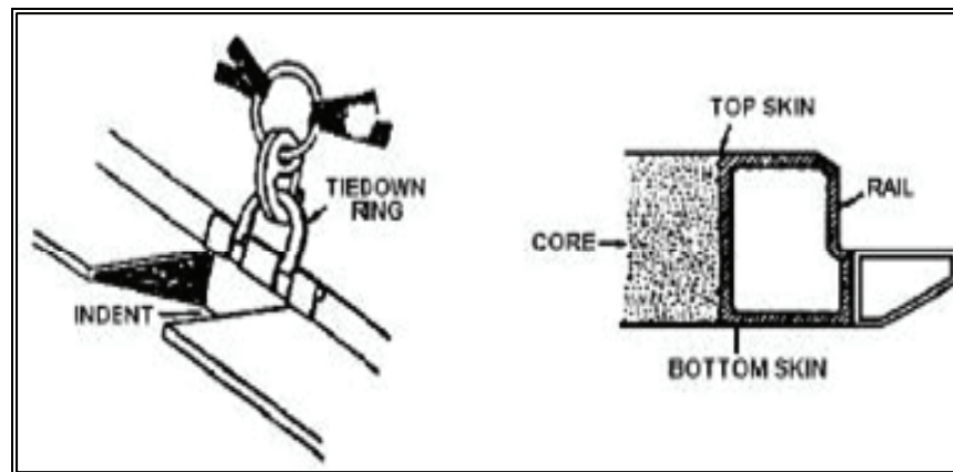
Figure 18-1. View of Rails and Indent on 463L Pallet
