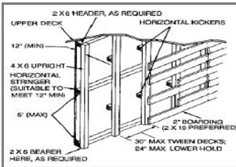
Figure 9-24. Heat Bulkhead, Smooth Side
