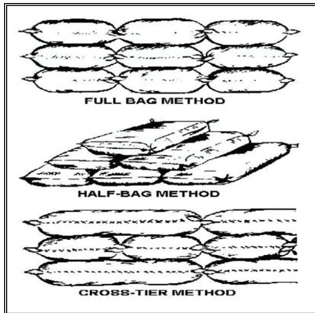
Figure 8-4. Methods for Stowing Bagged Cargo
