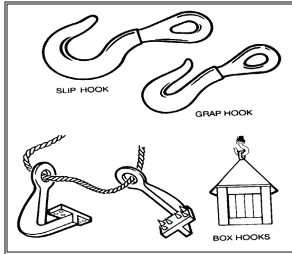
Figure 3-2. Sling Hooks
