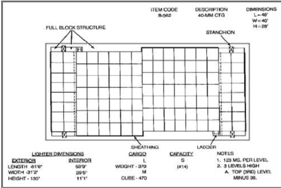
Figure 10-2. Lighter Prestowage Plan
