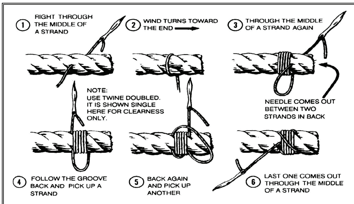
Figure 6-13. Making a Permanent Whipping
