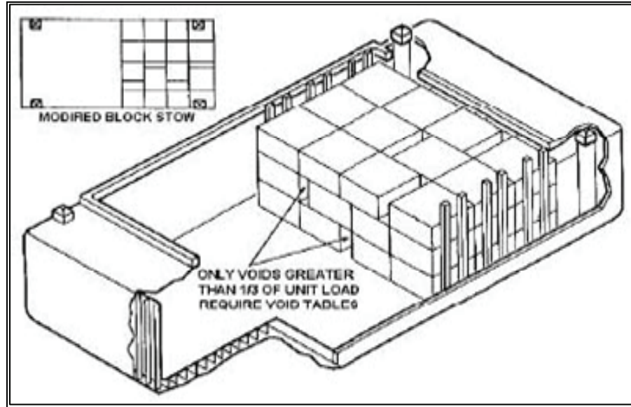
Figure 10-6. Modified Block Stow
