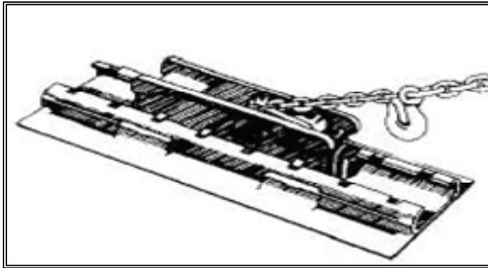
Figure 20-22. Saddleback Winch
