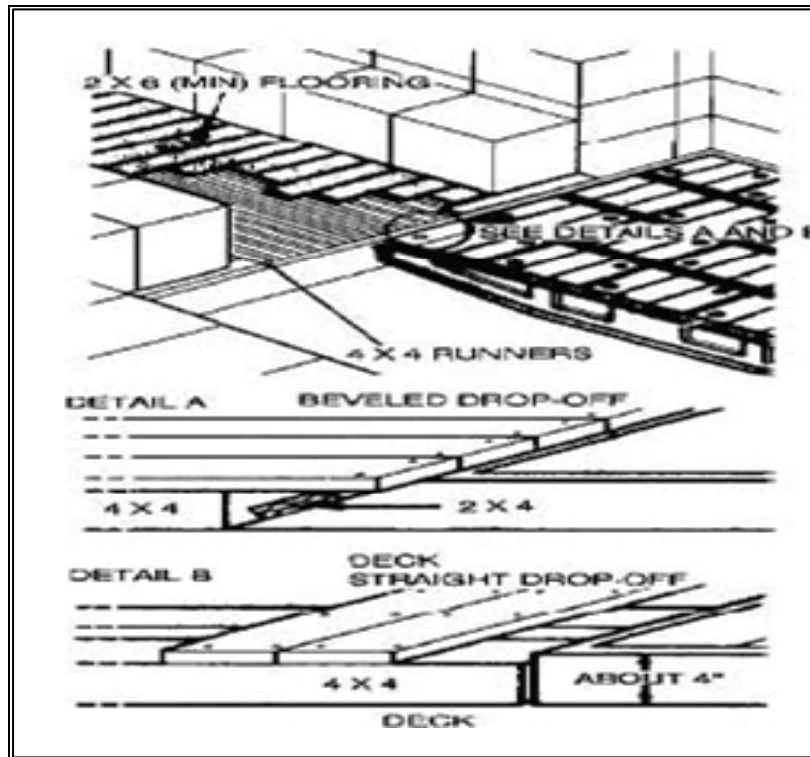
Figure 9-20. Examples of Elevated Flooring
