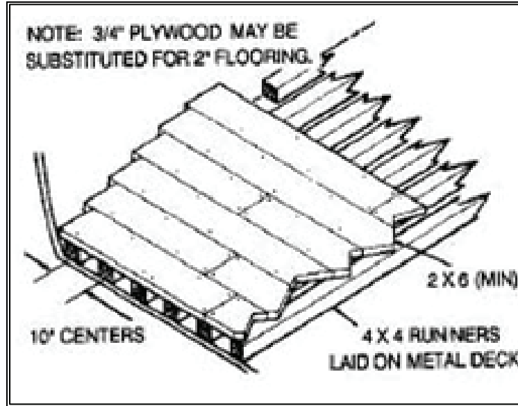
Figure 9-17. 2-Inch Wood Decking on 4 x 4 Runners
