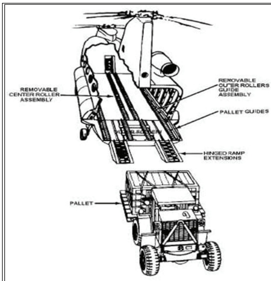
Figure 18-13. HICHS Installed in a CH-47 Helicopter
