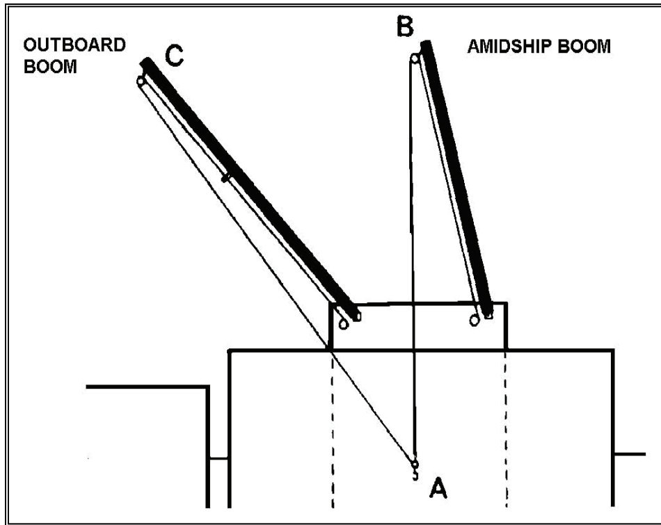
Figure 3-17. Determining if Outboard Boom Can Top Completely
