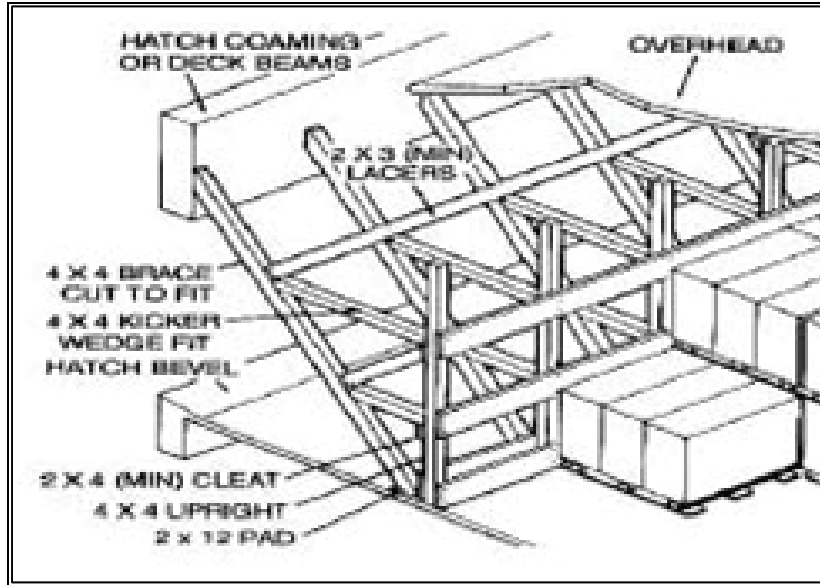
Figure 9-29. Nonheat Bulkhead using A-Frame
