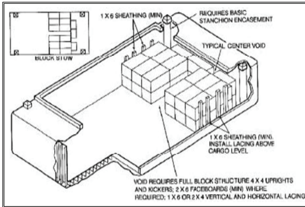
Figure 10-4. Block Stow
