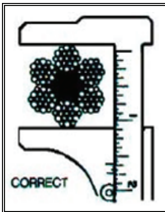
Figure 6-8. Measuring Wire Rope
