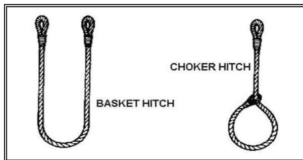
Figure 4-3. Ways of Using Single Slings
