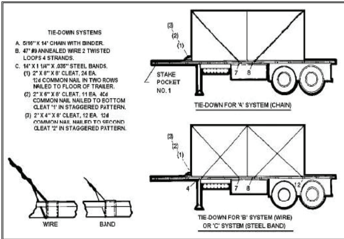
Figure 19-4. Recommended Tie-Down for Two CONEXs on M127 Semitrailer
