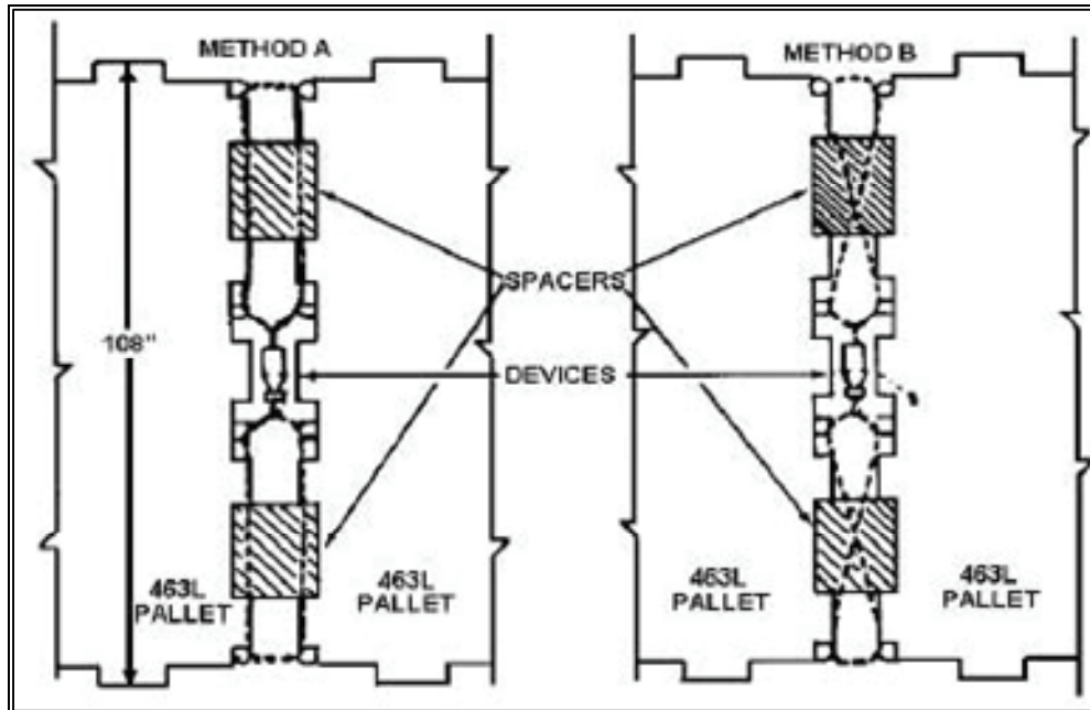
Figure 18-10. Methods of Marrying Pallets
