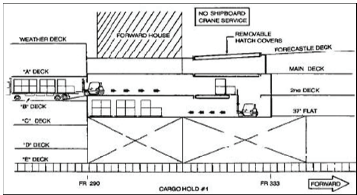
Figure 8-29. Alternate Loading Method for 37-Foot Flat
