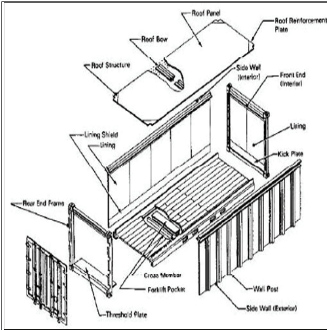
Figure 15-2. Exploded View of a Typical Aluminum Container
