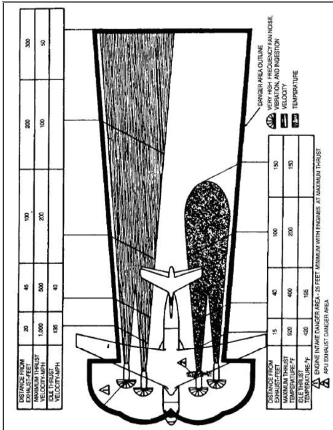
Figure 16-5. Danger Areas - Engines and APU
