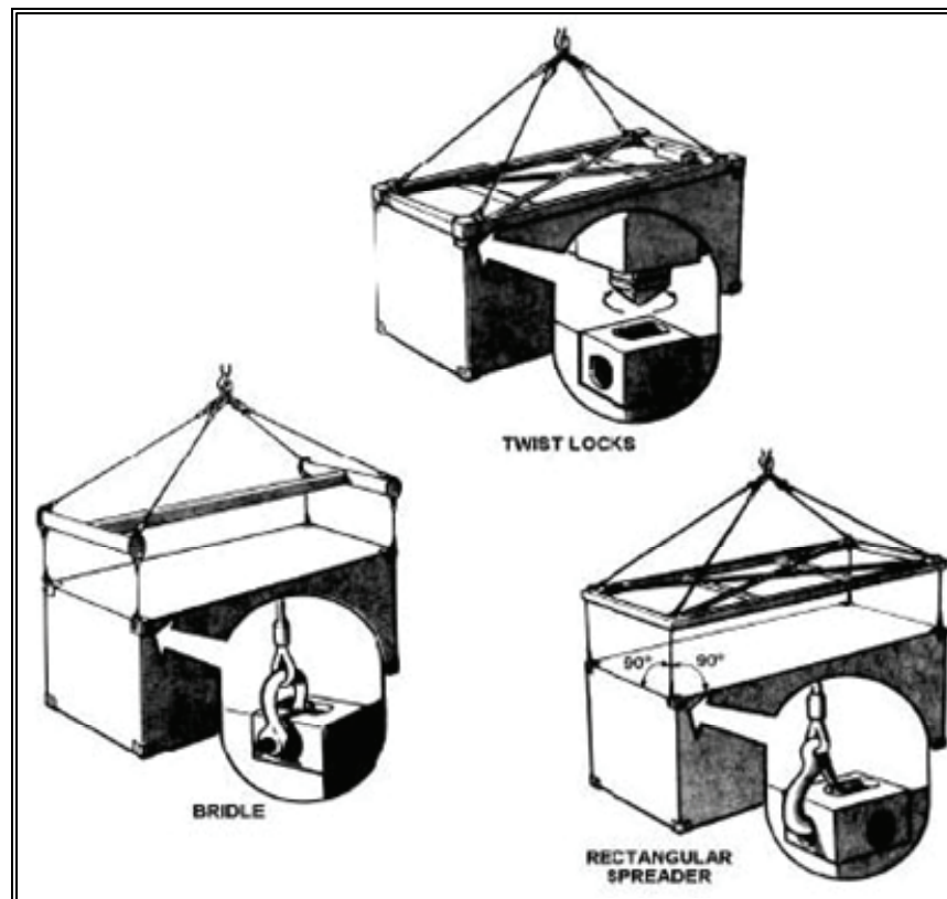
Figure 13-14. Top Corner Fittings for Lifting Containers
