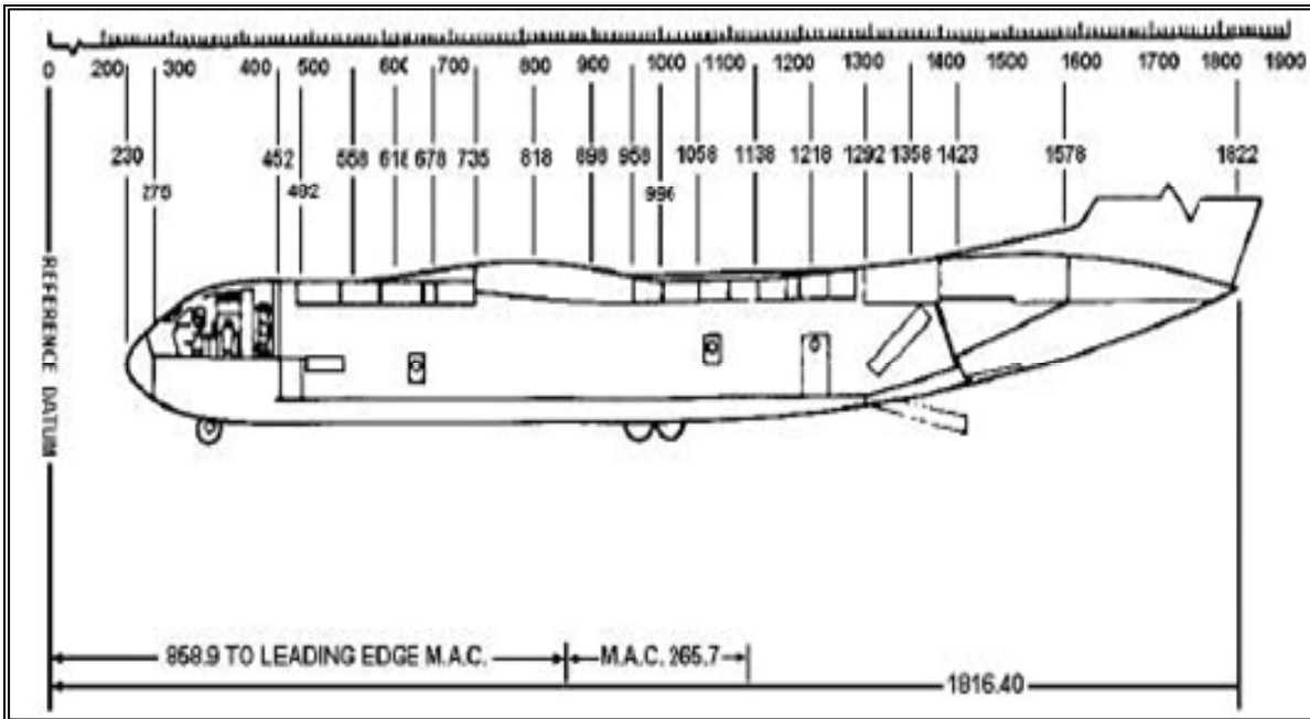
Figure 17-3. Airplane Station/Arm Measurements
