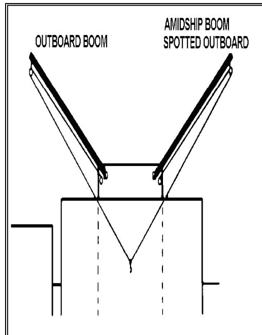
Figure 3-23. Spotting Booms with a West Coast Rig
