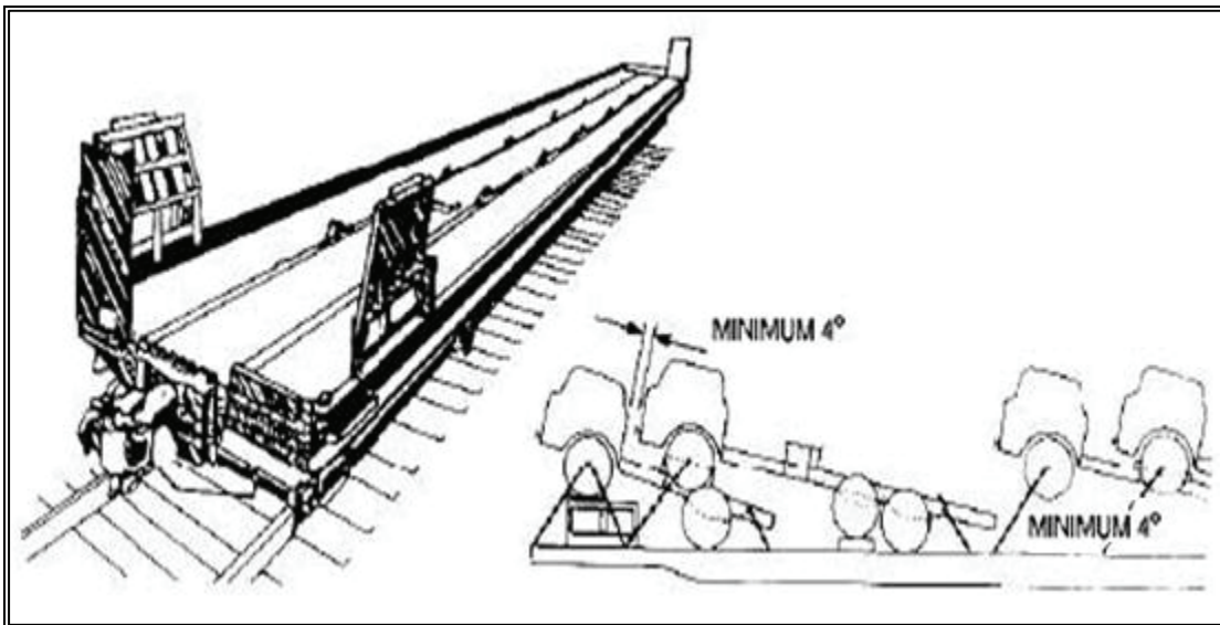
Figure 20-23. Flatcar, 89-Foot ITTX (Saddleback Flatcar)
