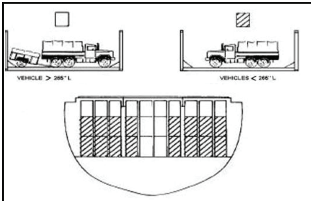
Figure 8-25. Required Cargo Mix for Hold 6 - Hatch Square Method
