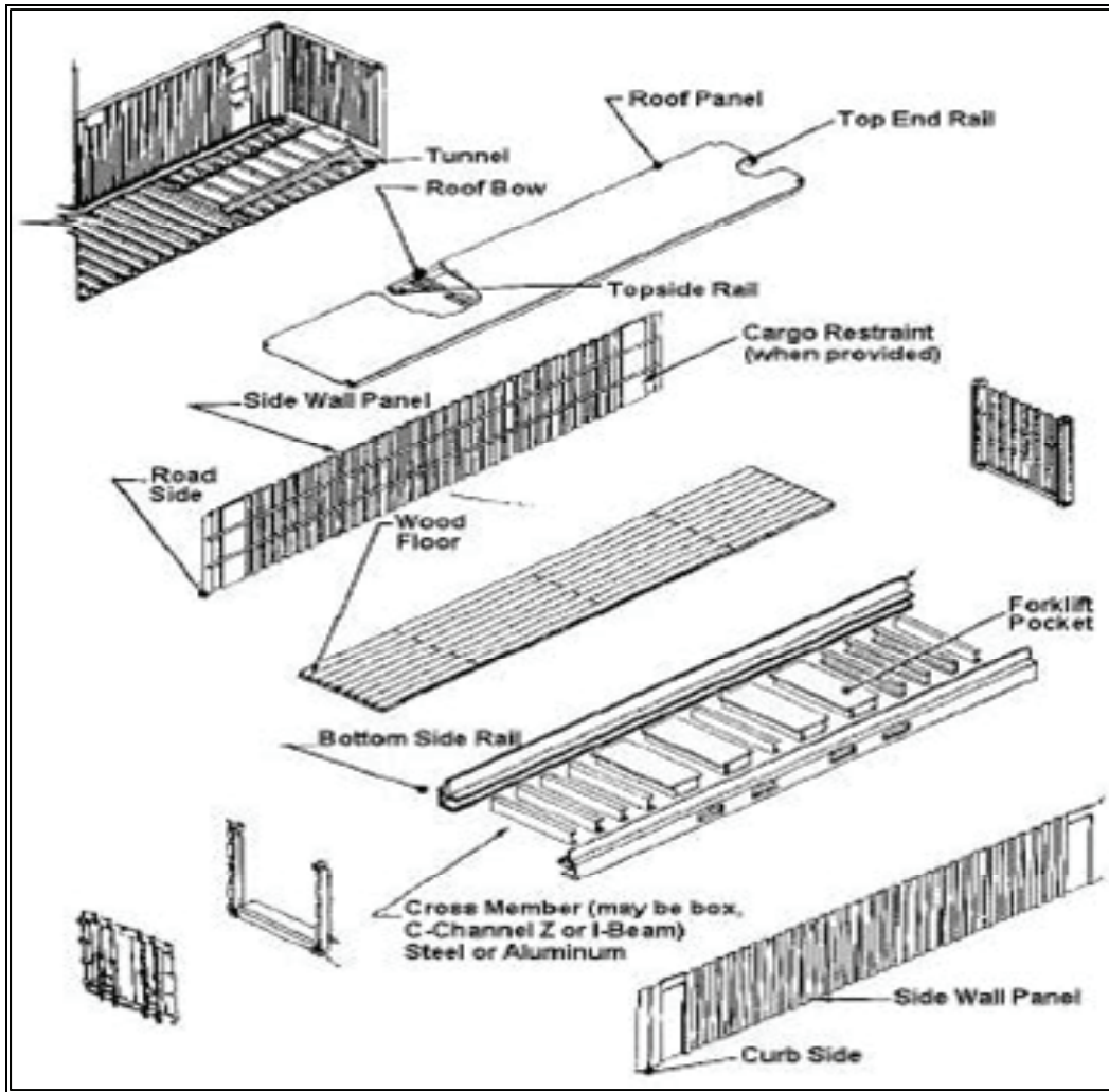
Figure 15-1. Exploded View of Typical Steel Container
