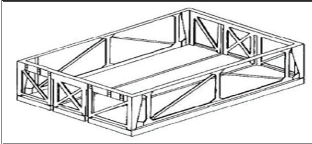
Figure 2-5. Conceptual Sketch of the Heavy-Duty Pontoon
