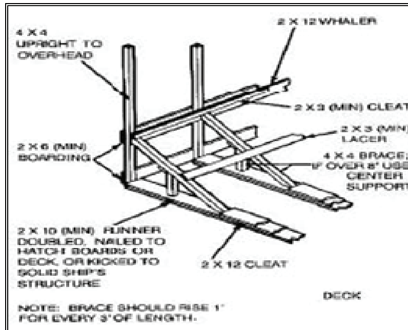
Figure 9-30. Nonheat Bulkhead using Deck Bracing
