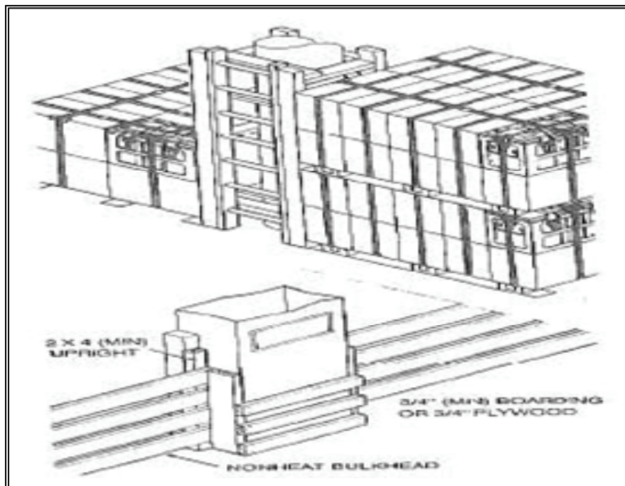
Figure 9-36. Partial Encasement with Rectangular Load
