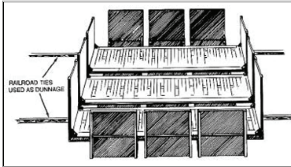
Figure 8-21. Flat rack Stacking Method
