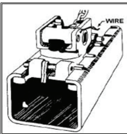
Figure 20-28. Anchor Seated and Ratchet Keeper Secured with Wire
