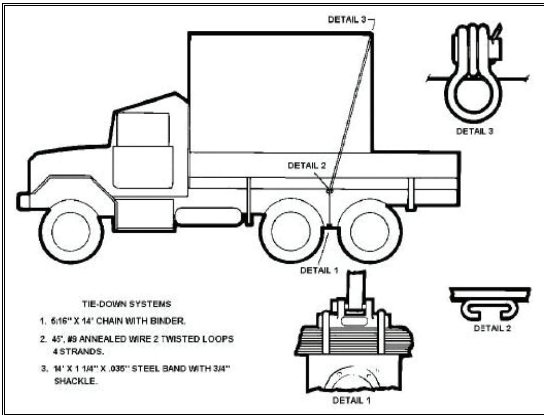
Figure 19-2. Recommended Tie-Down for CONEX on M35 Truck
