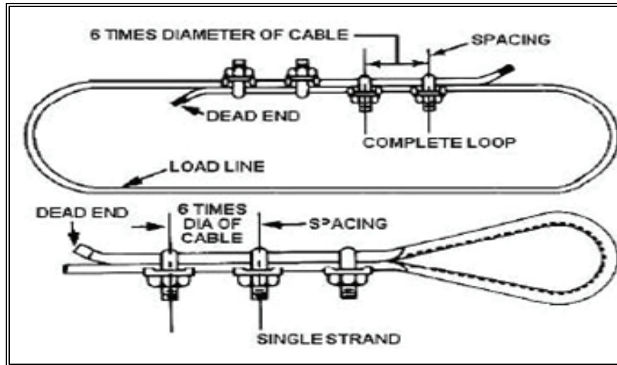
Figure 20-14. Cable Secured with Cable Clamps
