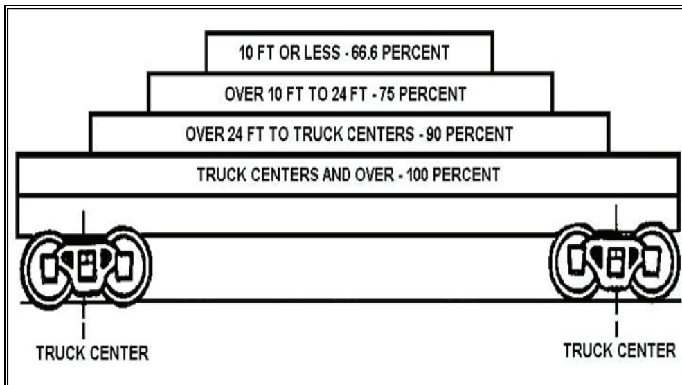
Figure 20-5. Standard Flatcar Load Limits
