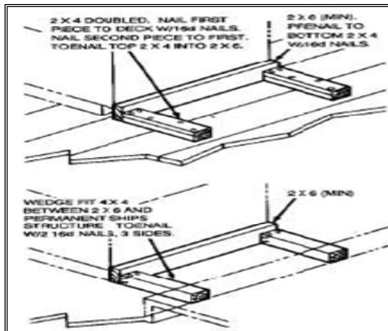
Figure 9-1. Blocking for Wood and Metal Decks
