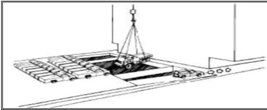
Figure 8-38. Simultaneous Lift-Off Operations for Hold 5 and Roll-Off Operations for MDA
