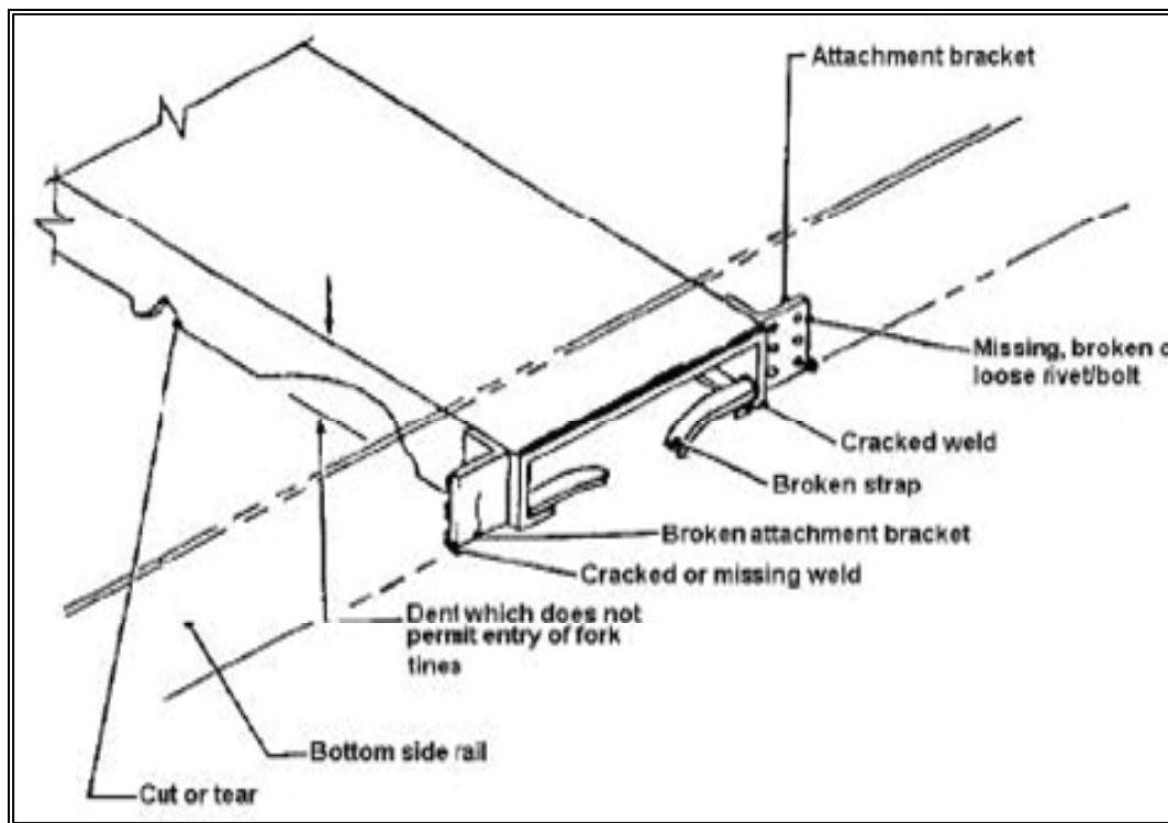
Figure 15-7. Examples of Forklift Pocket Damage
