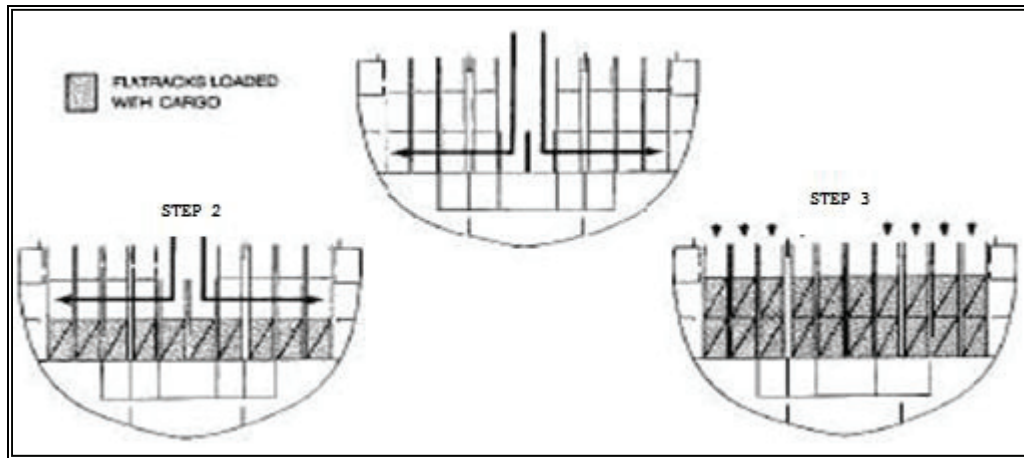
Figure 8-24. Hold 6 – Hatch Square Loading Method
