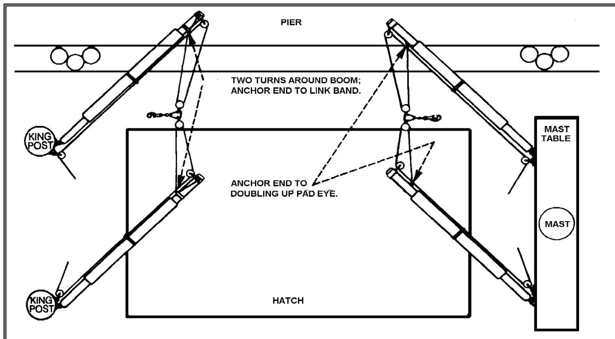
Figure 3-31. Yard-and-Stay Rig with a Double Purchase
