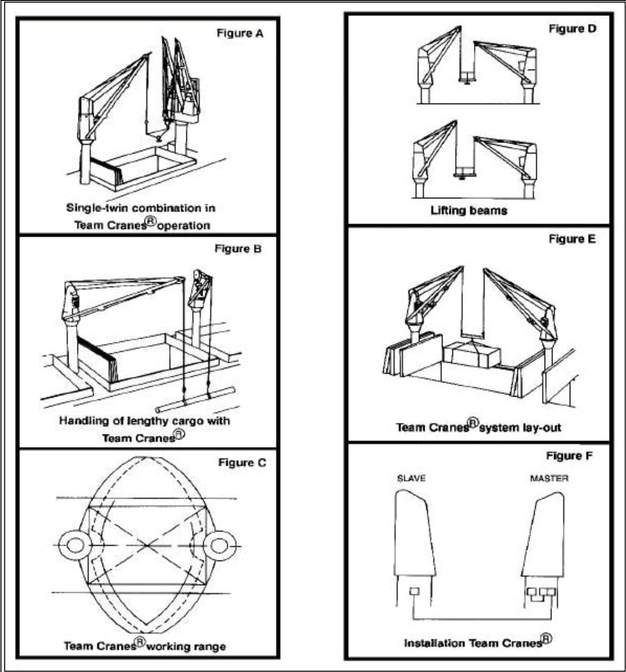
Figure 3-35. Various Crane Layouts for Operations
