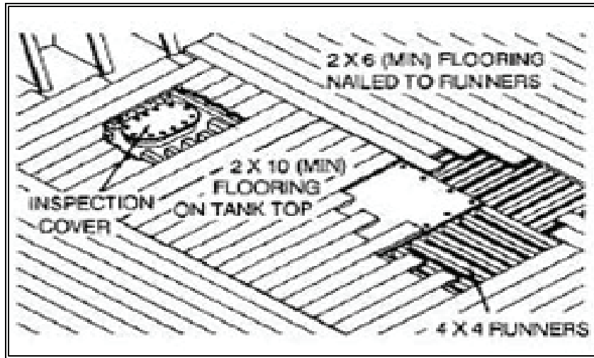
Figure 9-19. Flooring over Tank Top
