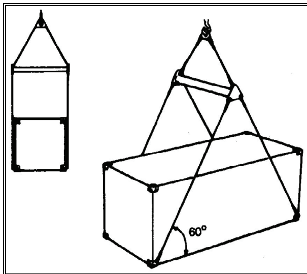
Figure 13-15. Bottom Lifting Techniques for Containers
