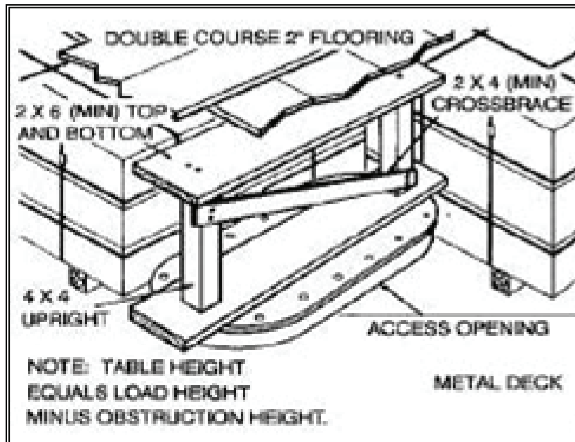
Figure 9-18. Void Table
