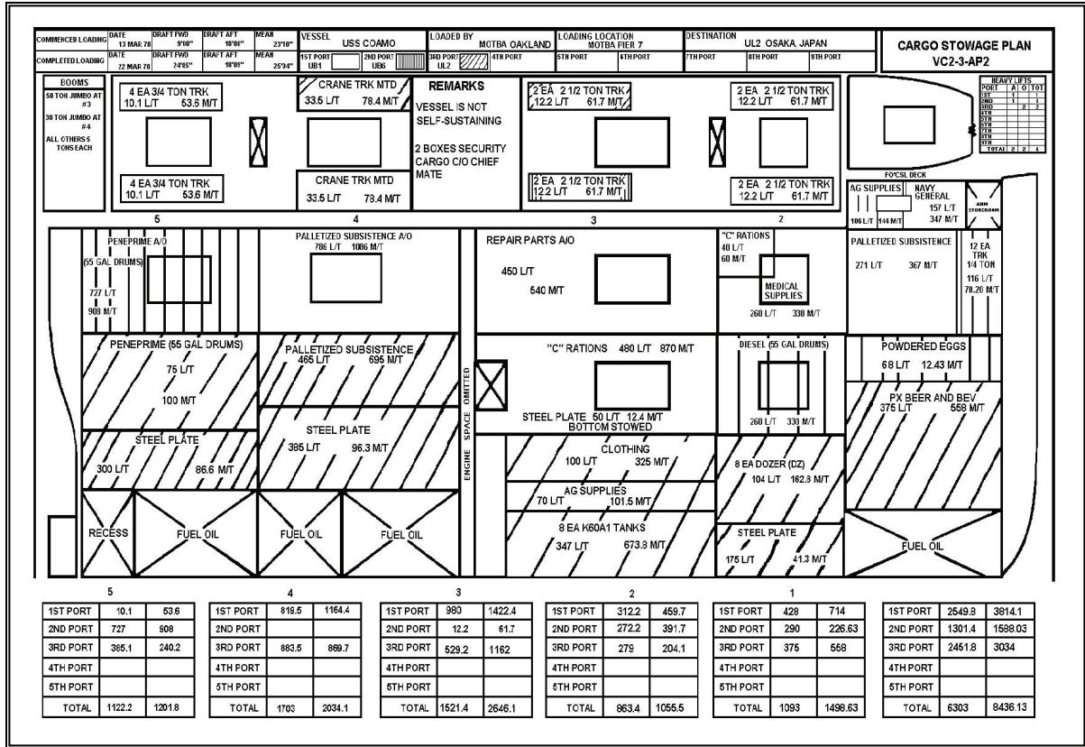
Figure 7-6. Cargo Stowage Plan
