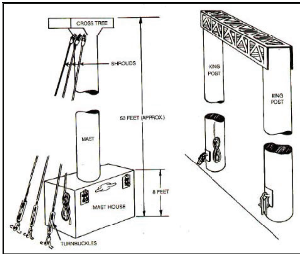
Figure 3-5. Standing Rigging
