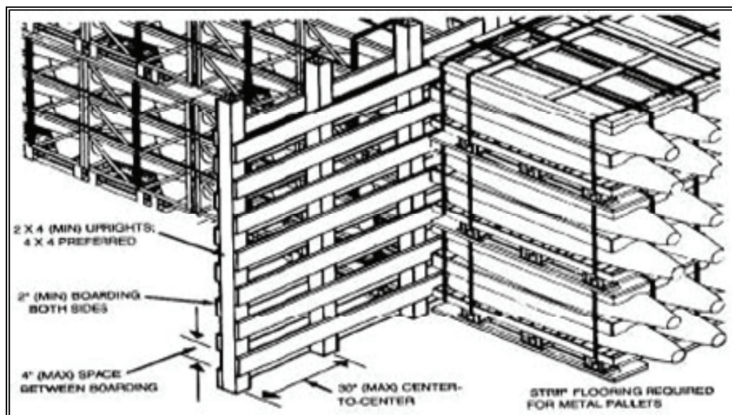
Figure 9-33. Partition Bulkhead
