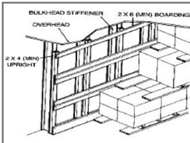
Figure 9-28. Nonheat Bulkhead, Stiffener Side
