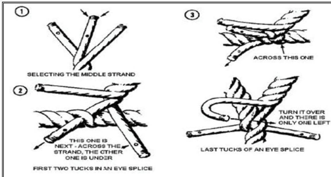
Figure 6-23. Making Eye Splices
