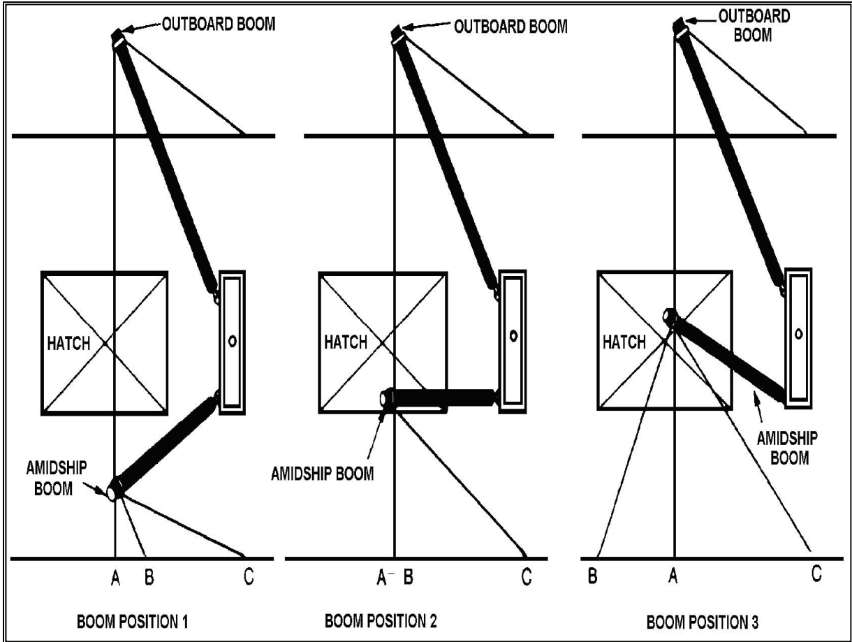
Figure 3-13. Guy and Boom Positions
