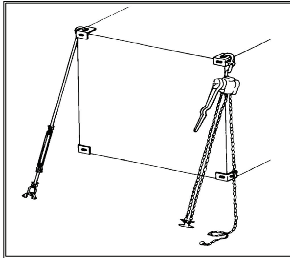
Figure 13-10. Two Types of Container Lashing Equipment
