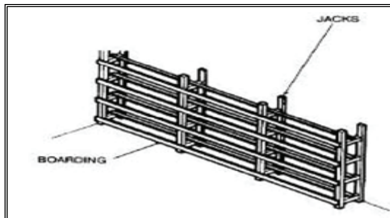
Figure 9-26. Typical Nonheat Bulkhead
