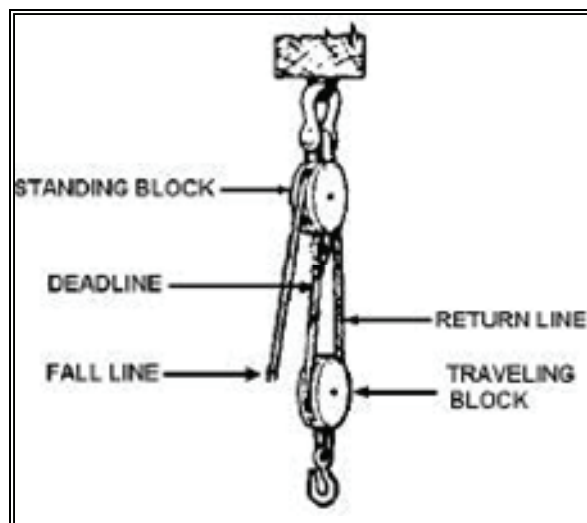
Figure 6-4. Double Block and a Tackle System
