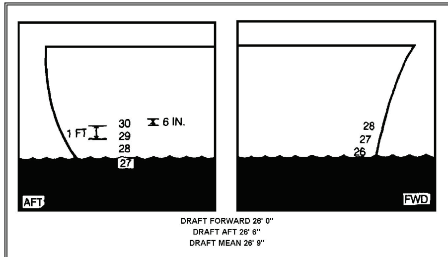
Figure 7-1. Draft Marks
