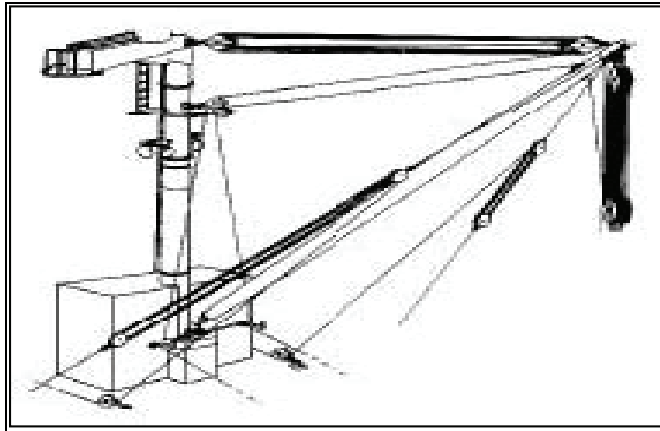
Figure 3-25. Typical Jumbo Boom
