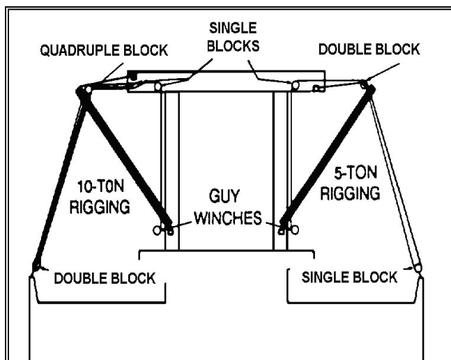
Figure 3-21. Ebel Rig
