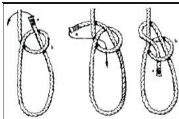
Figure 6-17. Bowline
