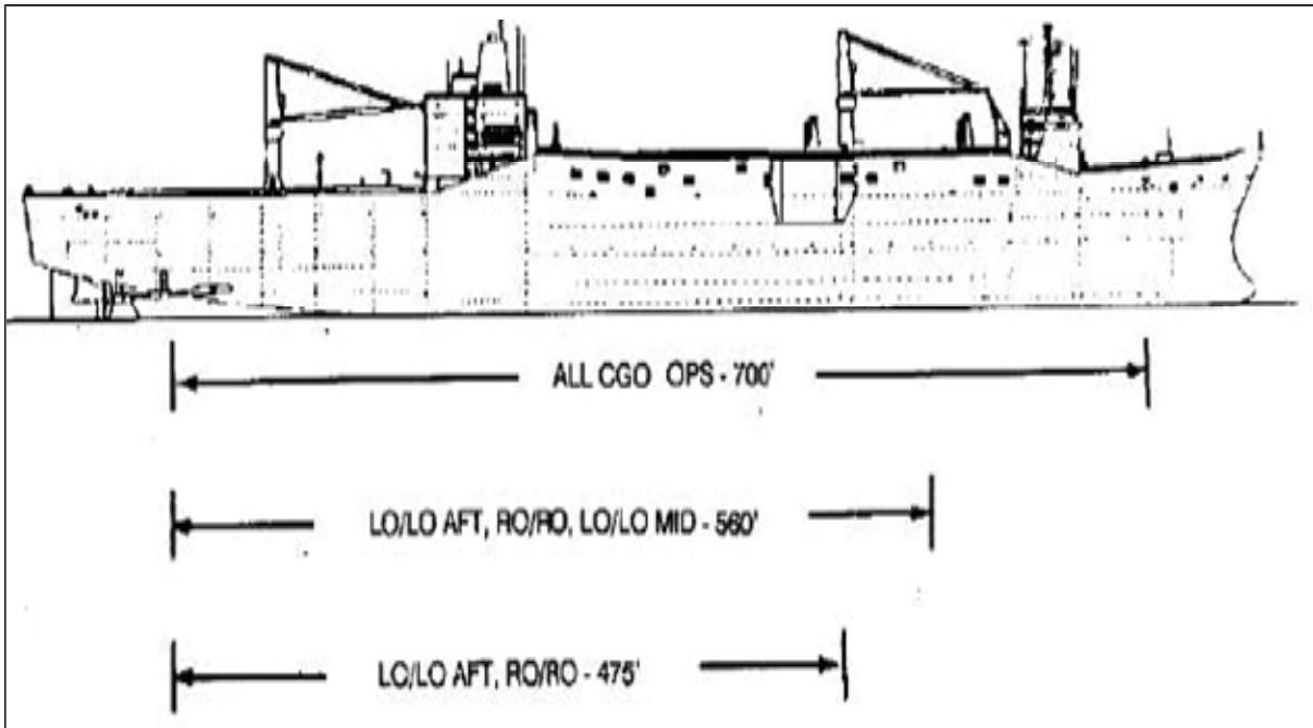
Figure 2-3. Fast Sealift Ship
