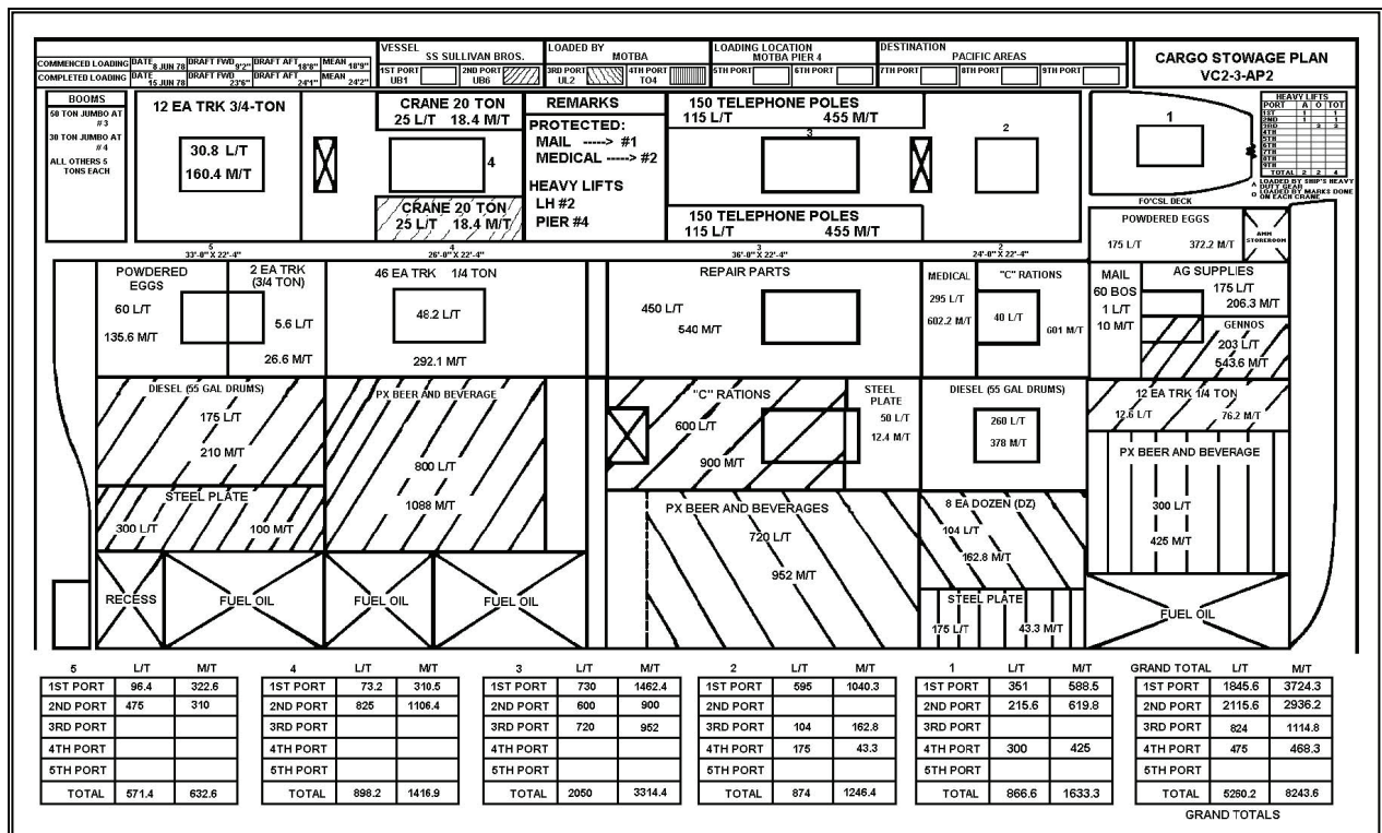
Figure 7-5. Cargo Prestowage Plan
