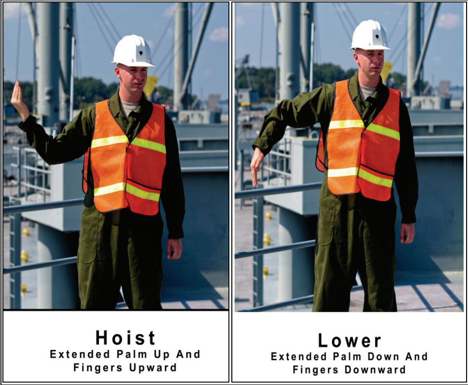
Figure 3-9. Signals Used in Winch Operations (One Winch)
