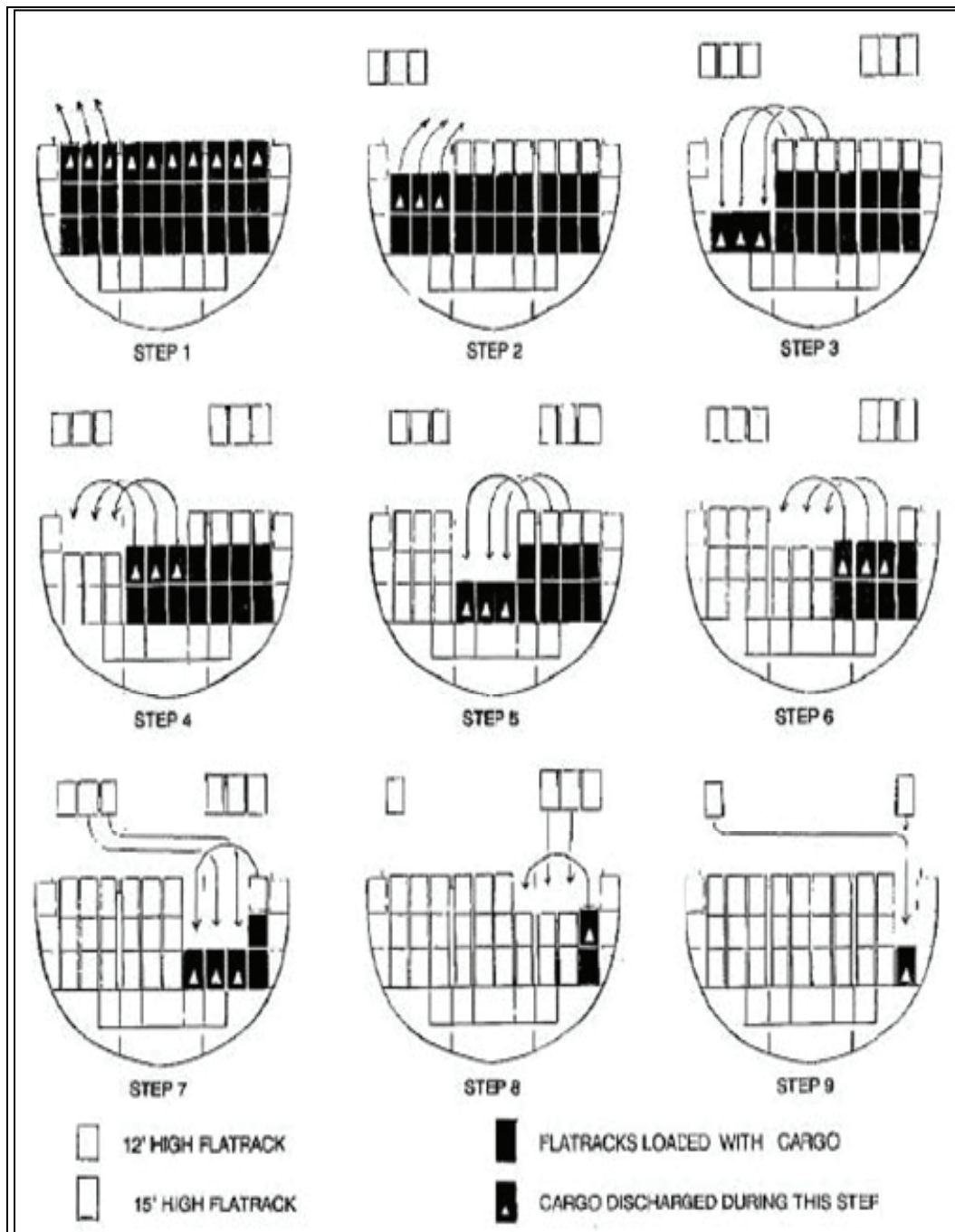
Figure 8-39. Hold 6 - Alternating Cells Discharge Method
