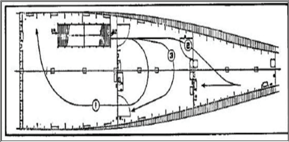
Figure 8-35. RO/RO Flow – "C" Deck
