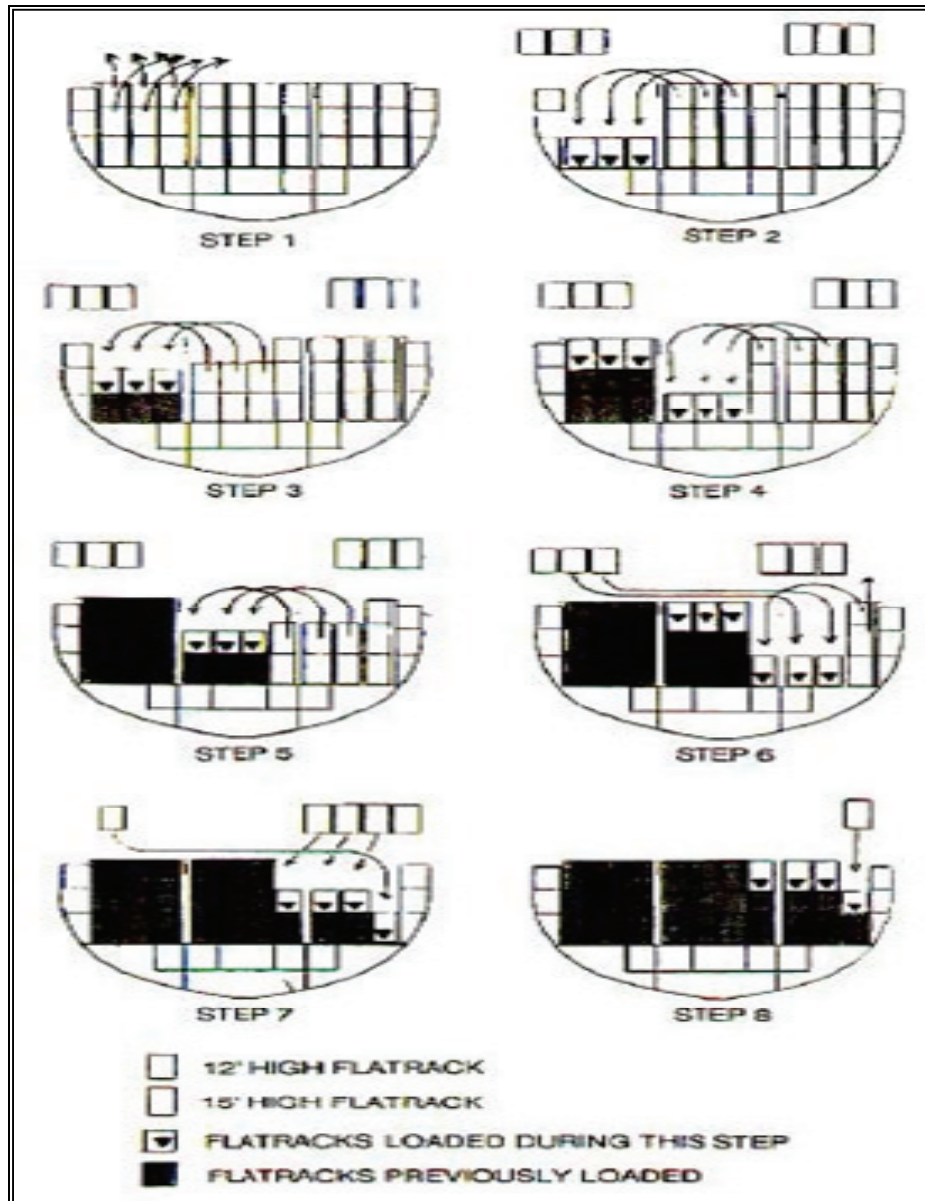
Figure 8-26. Hold 6 - Alternating Cells Loading Methods
