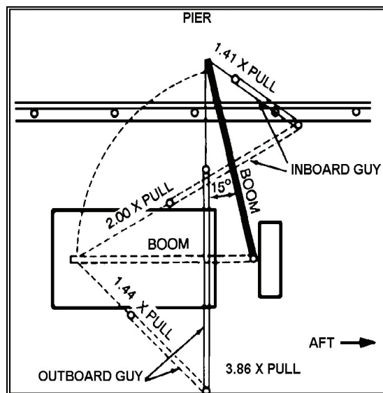
Figure 3-26. Proper Guying of Jumbo Boom
