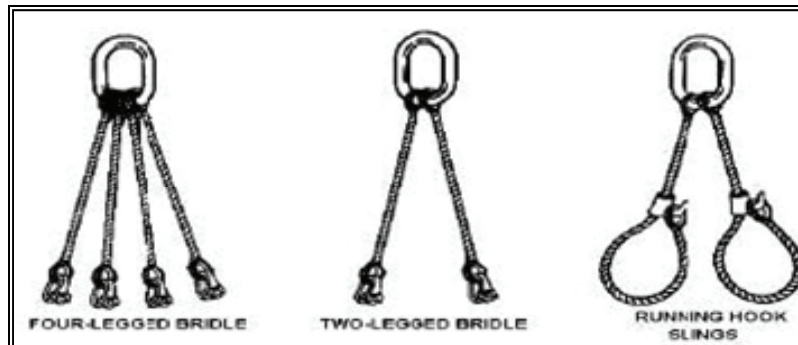
Figure 4-5. Combination Slings
