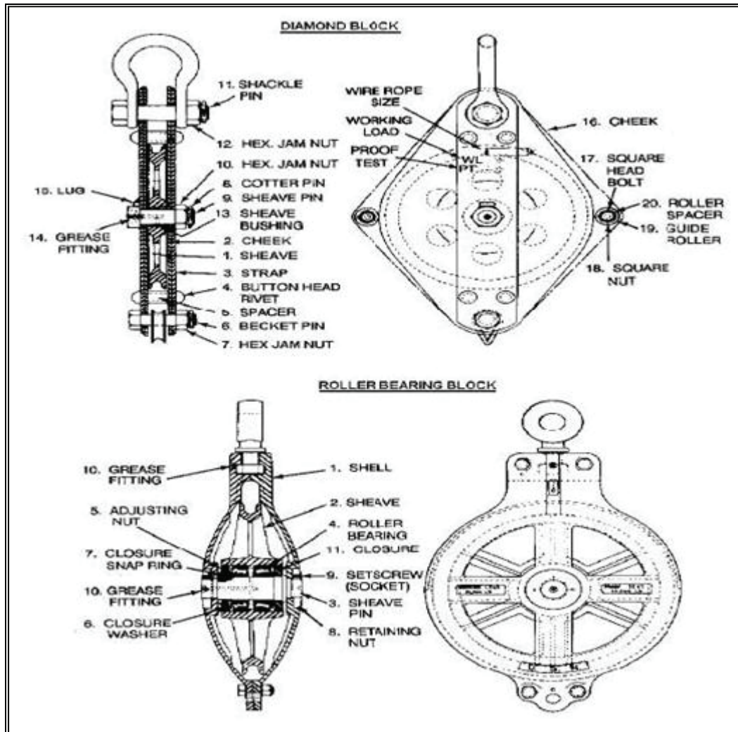
Figure 6-2. Components of Metal Blocks
