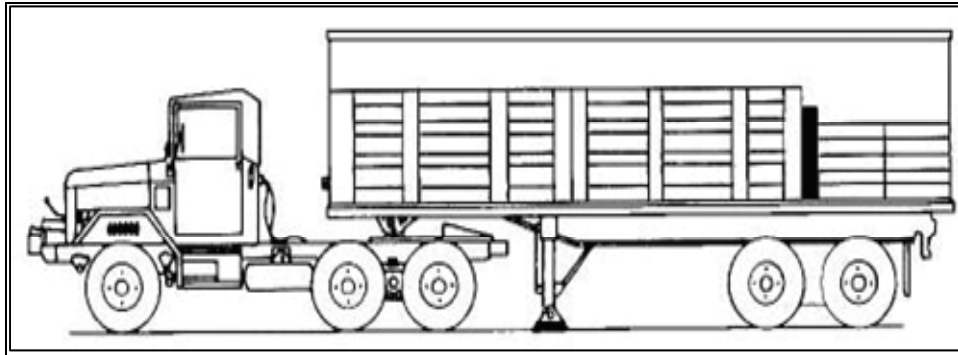
Figure 12-8. Dunnage Separating Mixed Commodities
