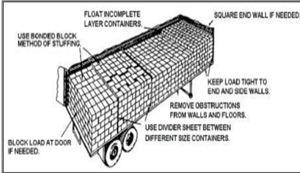
Figure 12-1. Bonded Block Method of Stuffing Cardboard Cartons
