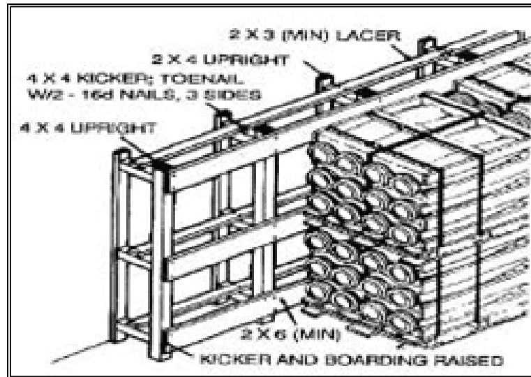
Figure 9-27. Nonheat Bulkhead using Jacks
