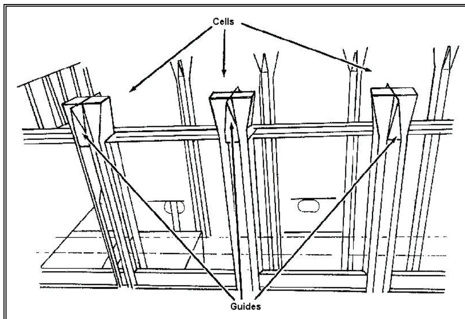
Figure 7-8. Location of Vertical Guides
