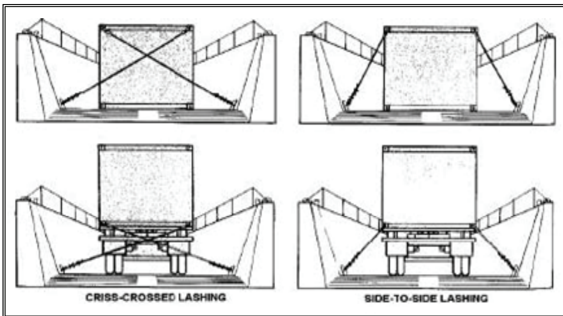
Figure 13-13. Container Lashing Methods
