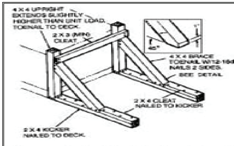
Figure 9-2. Basic Bracing for Wood Deck
