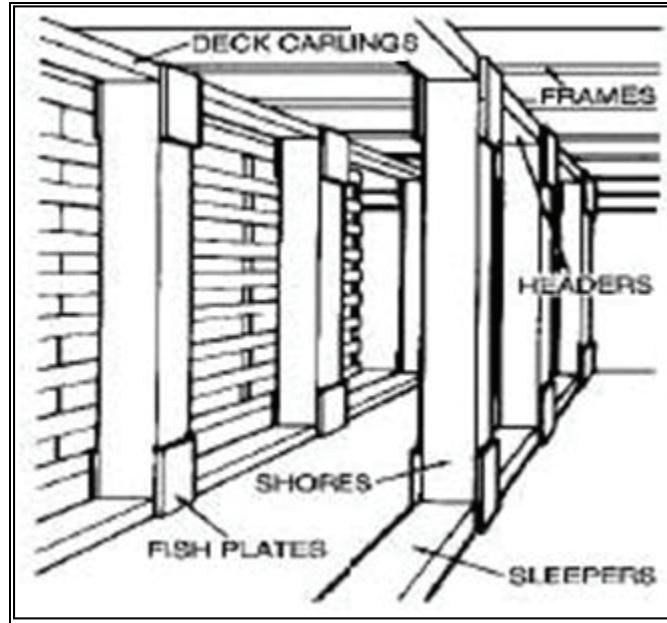
Figure 8-15. Applying Shoring Materials to a Ship's Hold
