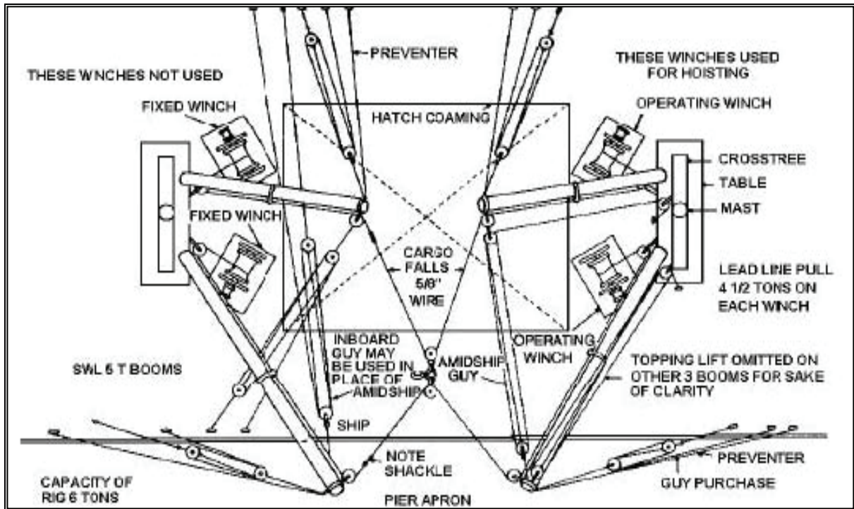
Figure 3-32. Block-in-Bight Method of Rigging Four Booms
