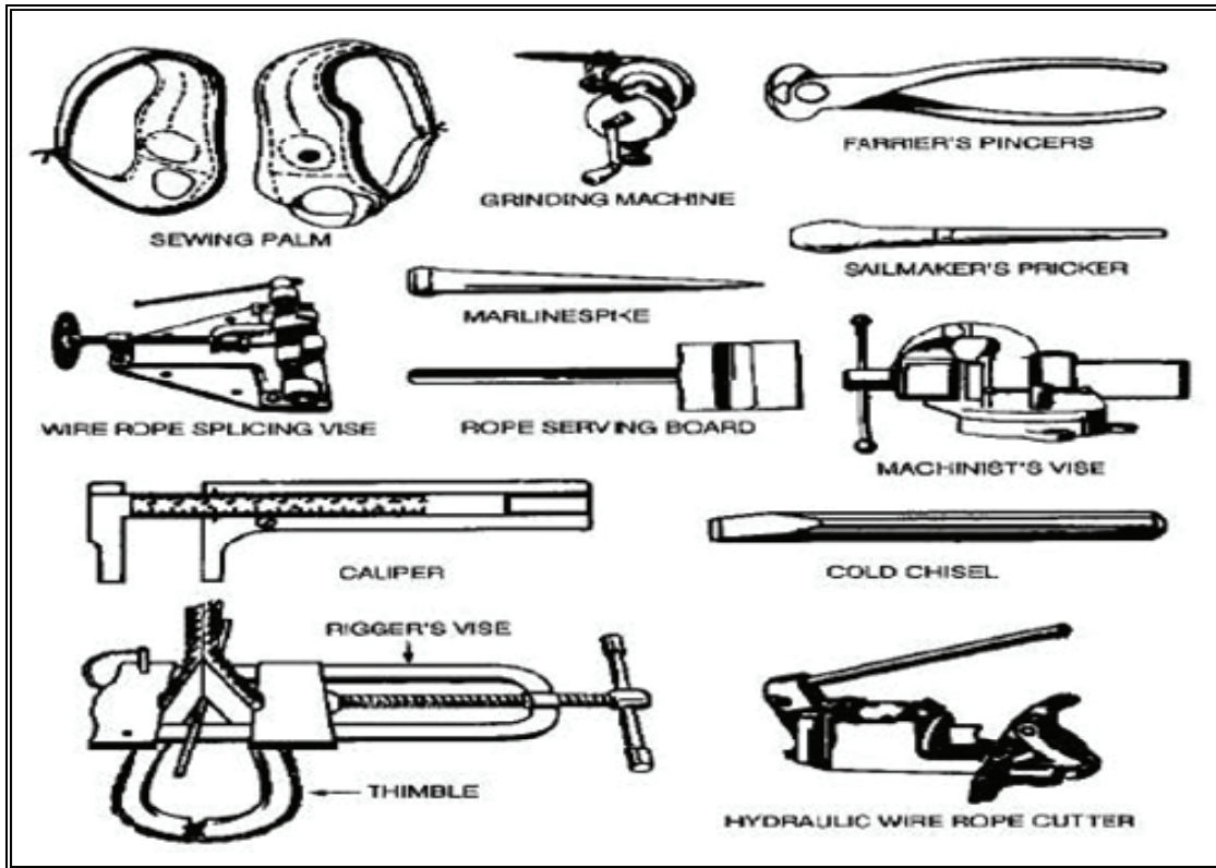
Figure 6-24. Selected Components of Rigger's Cargo Set
