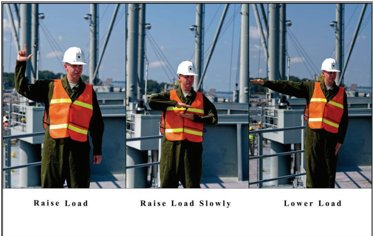
Figure 3-27. Jumbo Boom Signals
