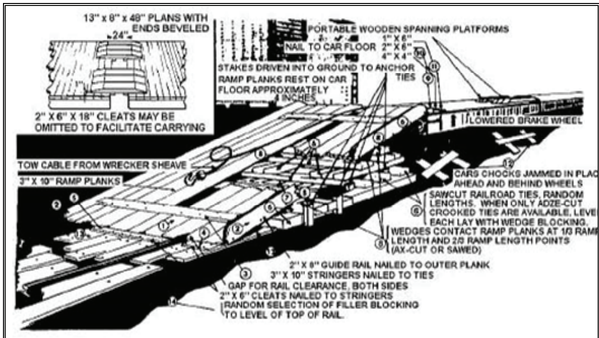
Figure 20-2. Improved End-Ramp for Loading
