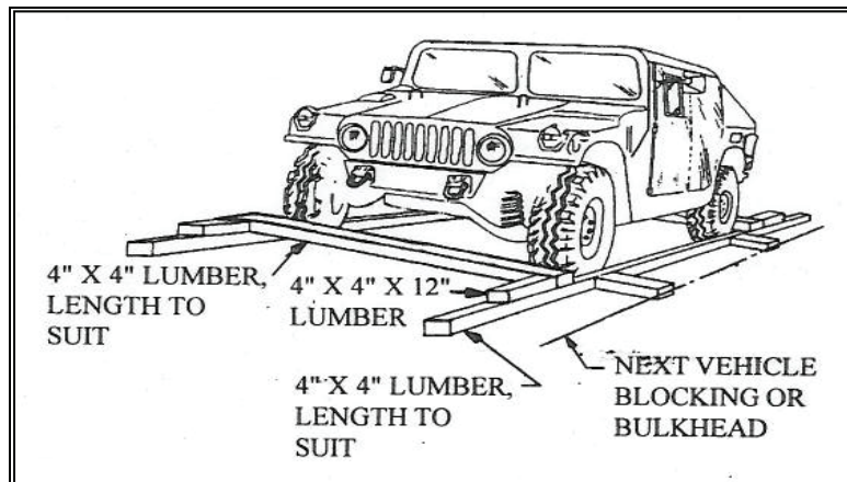
Figure 8-1. Vehicle Secured on Deck
