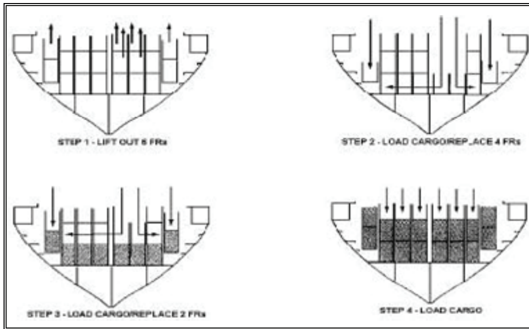
Figure 8-27. Holds 7A and 8F – Hatch Square Loading Method
