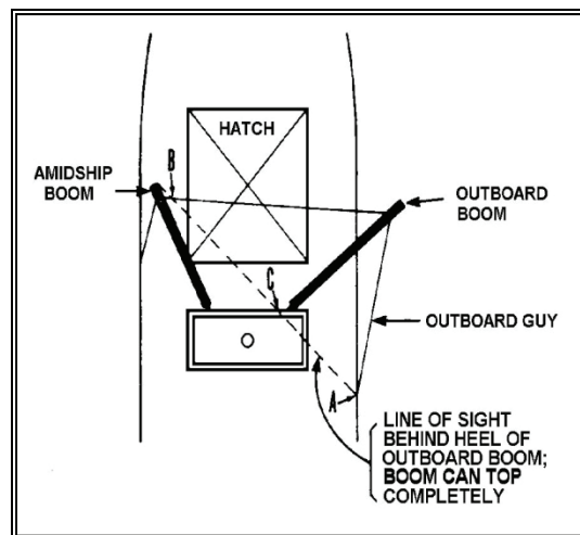
Figure 3-19. Spotting Booms with Yard-and-Stay Rig
