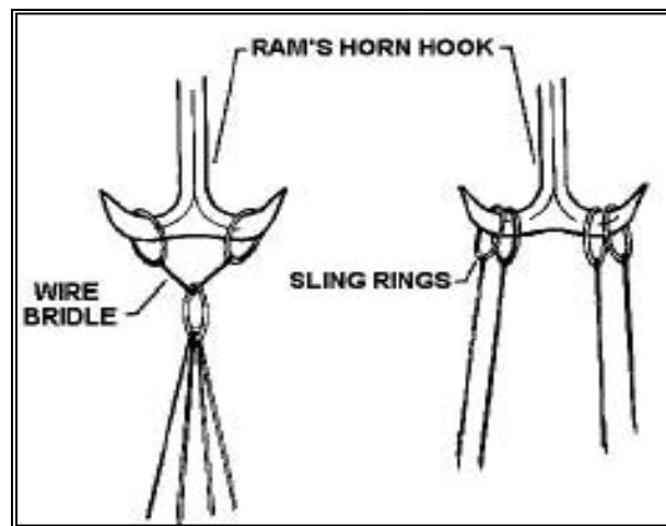
Figure 3-37. Two Methods of Attaching Slings to Ram's Horn
